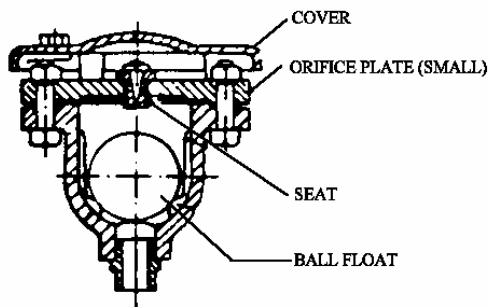
SINGLE VALVE
