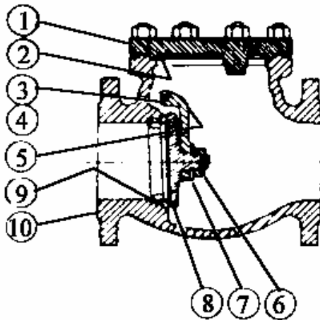
SWING
