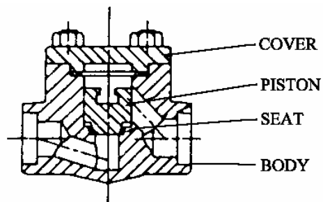
LIFT (PISTON)
