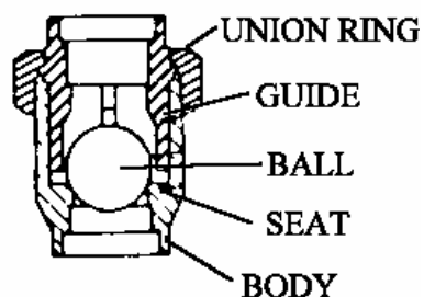
LIFT (BALL-VERTICAL)
