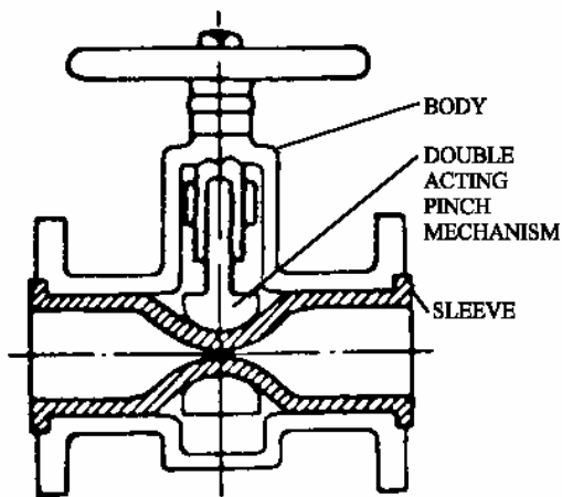
PINCH
