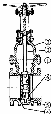
DOUBLE DISK GATE
