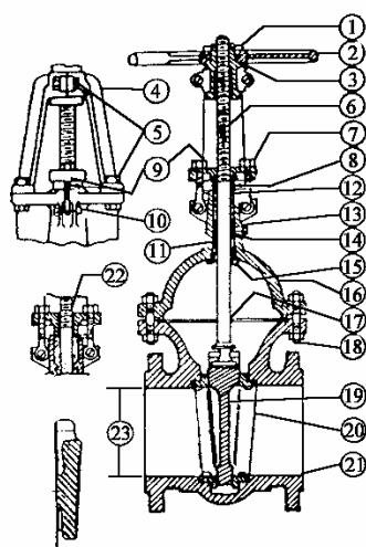
WEDGE GATE
