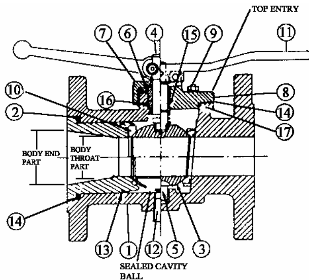
ONE PIECE BODY (END OR TOP ENTRY)
