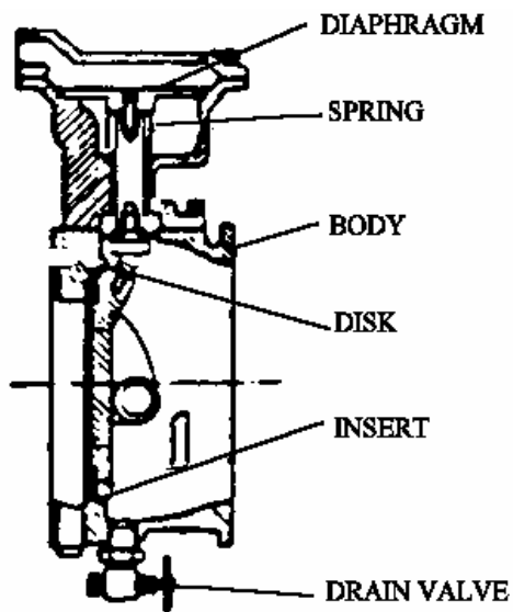
DELUGE VALVE
