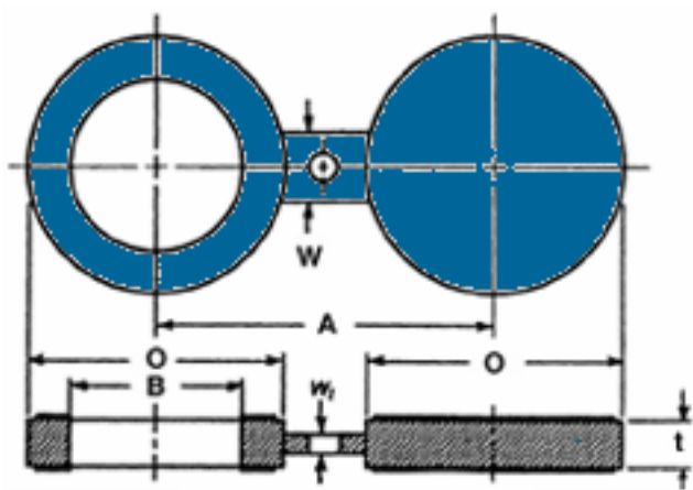
Figure 30: Spectacle blind
