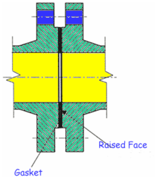
Figure 13: Raised face
