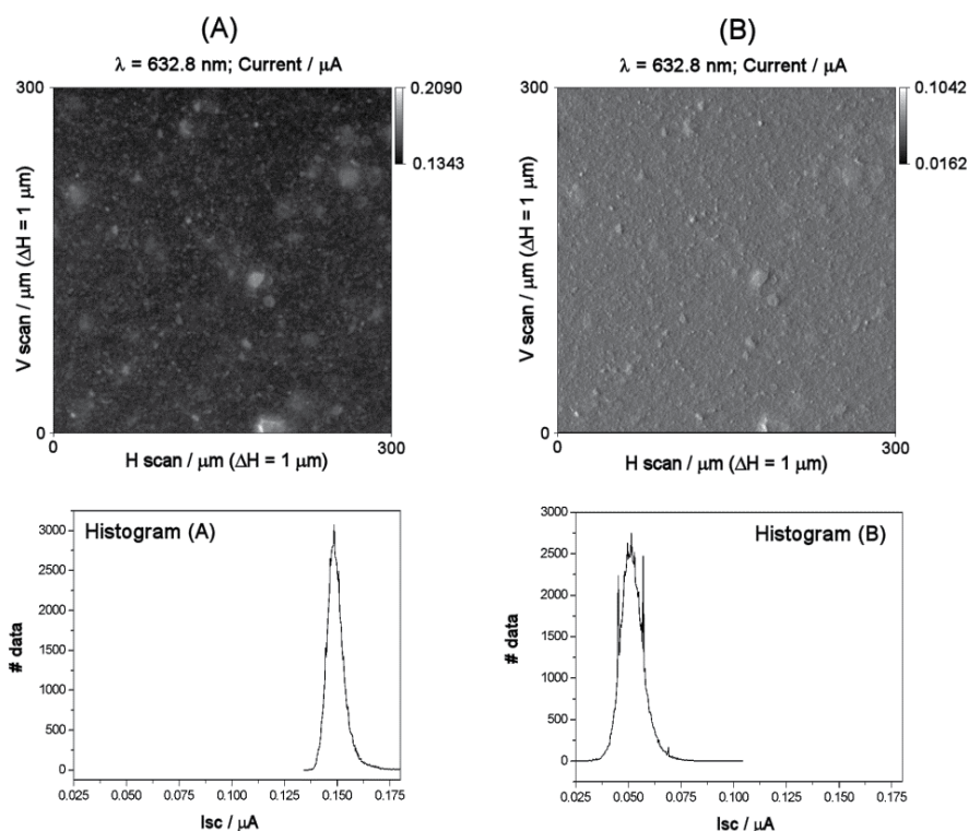
Fig. 14. (A) LBIC image for the DSSC using red laser. (B) The same image modified using our algorithm.
