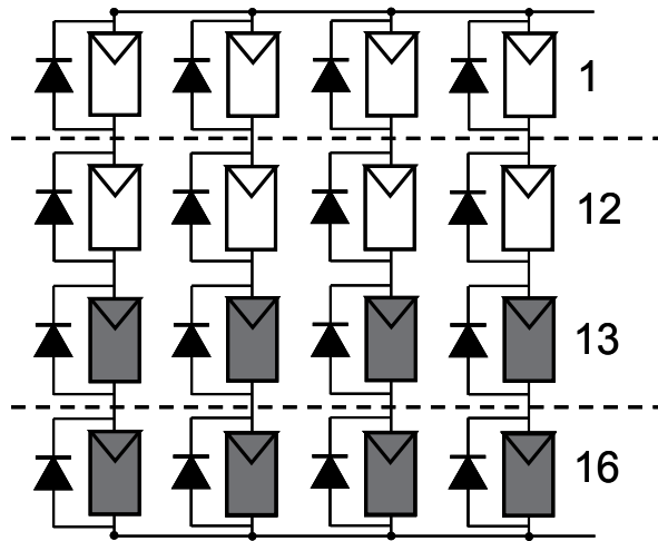
Fig. 9. Array ( N_S = 16, N_P = 4 ) with shading patterns - Configuration 1
