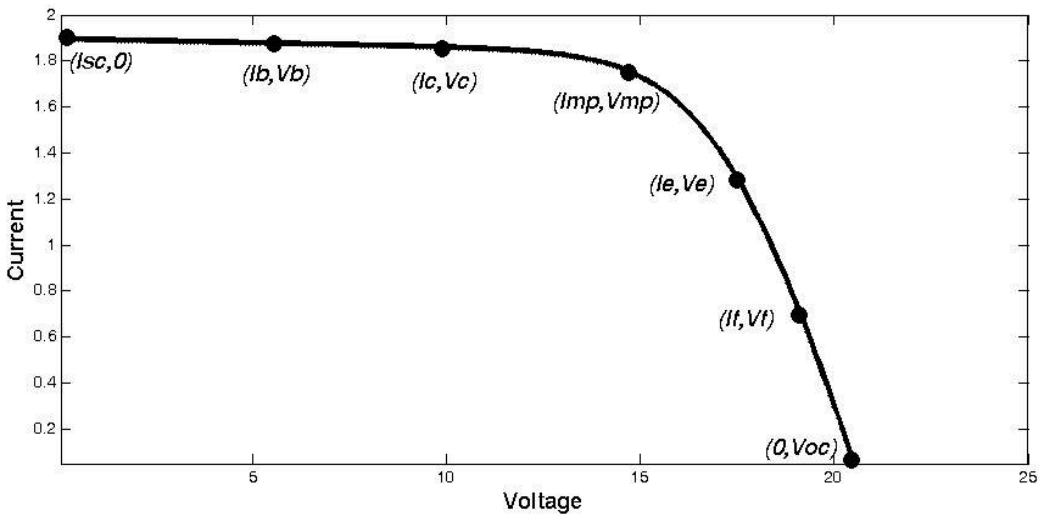
Fig. 3. Seven points on the I-V curve of a solar panel to solve the nonlinear equations.
