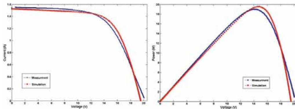
Fig. 12. A typical extracted solar panel's I-V curve
