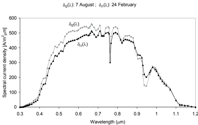
Fig. 2. Comparison of spectral current density in winter and summer.
