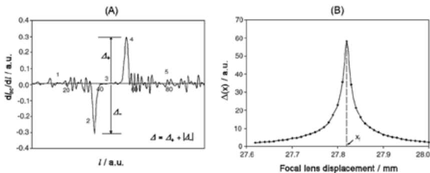
Fig. 3. (A) Numerical derivative of the I_{SC} -curve shown in Figure 2A. (B) Representation of the \Delta value versus positions of the focal lens.
