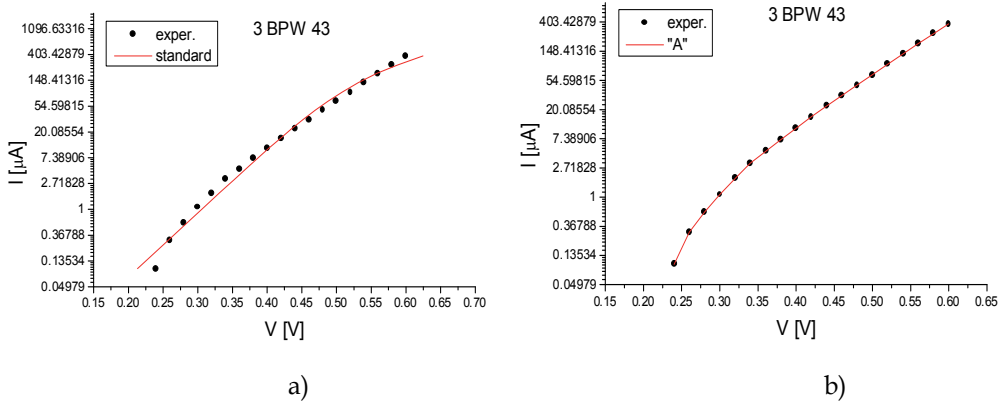
Fig. 3. Agreement: experimental and calculated data for a) standard, b) method "A" (Vasic et al., 2005).
