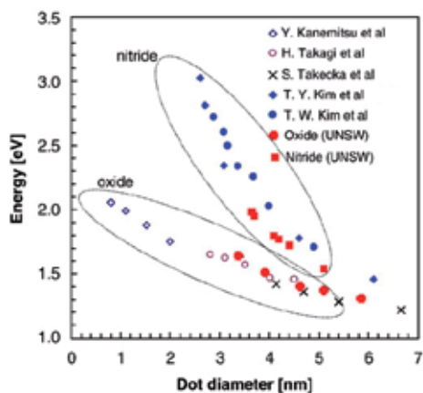
Fig. 12. Experimental energy gaps of three-dimensionally confined Si QDs in SiO 2 and SiN x matrices (300°C) for several research groups (Takeoka et al., 2000) (Kim et al., 2004), (Kim et al., 2005) (Yang et al., 2004) (Fangsuwannarak, 2007).
