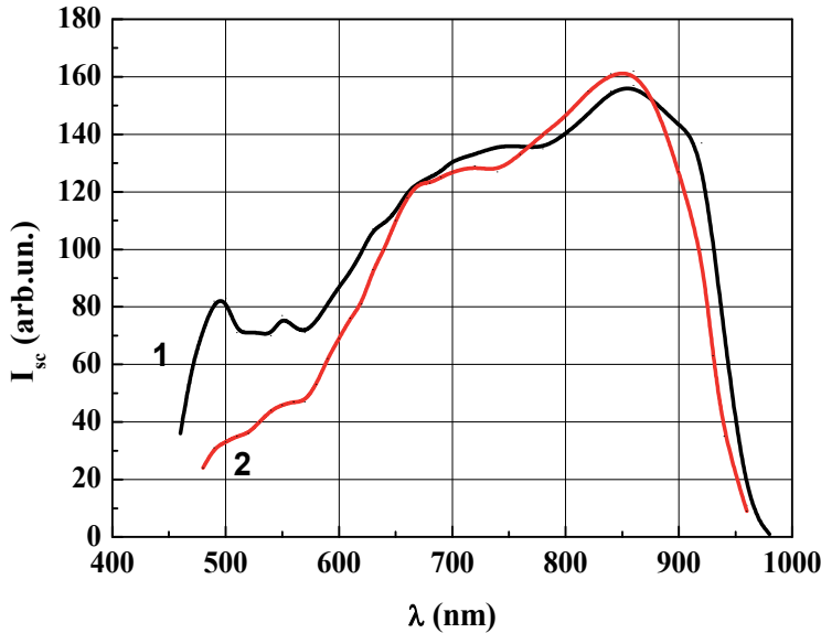
Fig. 13. The spectral photo sensitivity of Cu/n+ITO/pInP/Ag:Zn structure: 1- before H 2 annealing, 2- after H 2 annealing
