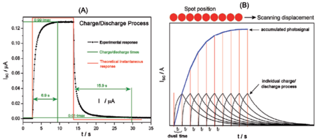
Fig. 6. (A) Representation of experimental data of the charge and discharge process of a cell irradiated with a power of 292 \mu W , and a comparison with a theoretical instantaneous response. (B) Simulation of the evolution of the irradiated spots showing how the photovoltaic response is influenced by the previously excited points.
