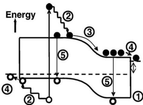
Fig. 1. Loss processes in a standard solar cell: (1) non-absorption of below band gap photons; (2) lattice thermalisation loss; (3) and (4) junction and contact voltage losses; (5) recombination loss (Green, 2003).
