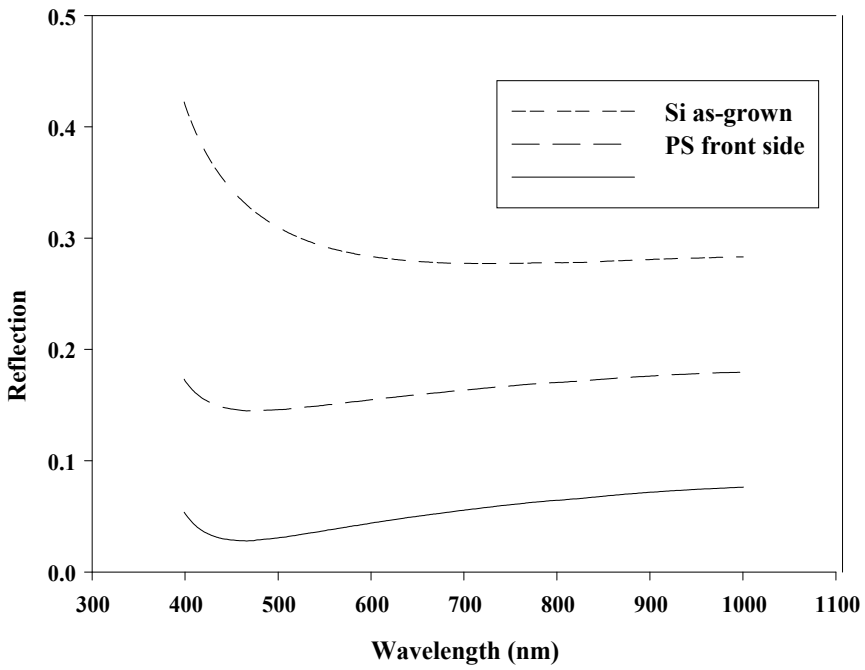
Fig. 11. The reflectance spectra of Si (as grown) and PS of both sides
