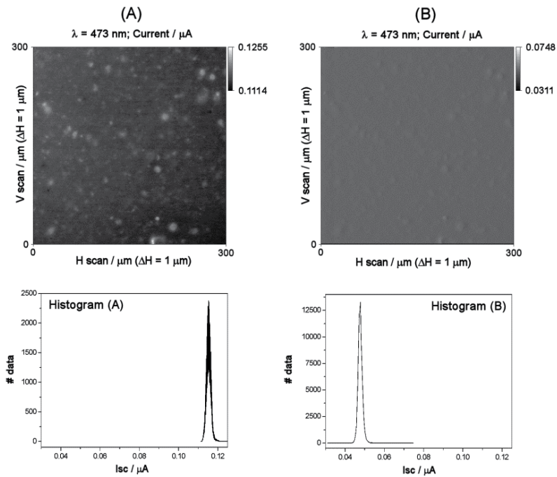
Fig. 16. (A) LBIC image for the DSSC using blue laser. (B) The same image modified using our algorithm.
