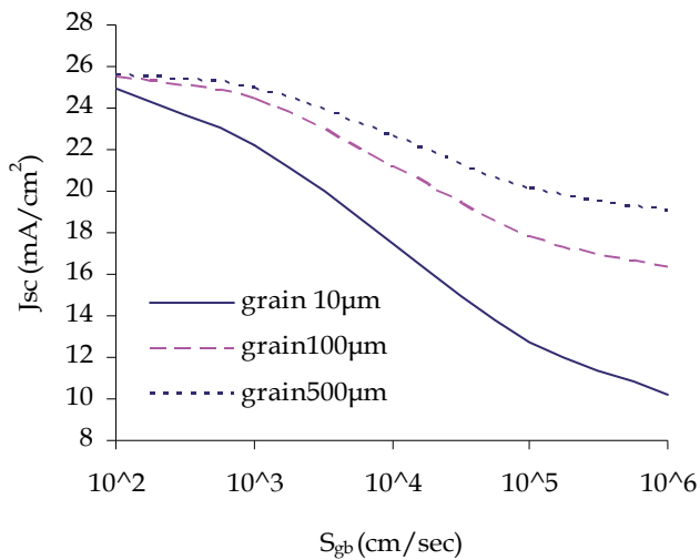
Fig. 8. Optimal short circuit current dependence on grain boundary recombination velocity S_{gb} of the cell B2, with grain size as parameter.
