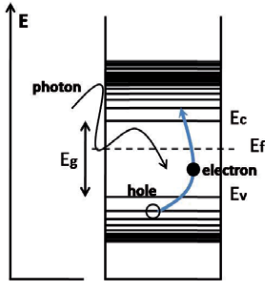
Fig. 7. Transition state probability illustration [4].
