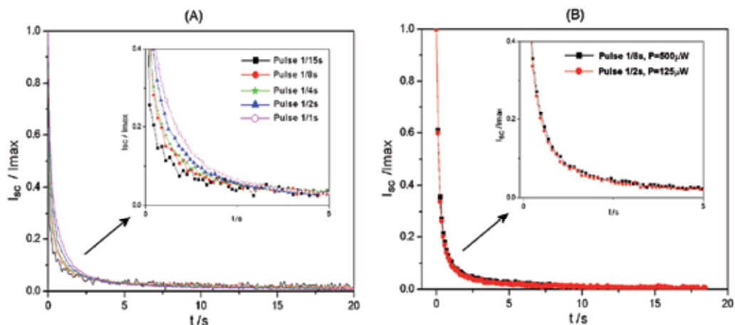
Fig. 5. (A) Time-evolution curve of the discharge process for a cell irradiated with a 532 nm laser, a power of 350 \mu\text{W} , and different exposure times to the radiation. (B) Comparison of two time evolution curve of the discharge process in which the photonic energy is identical but has been generated with different irradiation power and exposure time.
