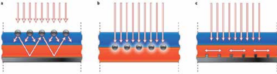
Fig. 13. Plasmonic light-trapping geometric for thin-film solar cells.[Atwater & Polman, 2010]
