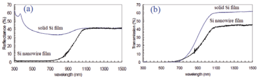
Fig. 29. Total (a) reflectance and (b) transmission data from integrated sphere measurements for 11 \mu\text{m} thick solid Si film and nanowire film on glass substrate (Tsakalakos et al., 2007).
