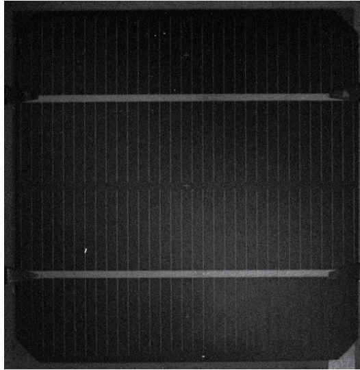
Fig. 19. Photoluminescence of solar cell 24B3 illuminated by UV-400 nm light, scan through blue filter (380- 460nm) - no strong luminescence.
