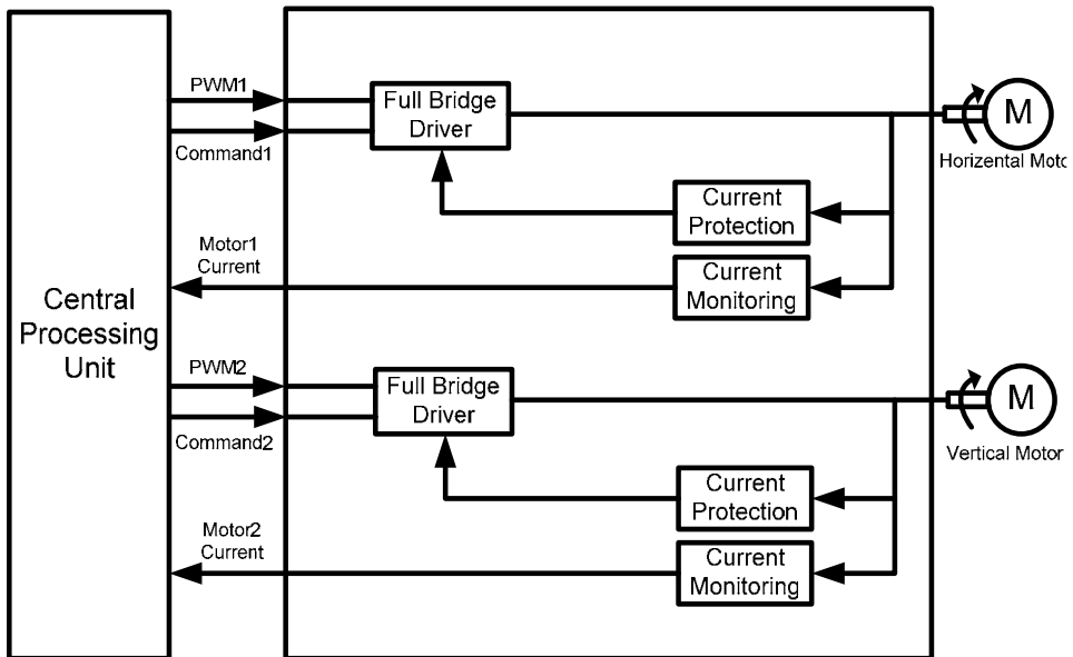
Fig. 7. Motor driver block diagram
