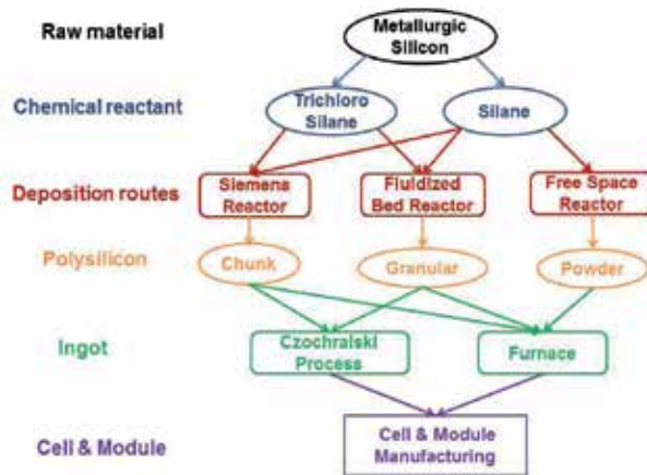
Fig. 4. Silicon based Solar Cell Production Process.
