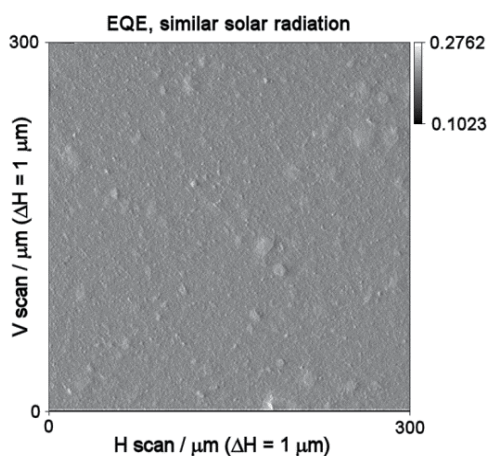
Fig. 17. EQE image approximated to solar radiation for a dye-sensitized solar cell.
