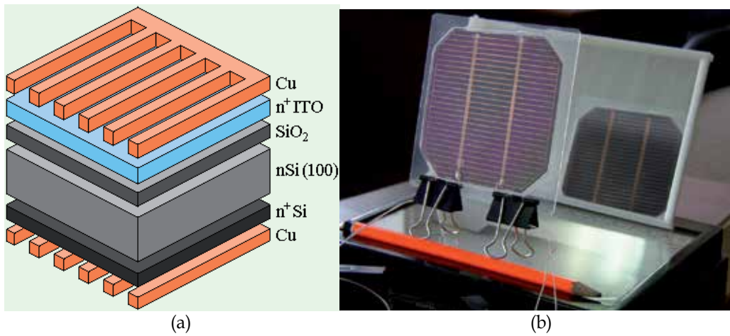
Fig. 23. The schematic a) and real b) view of the ITO/nSi BSC
