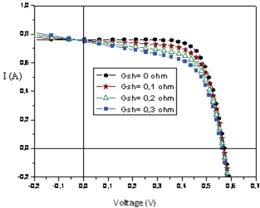
Fig. 10. Effect of shun resistance on the I-V characteristics of an illumination solar.
