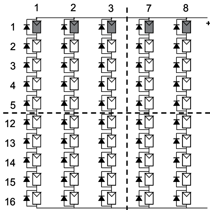
Fig. 11. Array ( N_S = 16 , N_P = 8 ) with shading patterns - Configuration 3
