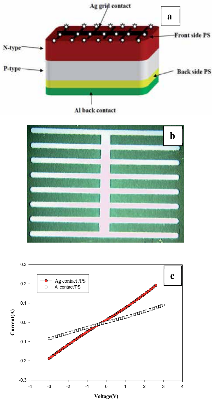
Fig. 2. Solar cells setup (a) p-n junction layers, (b) metal mask, and (c) contact I-V characterization
