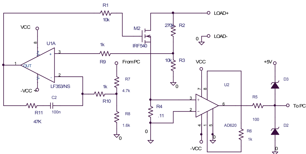
Fig. 11. The schematic diagram of continuous electronic load
