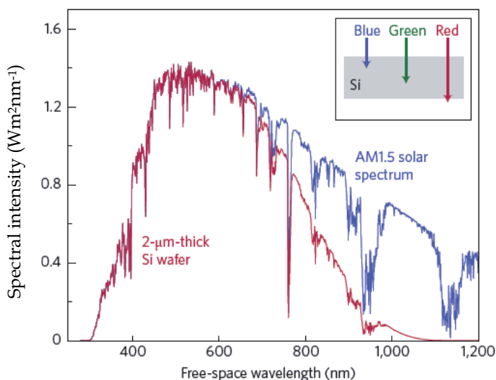
Fig. 10. AM1.5 solar spectrum, together with a graph that indicates the solar energy absorbed in a 2 \mu\text{m} -thick crystalline Si film (assuming single-pass absorption and no reflection). [Atwater & Polman, 2010]
