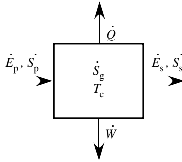
Fig. 2. Generalized schematic diagram of an energy converter. In the radiative limit, the energy flows pumped to and sunk by the converter ( i.e. \dot{E}_p and \dot{E}_s ) are limited to the radiant energy flux [ \text{J m}^{-2} \text{s}^{-1} ] pumped to and sunk by the converter: \dot{E}_p and \dot{E}_s , respectively.
