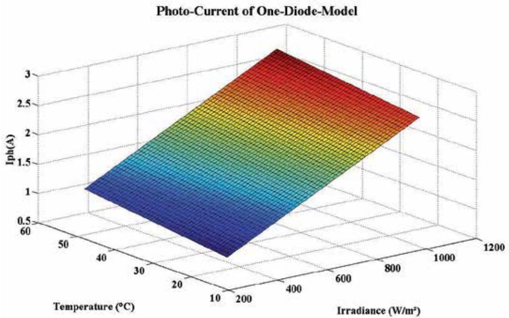
Fig. 15. Fitted sheet on photo-current of one-diode model by MATLAB.
