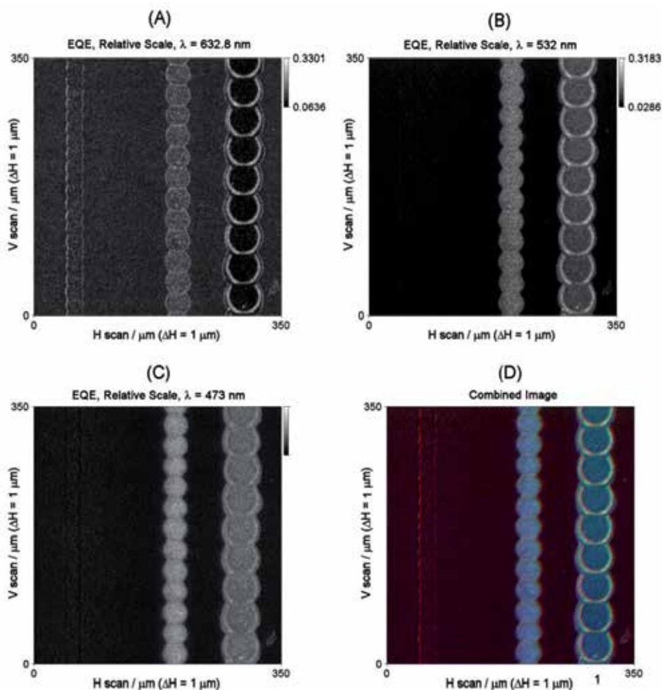
Fig. 12. LBIC images of the three high resolution scans performed using EQE values on a relative scale for each image and the combined image using all three.
