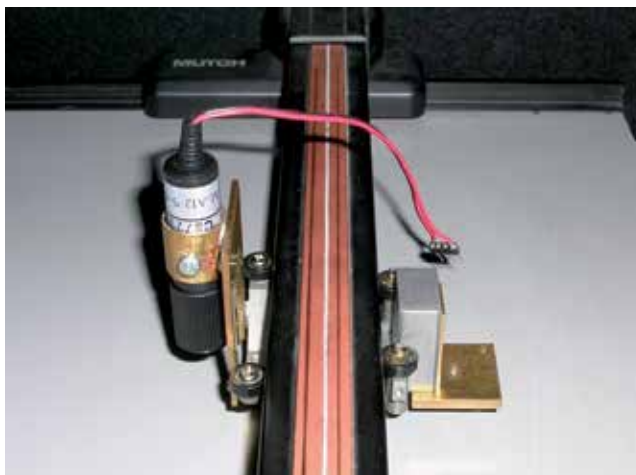
Fig. 4. Laser used in LBIC
