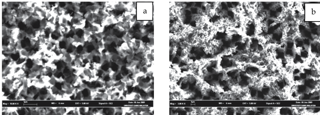
Fig. 3. SEM images of PS formed on (a) N (100), (b) P (100)
