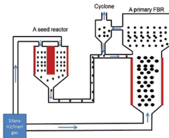
Fig. 6. Fluidized bed reactor with seed generator.
