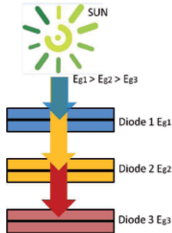
Fig. 10. Multi-junction and cell tandem concept.
