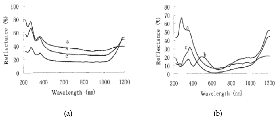
Fig. 5. Reflectance curves of polysilicon textured with the chemical etching. (a) Without ARC; (b) With SiN ARC. (a-NaOH texturing; b-NaOH after acidic texturing; c-Acidic texturing). [Meng, 2001]
