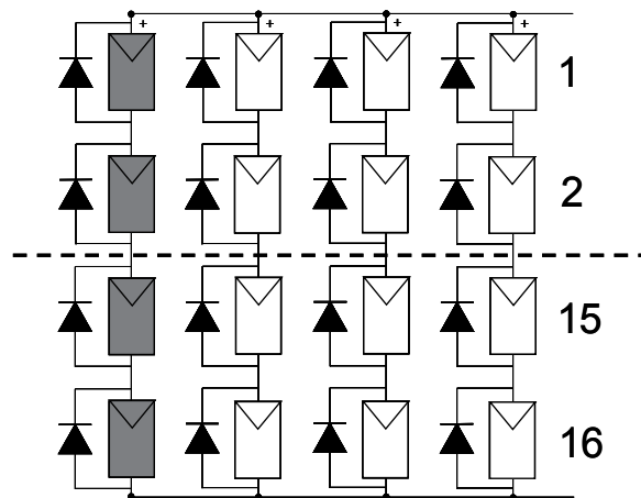
Fig. 10. Array ( N_S = 16, N_P = 4 ) with shading patterns - Configuration 2
