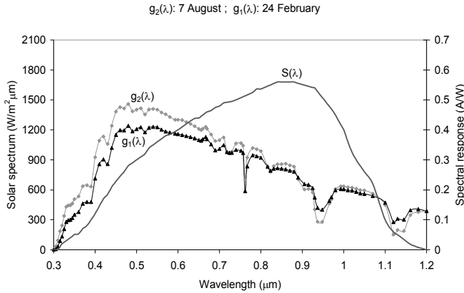
Fig. 1. Comparison of solar spectra in winter and summer.
