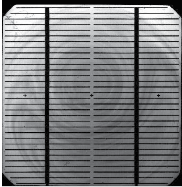
Fig. 8. Analyses of output local current of the sample no. 1 by usage of focused LED diode with middle wavelength 560 nm (green LED, T=297 K)
