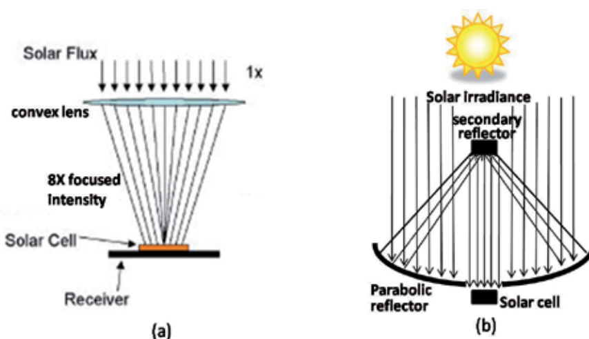
Fig. 21. Two examples of concentrating system engineering concepts with (a) convex lens and (b) parabolic reflector [2].
