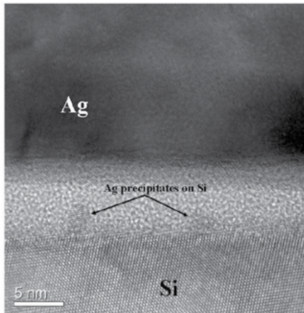
Fig. 6. HRTEM contrast of the Ag embryos on Si-bulk. This results in Ag-bulk/thin-glass-layer/Si contact structure.
