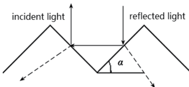
Fig. 1. Light trapping by "pyramid" covered at the textured surface.
