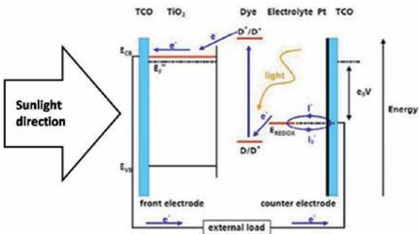
Fig. 25. The principles work of DSSC.
