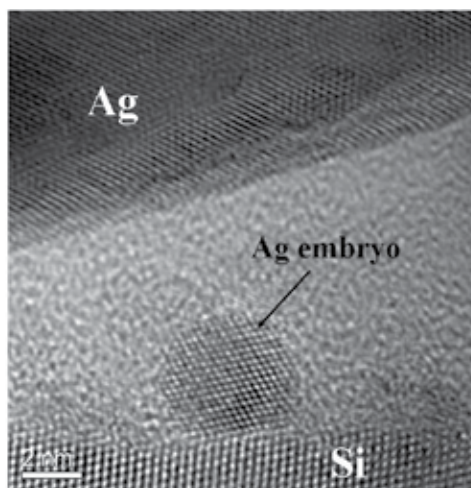
Fig. 11. Cross-sectional HRTEM of the Ag embryos on Si-bulk. This results in Ag-bulk/thin-glass-layer/Si contact structure.
