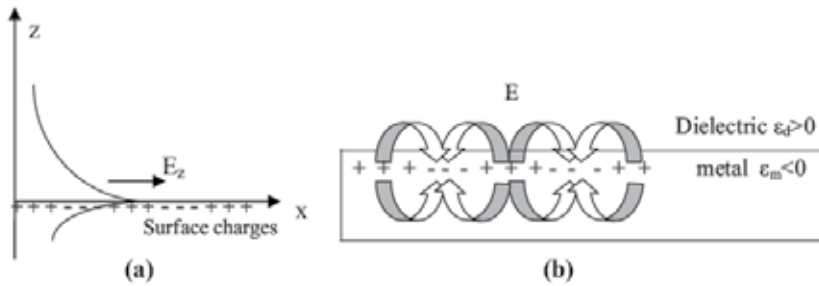
Fig. 11. (a) Schematic of a surface plasmon at the interface of a metal and dielectric showing the exponential dependence of the field E in the z direction along with charges and (b) electromagnetic field of surface plasmons propagating on the surface in the x direction. [Pillai, 2007]
