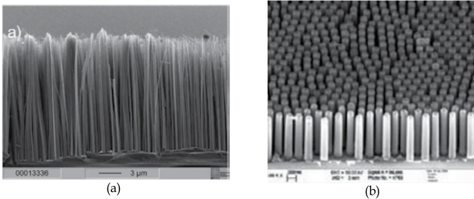
Fig. 27. SEM images of Si NWs obtained by (a) simple metal-assisted etching technique (Andra 2008) and (b) by colloidal crystal patterning combined with metal-assisted etching approach (Wang et al., 2010).
