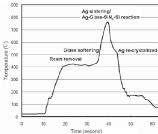
Fig. 2. A typical firing profile of a commercial crystalline silicon solar cell.
