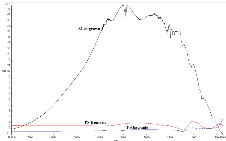
Fig. 13. FTIR reflection spectra of Si (as grown) and PS of both sides
