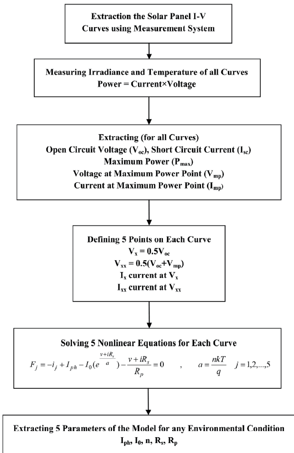
Fig. 4. Flowchart of extraction the one-diode model parameters
