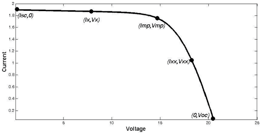
Fig. 2. Five points on the I-V curve of a solar panel are used to solve the nonlinear equations.
