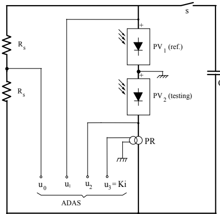
Fig. 5. "Series type" bridge measuring circuit.
