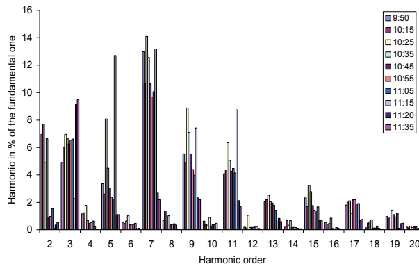
Fig. 28. Histogram of the harmonic currents (inverter 2).
