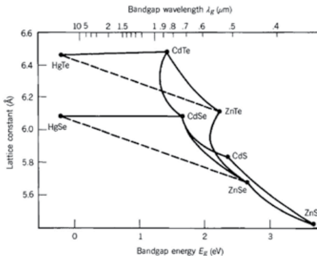
Fig. 13. Lattice constants, bandgap energies and bandgap wavelengths for important II-VI binary compounds [4].
