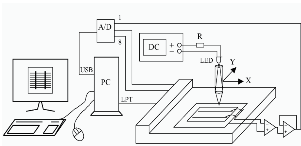
Fig. 1. Diagrammatical demonstration of measuring system (Vanek J, Fort T, 2007)
