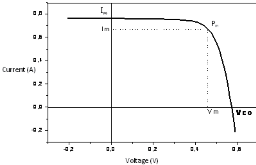
Fig. 2. Solar cell I-V Characteristics.
