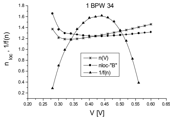
Fig. 6. Comparison for n_{loc} (Vasic et al., 2005).
