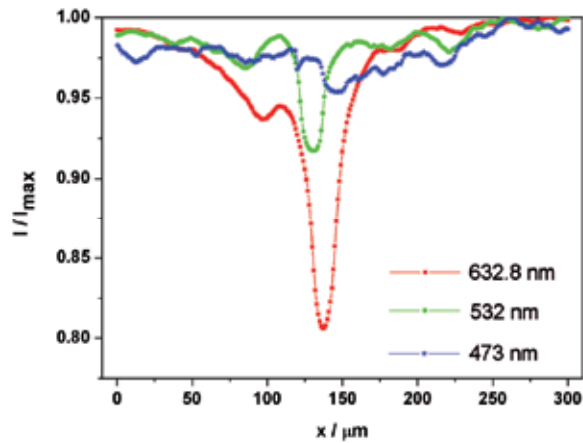
Fig. 11. Average LBIC signal profiles obtained for each of the three high resolution scans performed of a grain boundary.
