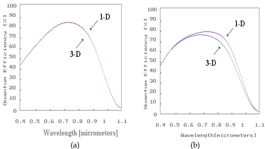
Fig. 12. Optimized external quantum efficiency and comparison with 3D model, for the cells B2 (a) and T2 (b), evaluated for experimental values included in tables 3 and 4.
