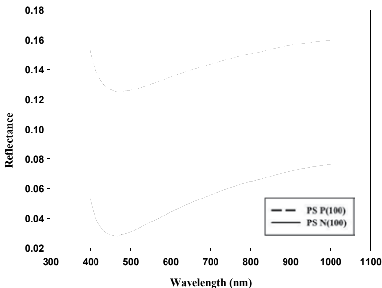
Fig. 5. Reflectance spectra for PS N (100) and P (100)
