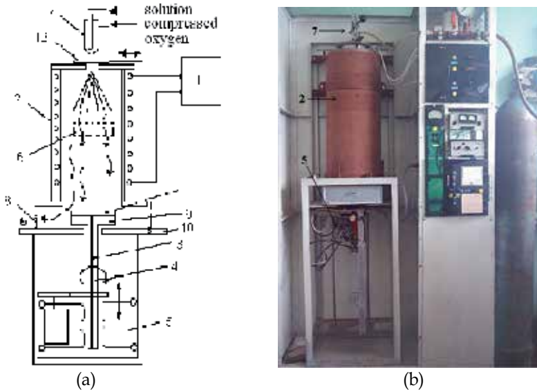
Fig. 15. Schematic a) and real b) view of the installation for ITO thin films deposition
