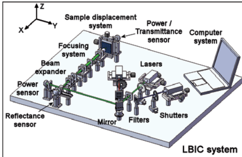
Fig. 1. General outline of the LBIC system.
