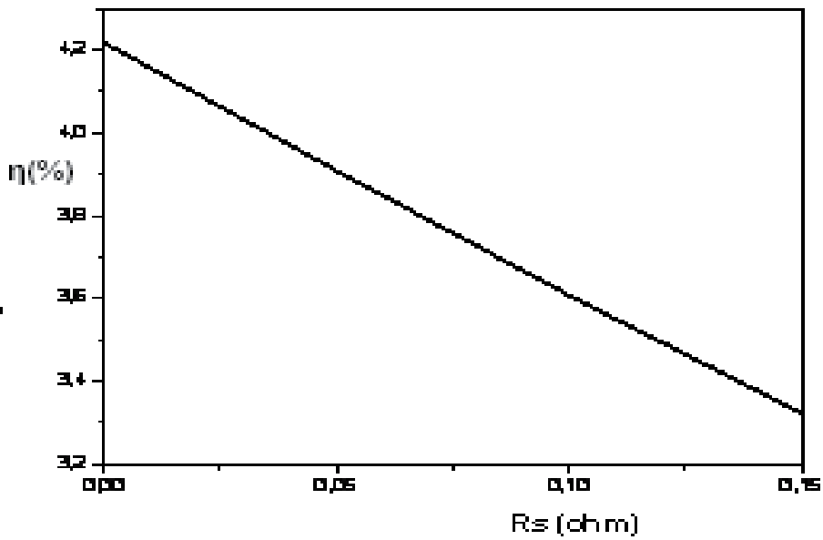
Fig. 8. Effect of series resistance on the \eta and FF.
