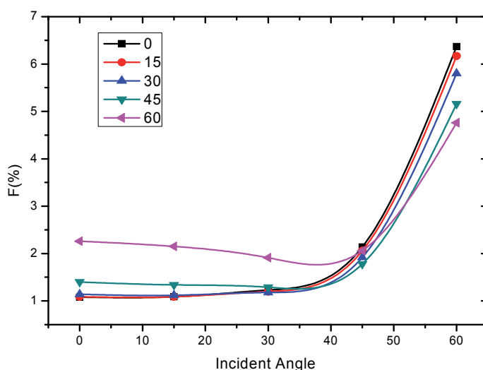
Fig. 9. Weighted average reflectance of double-layer anti-reflection coatings versus different incident angles.[ Chen & Wang, 2008]
