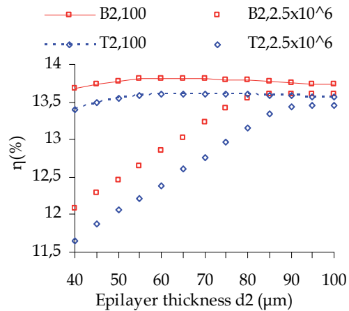
Fig. 4. Efficiency graph versus base thickness d_2 of the cells under investigation, calculated for S_{eff} = 100 cm/ sec and 2.5 \times 10^6 cm/sec.
