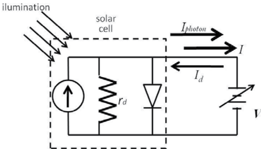
Fig. 3. The equivalent circuit model of an ideal diode solar cell.
