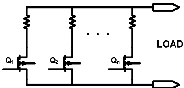
Fig. 8. The proposed switching load circuit
