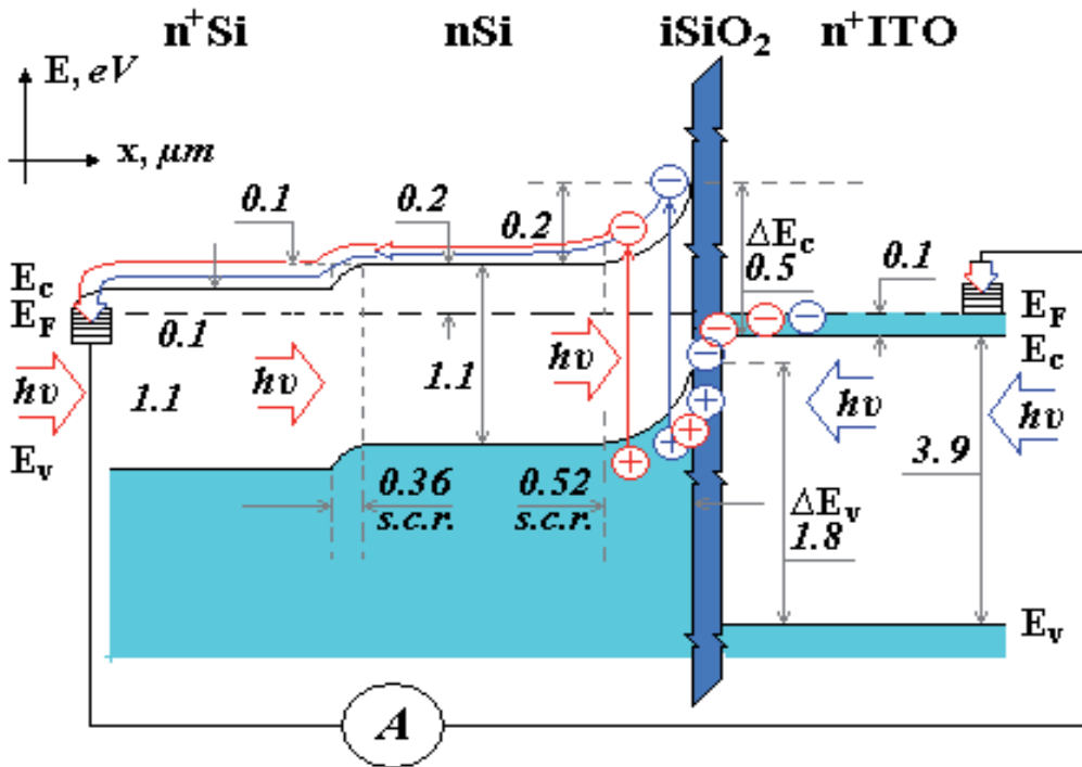
Fig. 28. Energy band diagram of the bifacial \text{Cu}/n^+\text{ITO}/\text{SiO}_2/n\text{Si}/n^+\text{Si}/\text{Cu} structure
