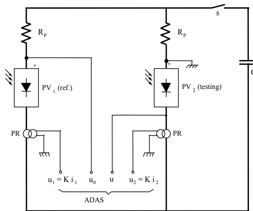
Fig. 6. "Parallel type" bridge measuring circuit.
