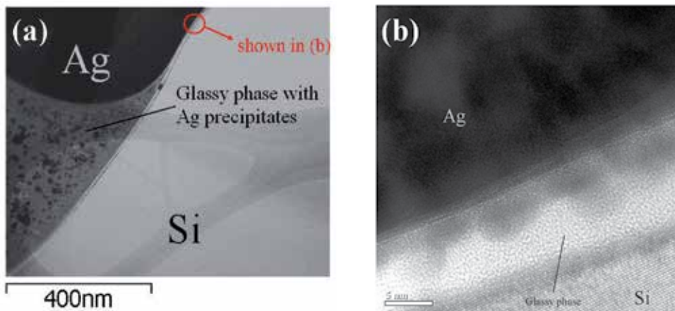
Fig. 4. (a) TEM bright field cross-sectional image of the the Ag-bulk/Si contact structure with localized large glassy-phase region. (b) HRTEM of the Ag-bulk/Si interface. There is a very thin glass layer between Si and Ag-bulk.
