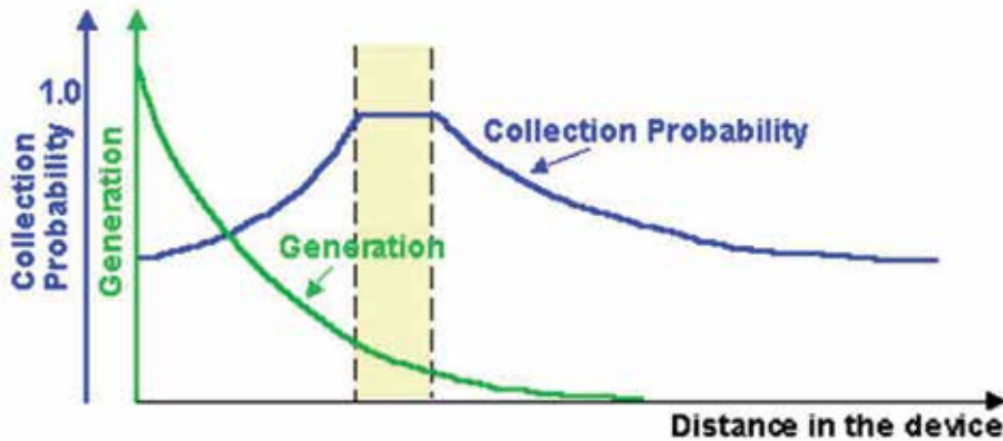
Fig. 8. The collection probability of the generated hole-electron pairs at junction [5].
