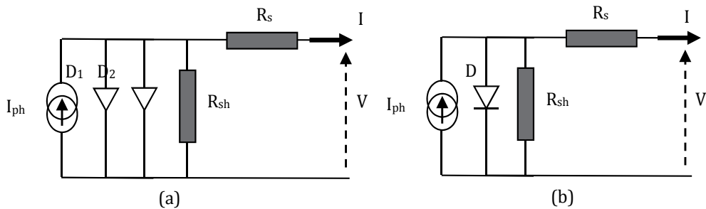
Fig. 1. Scheme of the equivalent electrical circuit of an illuminated solar cell: (a) the double diode model, and (b) the one diode model.
