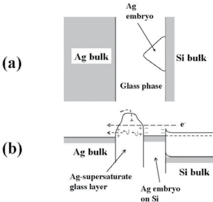
Fig. 12. (a) Schematic cross-section drawing of the Ag-embryo on Si-bulk. (b) Schematic energy-band drawing of a possible conductance mechanisms across Ag-bulk/thin-glass-layer/Si contact structure.
