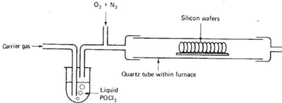
Fig. 22. Chemical (phosphorus) diffusion process [2].
