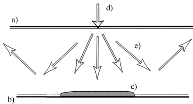
Fig. 18. Theory of projection back side contact during secondary emission of long wavelength light.
