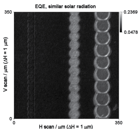
Fig. 13. EQE image approximated to solar radiation using equation (14) for an amorphous thin film silicon solar cell.
