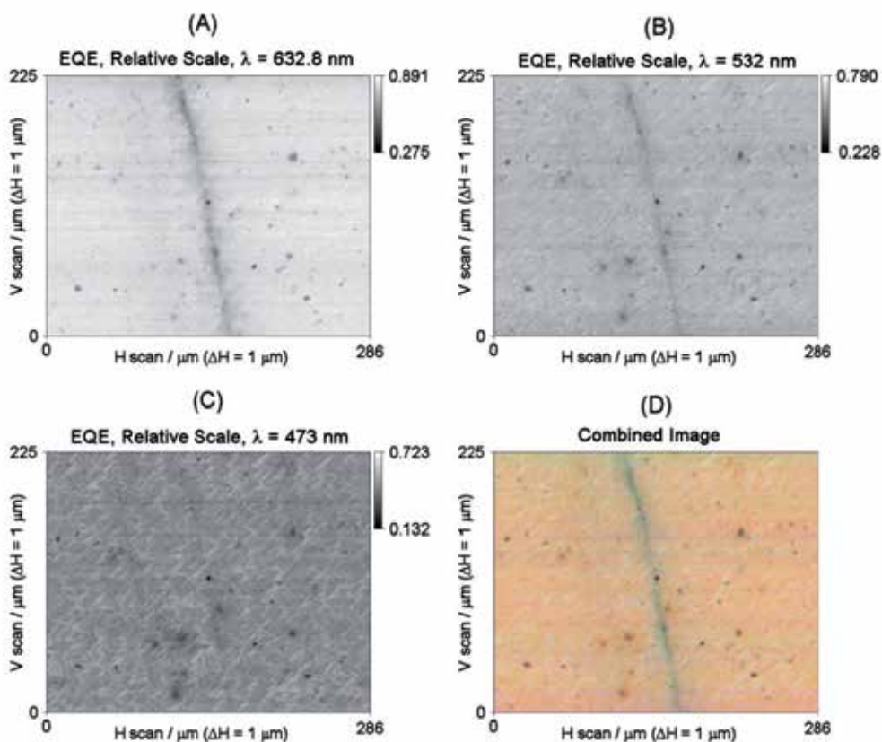
Fig. 10. LBIC images obtained of the three high resolution scans (1 \mu m) performed using EQE values on a relative scale for each image and the combined images using all three.
