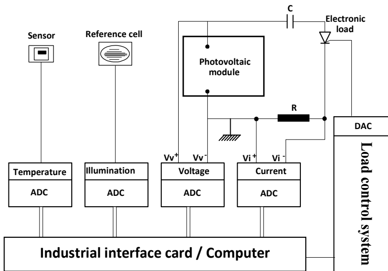
Fig. 11. Block diagram of the PV module tester.
