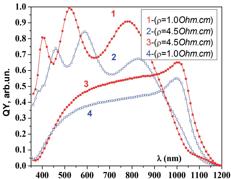
Fig. 24. Spectral distribution of the quantum efficiency 1, 2-frontal illumination; 3, 4-rear illumination
