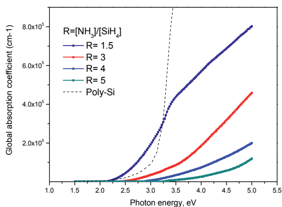
Fig. 14. Global absorption coefficient of \text{SiN}_x layers of different stoichiometries with embedded Si QDs. The absorption coefficient of poly-Si is also presented for comparison (Nychporuk et al., 2008).
