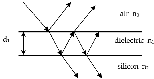
Fig. 6. The principles of the antireflection coating.
