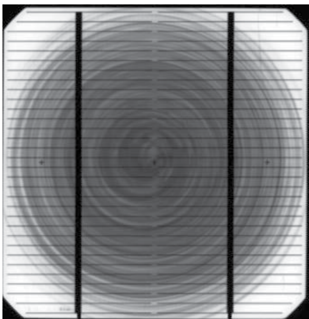
Fig. 12. Analyses of output local current of the sample no. 3 by usage of focused infrared laser (830nm, T=297 K)
