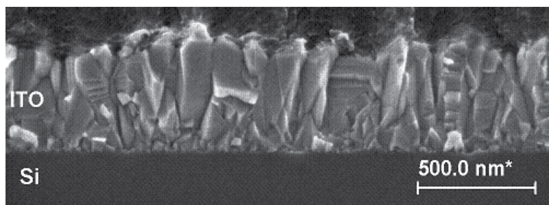
Fig. 17. SEM image of ITO film
