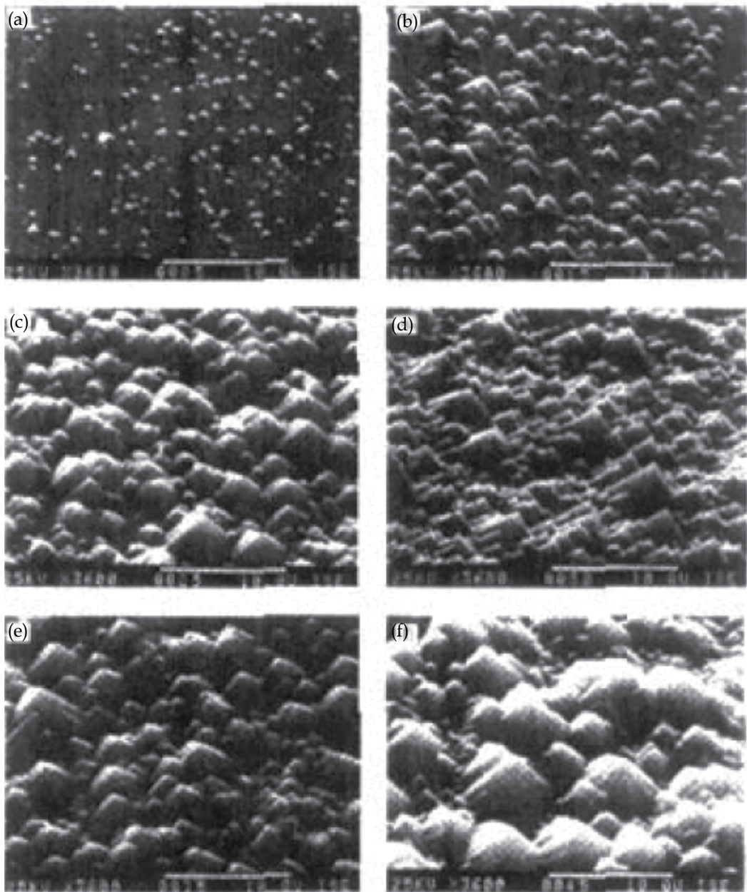
Fig. 2. The SEM pictures of textured surface with the corrosion time, the corrosion time are: (a)5min,(b)15min,(c)25min, (d)30min,(e)35min, (f)40min, respectively.[Wang, 2005]
