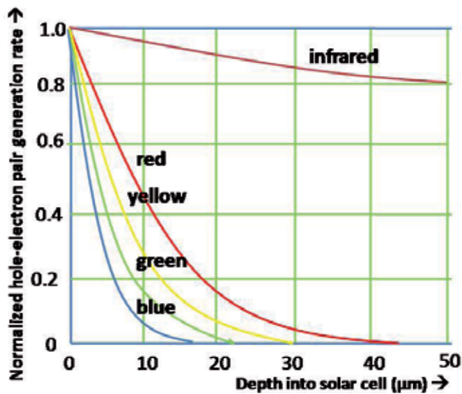
Fig. 6. A normalized hole-electron pair generation rate [2].
