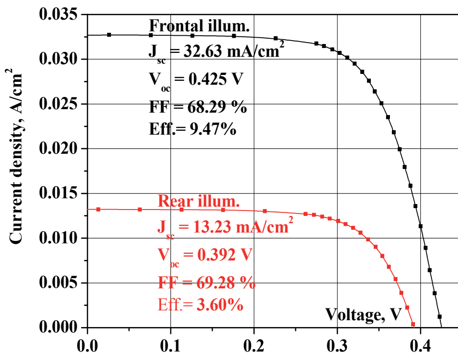
Fig. 25. The I-V load characteristics and the photoelectric parameters of the elaborated BSC at AM1.5 spectral distribution and 1000W/m 2 illumination
