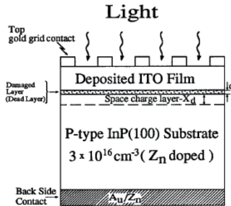
Fig. 7. Schematic diagram of the ITO/InP photovoltaic device obtained by ion beam sputtering.
