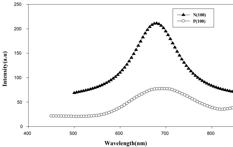
Fig. 7. PL spectra of PS prepared by electrochemical etching
