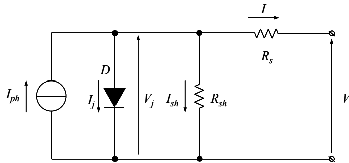
Fig. 3. Equivalent circuit of solar cell with one exponential.
