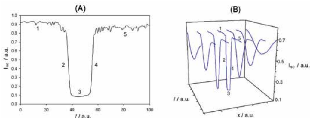
Fig. 2. (A) I_{sc} -curve obtained after performing a linear scan along a l superficial coordinate on a Si(MC) solar cell and through a current collector. (B) I_{sc} -curve generated at different positions of the focal lens along X -axis.
