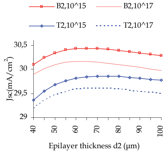
Fig. 5. Variation of the short circuit current density J_{sc} of the cells, as a function of base thickness d_2 calculated for doping concentration values of 10^{15}\text{cm}^{-3} , and 10^{17}\text{cm}^{-3} .
