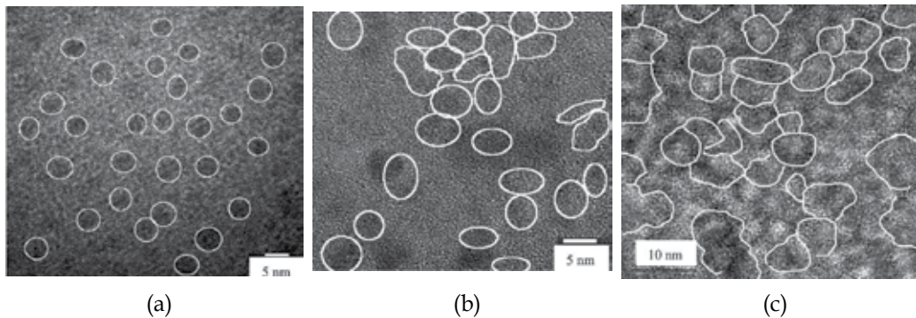
Fig. 15. HRTEM images of the ensembles of Si QDs corresponding to different structural-electrical regimes: (a) uniformly dispersed isolated spherical QDs (regime a), (b) clusters of "touching" QDs (regime c) and (c) percolation clusters of "touching" QDs (regime e) (Antonova et al., 2008).
