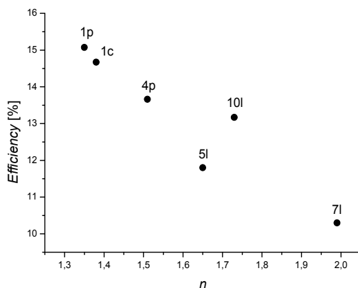
Fig. 8. Efficiency dependence on the ideality factor (Vasic et al., 2000).
