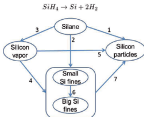
Fig. 7. Reaction pathways for conversion of silane to silicon. (Lai et al., 1986)
