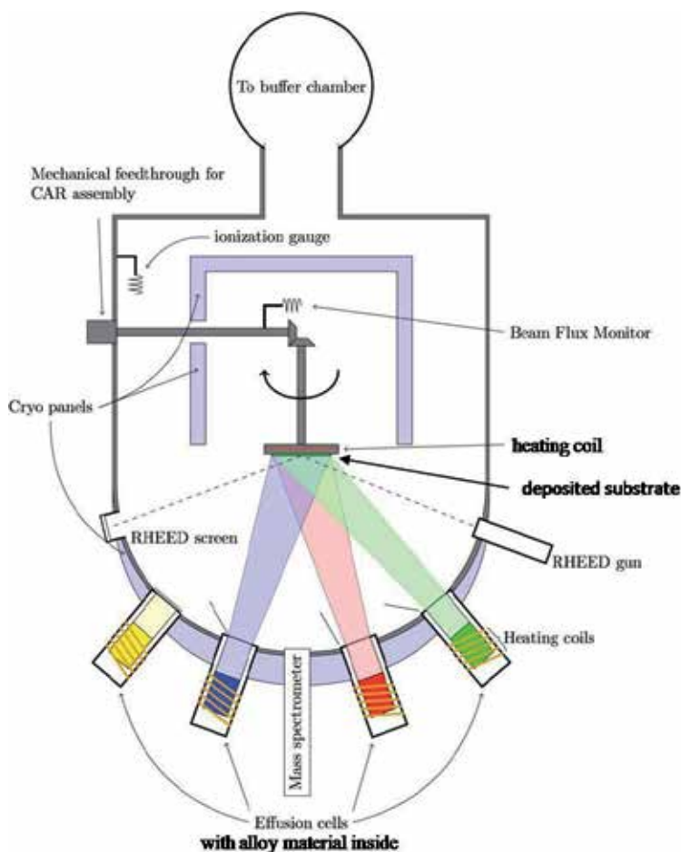
Fig. 23. Molecular beam epitaxy components [8].
