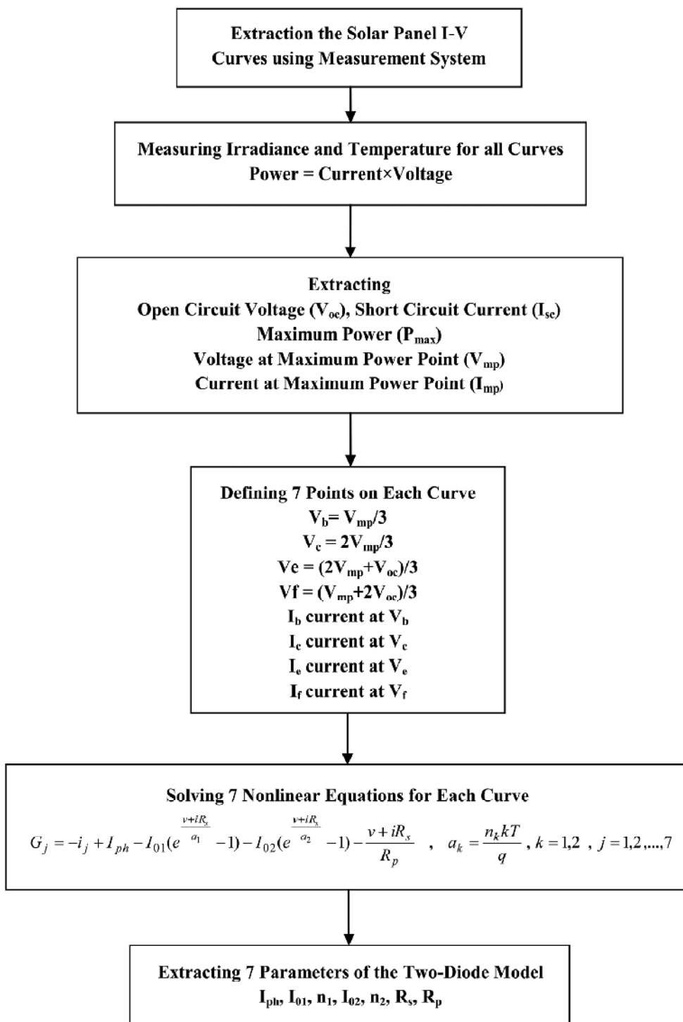
Fig. 5. Flowchart of extraction the two-diode model parameters
