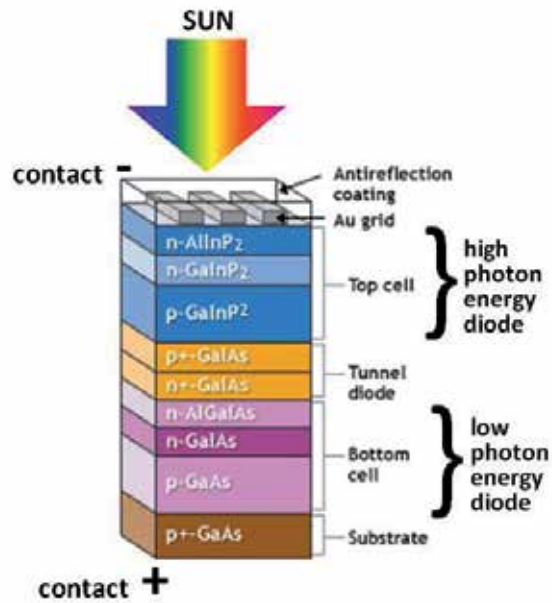
Fig. 11. Typical of high efficient solar cell with dual cell tandem structure [12] .
