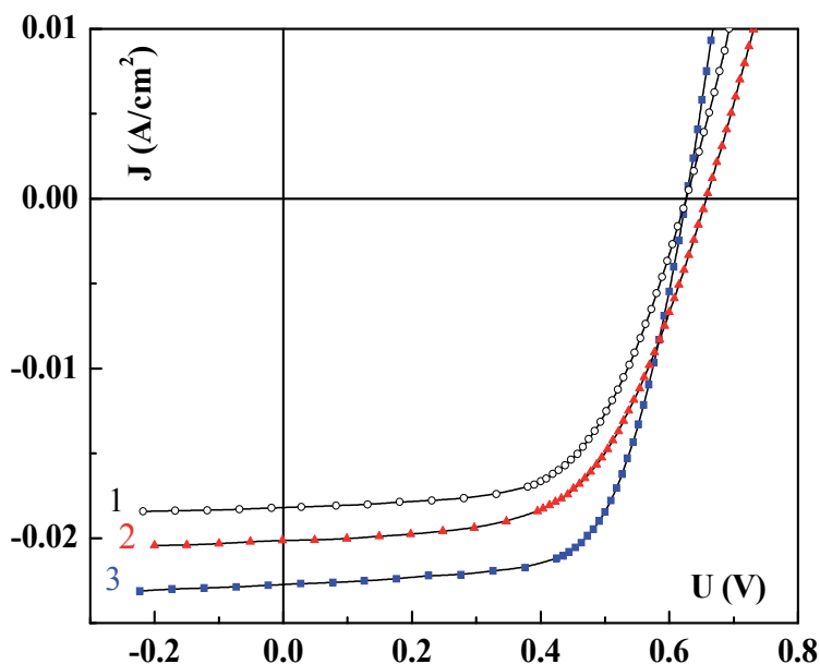
Fig. 12. Load I-V characteristics of Cu/nITO/pInP/Ag:Zn solar cells: 1-before thermal treatment; 2-after thermal treatment in H_2 ; 3-best parameters after thermal treatment in H_2
