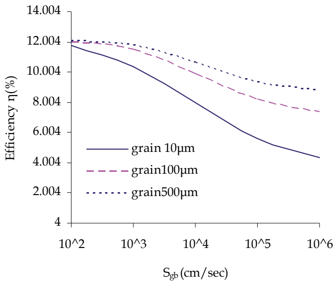
Fig. 9. Variation of efficiency \eta of the cell B2, as a function of grain boundary recombination velocity S_{gb} , calculated for optimal base thickness and variable grain sizes.
