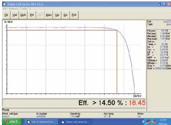
Fig. 8. Experimental I-V curve of the solar cell performed with the Pasan machine.
