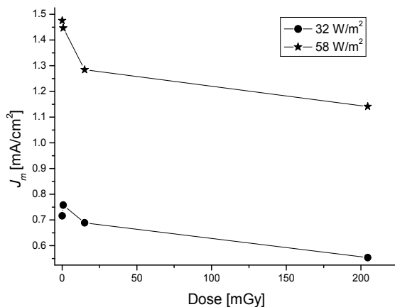
Fig. 14. Dependence of the J_m on doses (Vasic et al., 2008).
