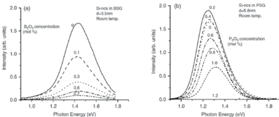
Fig. 9. PL spectra of (a) B-doped (Mimura et al., 1999) and (b) P-doped Si nanocrystals (Fujii et al., 2002) at room temperature for different doping concentrations.
