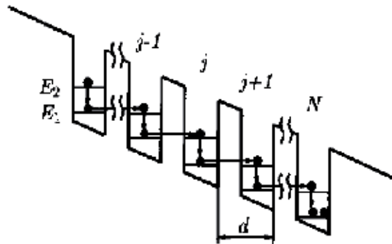
Fig. 18. Sequential resonant tunneling transfer in multiple-quantum-well structure. E_1 and E_2 are the energies of the ground and first excited states in the quantum well, respectively, and d the superlattice period (Raisky et al., 1999).
