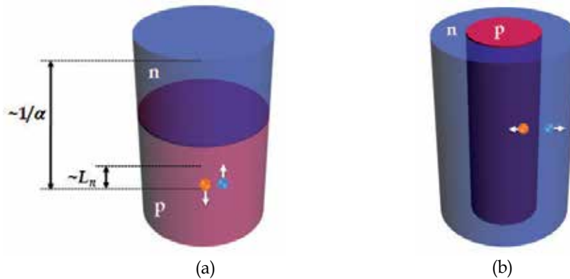
Fig. 30. Schematic views of the (a) axial and (b) radial nanowire solar cell. Light penetration into the cell is characterized by the optical thickness of the material ( \alpha is the absorption coefficient), while the mean free path of generated minority carriers is given by their diffusion length. In the case of axial nanowire solar cell, light penetrates deep into the cell, but the electron-diffusion length is too short to allow the collection of all light-generated carriers (Kayes et al., 2005).
