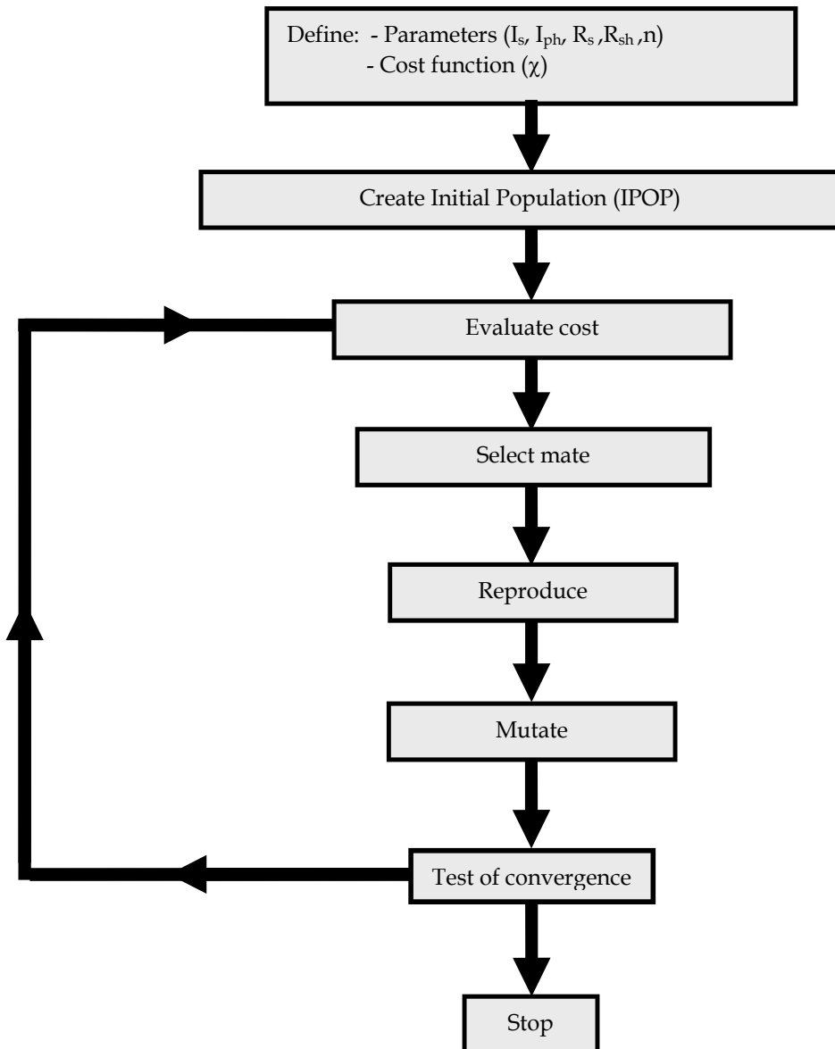
Fig. 7. Flow chart of the genetic algorithms.
