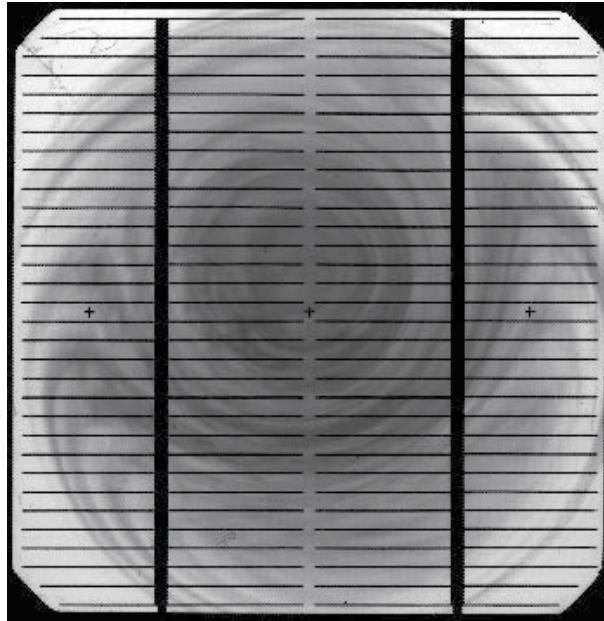
Fig. 6. Analyses of output local current of the sample no. 1 by usage of focused LED diode with middle wavelength 650 nm (red LED, T=297 K)
