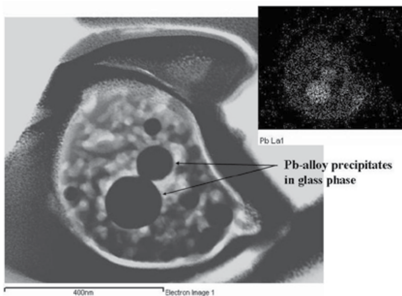
Fig. 8. TEM bright field image shows Pb precipitates in the glassy phase. The inset is the energy dispersive spectroscopy (EDS) mapping.
