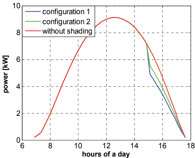
Fig. 21. The daily power diagrams in October for configurations 1 and 2 (Clear-sky)
