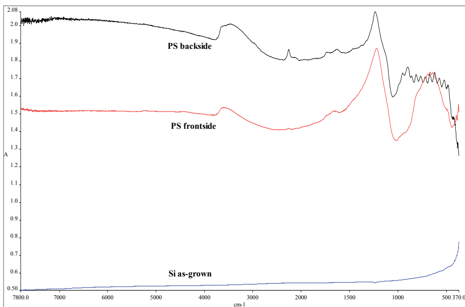
Fig. 14. FTIR absorption spectra of Si (as grown) and PS of both sides
