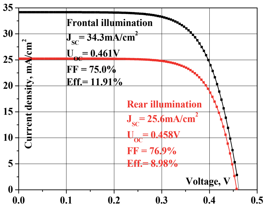
Fig. 27. Load I-V characteristic of n + ITO/SiO 2 /n/n + Si BSC with regular Si surface
