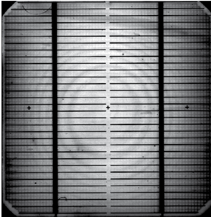
Fig. 17. Projection of back contact bar in LBIC of the sample 57A3 by usage of focused LED diode with middle wavelength 430 nm (blue LED, T=297 K)
