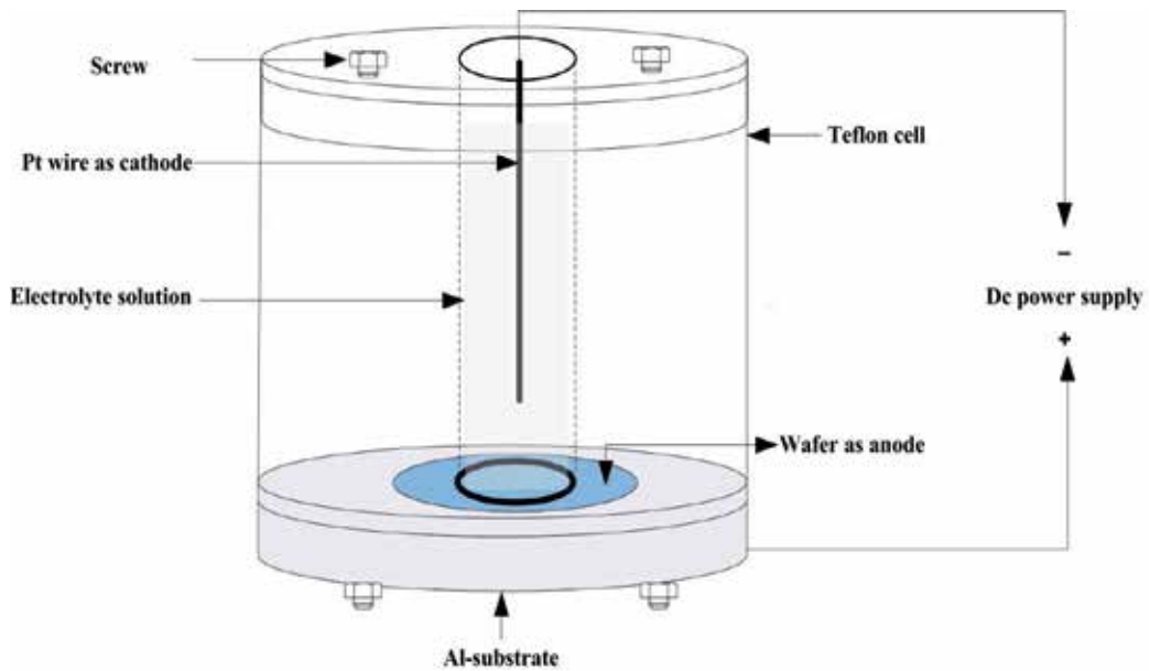
Fig. 1. Schematic of the electrochemical etching setup
