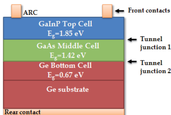
Fig. 3. Schematic view of GaInP/GaAs/Ge solar cell.
