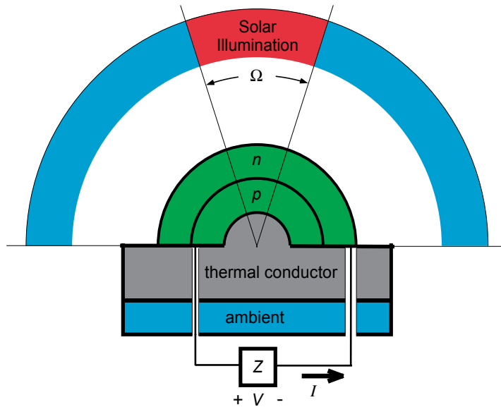
Fig. 3. Cross section of an abstracted p - n junction solar cell with spherical symmetry. The exaggerated physical symmetry reinforces the solar geometry, where a solid angle of the solar cell's surface, \Omega , is subtended by direct insolation from the sun and the remainder of the hemisphere is subtended by diffuse radiation from the atmosphere. The solid angle may be adjusted by geometrical concentration of the sun's light. The solar cell is maintained at the ambient temperature, the surface terrestrial temperature, by a thermal conductor.
