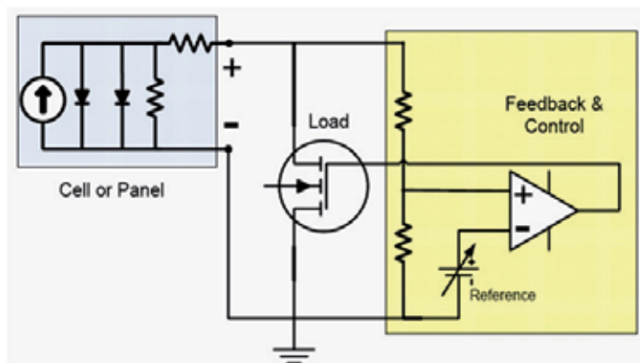
Fig. 9. The proposed continuous electronic load
