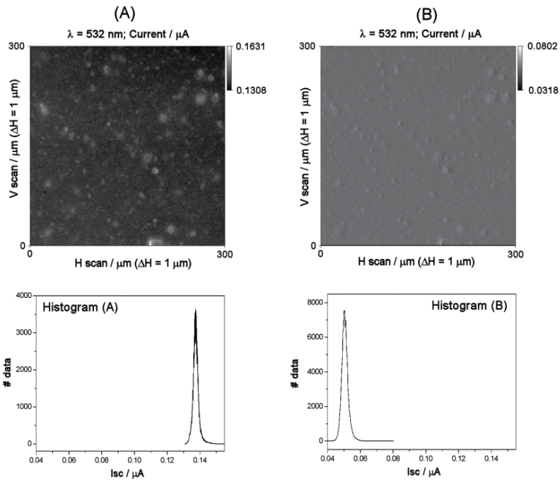
Fig. 15. (A) LBIC image for the DSSC using green laser. (B) The same image modified using our algorithm.
