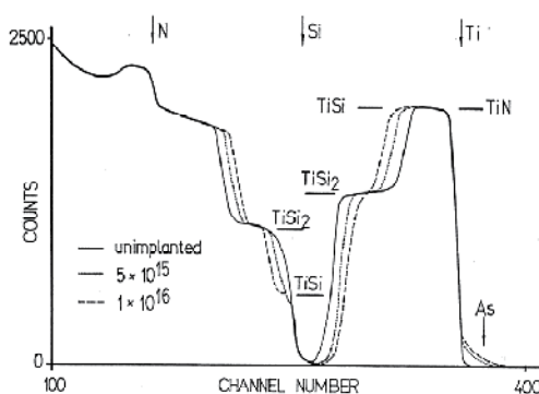
Fig. 1. RBS spectra of TiN/Ti/Si samples (Vasic et al., 2011).
