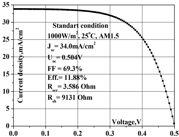
Fig. 5. Load I-V characteristic of ITO/SiO 2 /nSi solar cells with irregular landform Si surface
