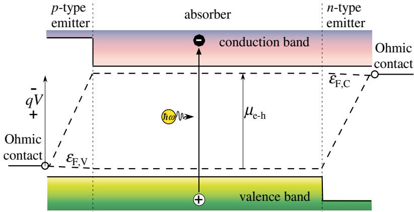
Fig. 1. Ideal structure of a solar cell. Shown is the absorber, which is sandwiched between an n -type emitter and a p -type emitter. An Ohmic contact is made to each of the emitters. A voltage, V , exists between the contacts of the solar cell.
