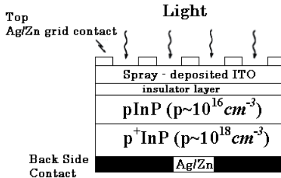
Fig. 8. Schematic diagram of the ITO/InP structure obtained by spray pyrolytic method.
