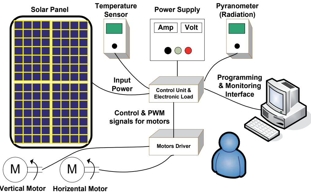
Fig. 6. Block diagram of the proposed measurement system
