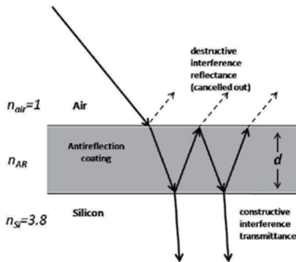
Fig. 15. Bragg reflection effect of mirror stacks structure with distance d = \lambda/4 .
