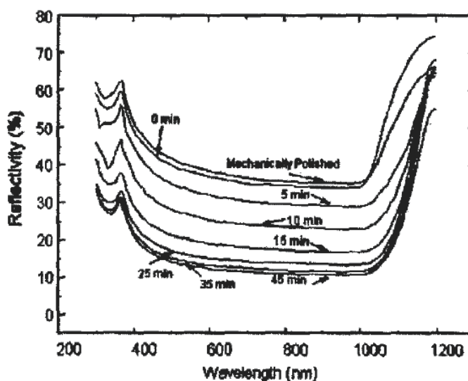
Fig. 3. The reflectivity of silicon wafers after different etching time.[Wang, 2005]
