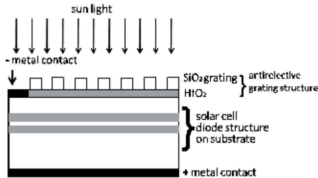
Fig. 19. Solar cell structure incorporating antireflective grating structure.
