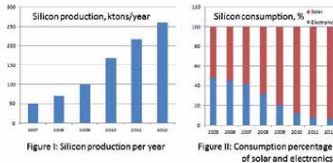
Fig. 2. Poly-Silicon Production and consumption for Electronic and PV Industries (Fishman, 2008).
