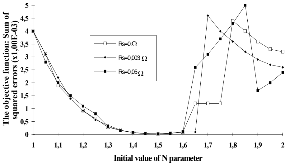
Fig. 5. Search path of the absolute minimum in R_s plans.
