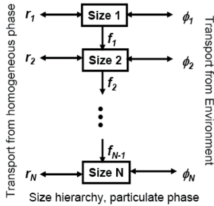
Fig. 8. The network representation of population balance
