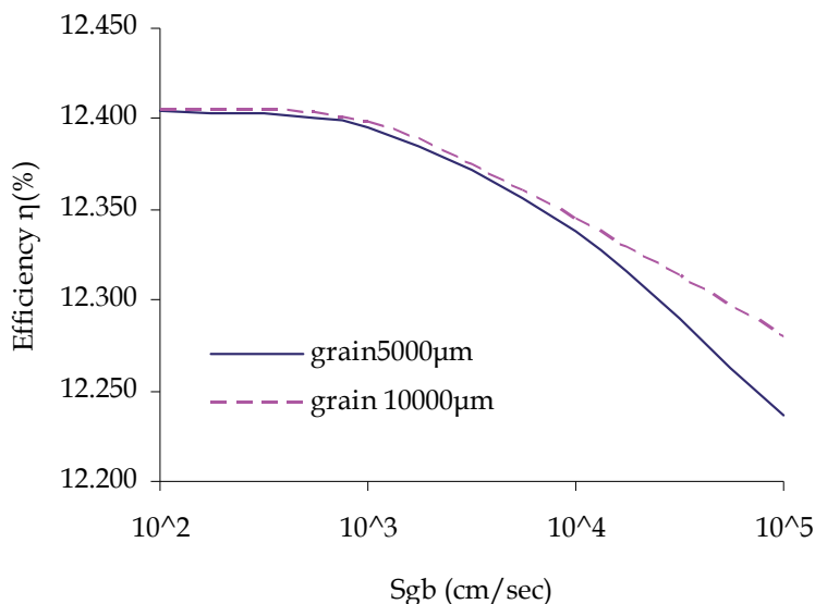
Fig. 11. Variation of the efficiency \eta as a function of grain boundary recombination velocity S_{gb} , calculated for optimal base thickness and variable grain sizes (cell T2).
