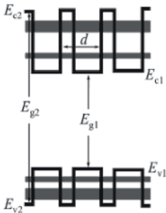
Fig. 17. The energy bandstructure of a semiconductor type-I heterostructure superlattice: E_{g1} and E_{g2} are the bandgaps, E_{c1} and E_{c2} are the bottoms of the conduction bands of narrow bandgap and wide bandgap semiconductors, respectively; d is the period of the heterostructure superlattice (Mitin, 2010).
