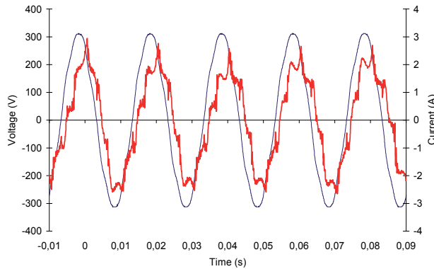
Fig. 27. AC waveforms of inverter 2 at 10.45.
