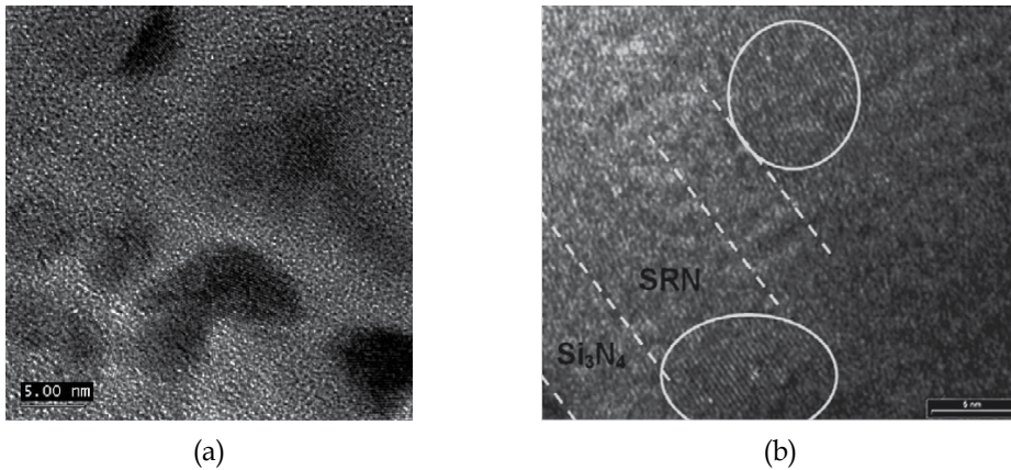
Fig. 6. In-situ grown Si QDs in the gas phase and dispersed in \text{Si}_3\text{N}_4 matrix: (a) One layer structure (Lelièvre et al., 2006); (b) multi-layer structure (Conibeer et al., 2008).
