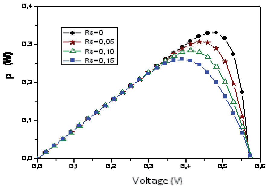
Fig. 7. Effect of series resistance on the P-V characteristics of an illumination solar cell.
