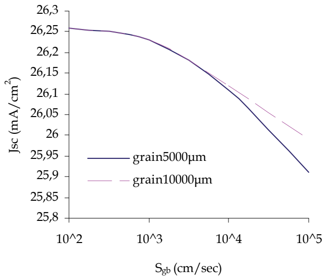
Fig. 10. Optimal short circuit current dependence on grain boundary recombination velocity S_{gb} of the cell T2, with grain size as parameter.
