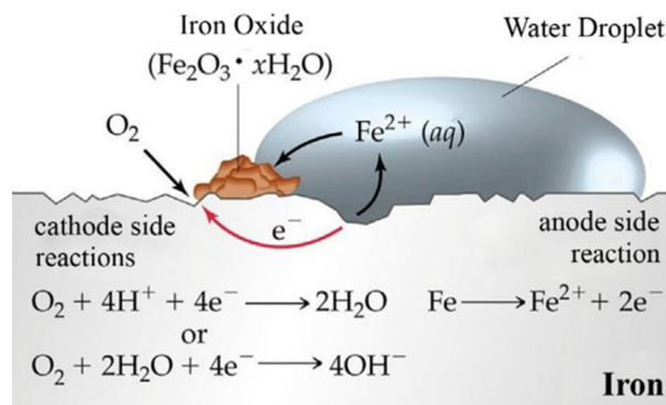
Fig. 2. Schematic representation for corrosion mechanism [15]
