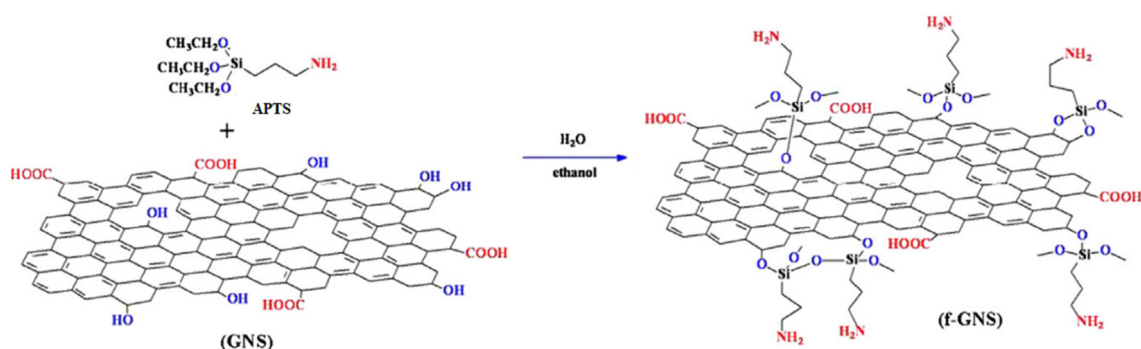
Fig. 10. Modification of Graphene with APTS [84]
