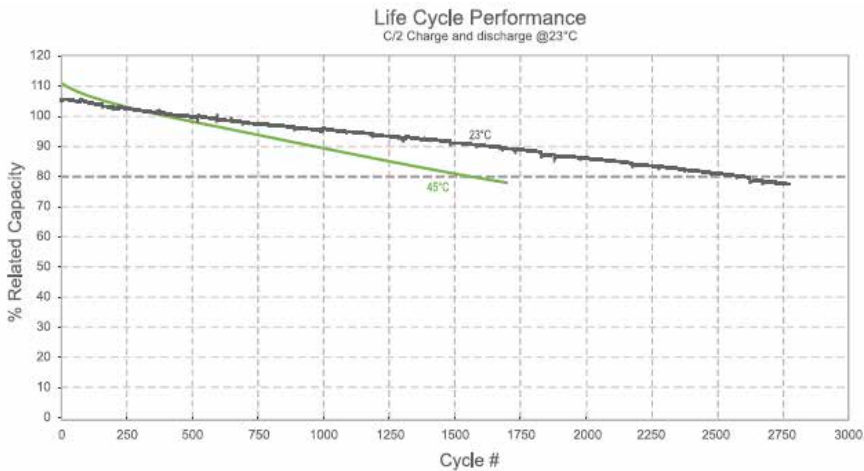
Fig. 6. Battery cycle life depends on operating temperature ( \text{LiFeMgPO}_4 ) (Valence Technology, 2010)
