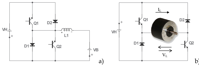
Fig. 9a,b. Two-quadrant dc-to-dc converter a) III-Q and IV-Q) b) I-Q and IV-Q
