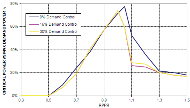
Fig. 19. Critical Power for baseline case under Demand Control.
