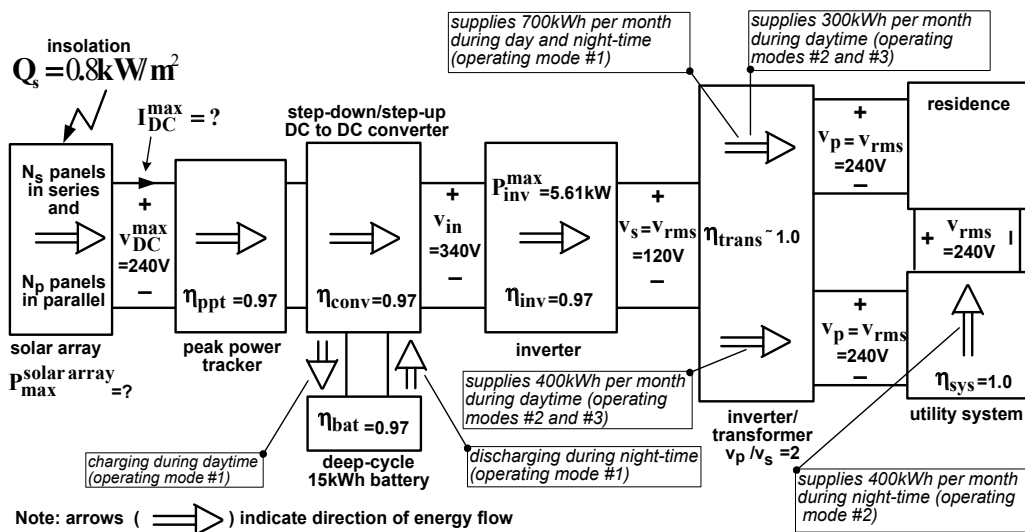
Fig. 8. Block diagram of a PV plant power plant for a residence
