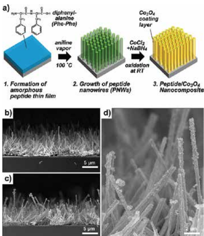
Fig. 17. Diphenylalanine- \text{Co}_3\text{O}_4 hybrid nanowires: (a) schematic illustration of the fabrication process of hybrid nanowires and SEM images of (b) the pure peptide nanowires and (c-d) the hybrid nanowires (Ryu et al., 2010b).
