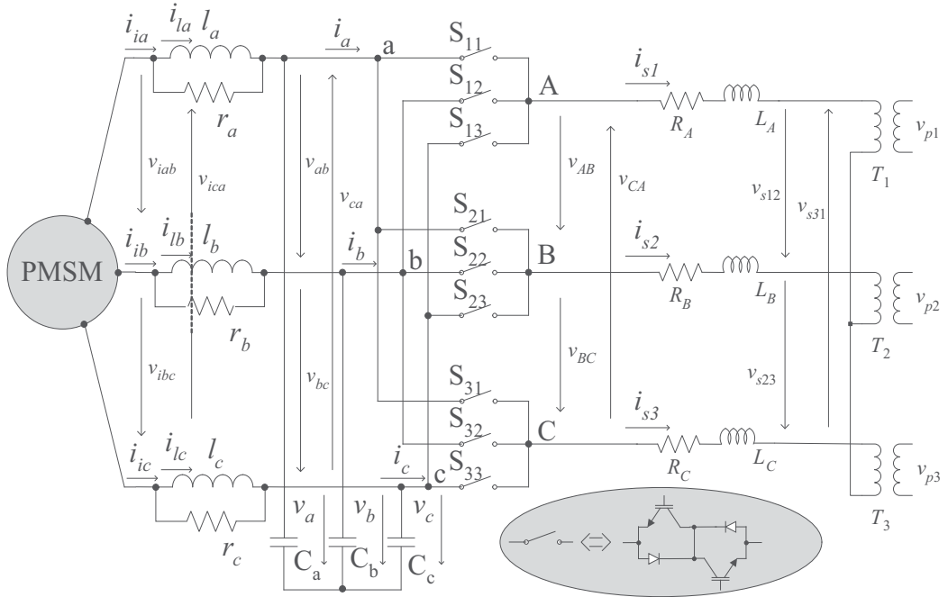
Fig. 5. Matrix converter topology.
