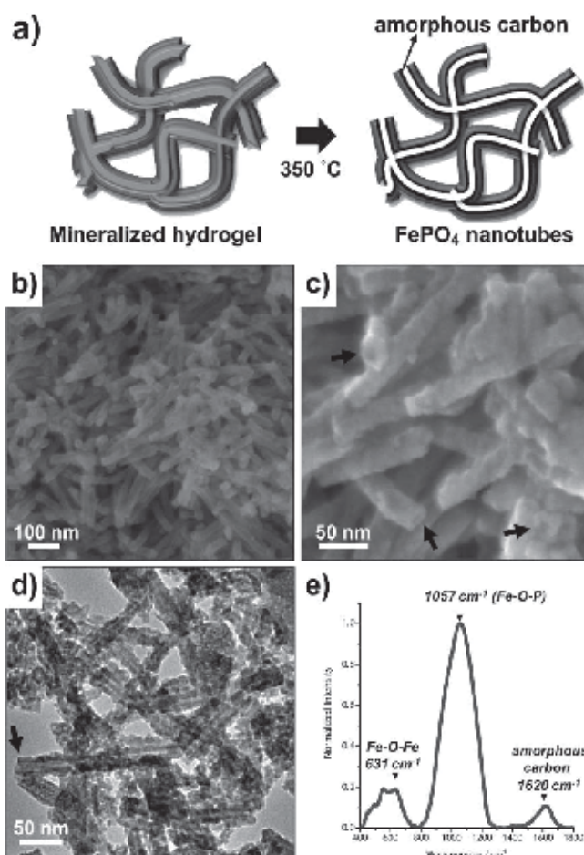
Fig. 24. Amorphous \text{FePO}_4 nanotube synthesized by a peptide template: (a) schematic diagram for synthesis procedure, (b-c) SEM images, (d) TEM image, and (e) FT-IR spectra (Ryu et al., 2010a).
