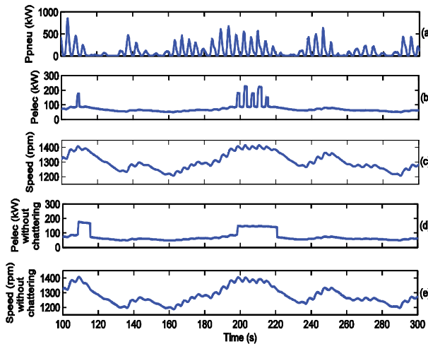
Fig. 17. Generator power and speed with and without the switched controller to prevent chattering for a given input pneumatic power.
