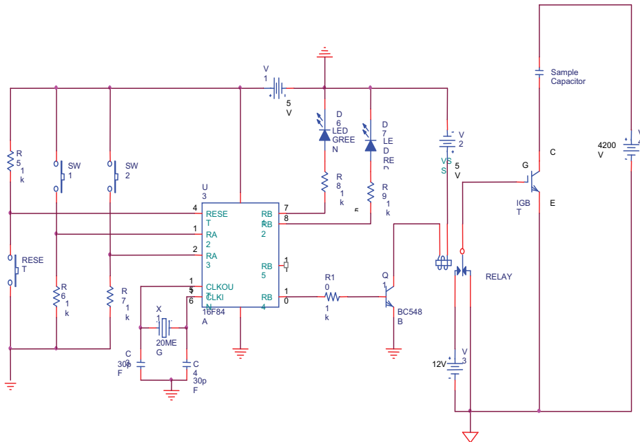
Fig. 7. Schematic diagram of the high speed switching circuit
