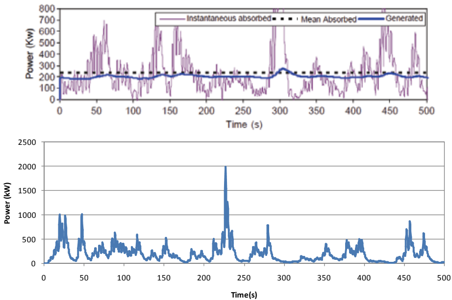
Fig. 13. Output electrical power time series from (top) attenuator device with significant hydraulic accumulator storage (bottom) OWC device with impulse turbine.
