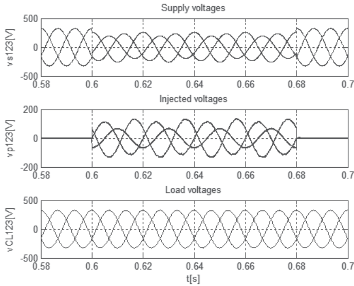
Fig. 15. Simulation result of DVR response to unbalanced voltage sag: Supply voltages ( v_1, v_2, v_3 ), Injected voltage ( v_{p1}, v_{p2}, v_{p3} ) and Load voltage ( v_{CL1}, v_{CL2}, v_{CL3} ).
