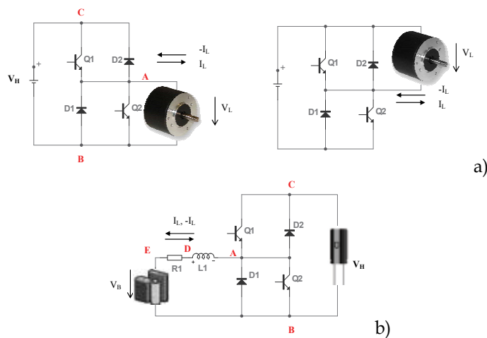
Fig. 7. Two-quadrant convertrs (I-Q, II-Q)
