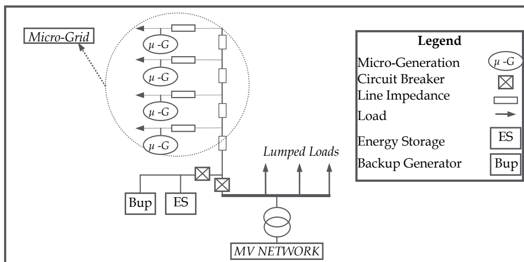
Fig. 1. Case study micro-grid
