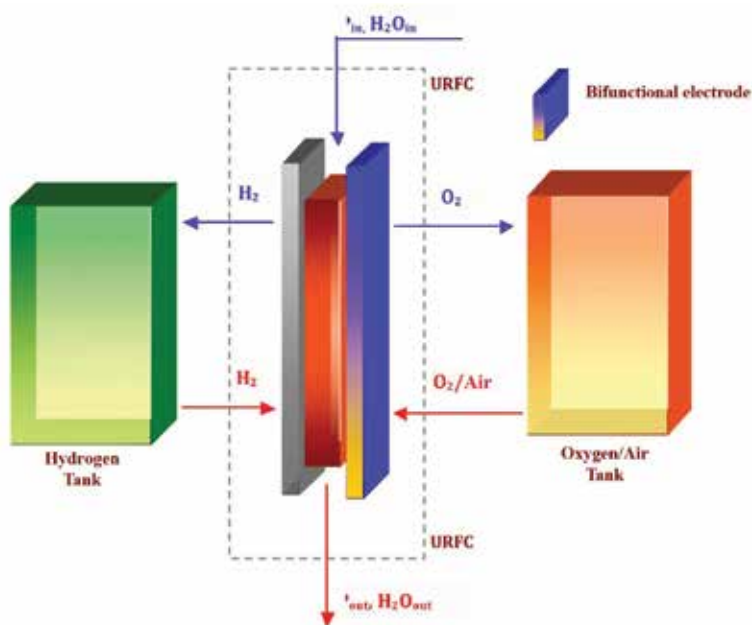
Fig. 7. Unitized regenerative fuel cell outline
