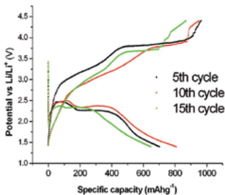
Fig. 11. The charge-discharge curves of Poly(tetrahydrobenzodithiophene) PTKP
