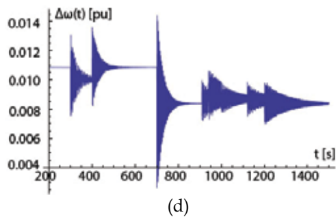
Figs. 18c,d. (c) Transient response \Delta\omega(t) if storage plants 4 and 6 absorb the additional energy generated by WP plant with 0.2 s delay; (d) Transient response \Delta\omega(t) if only storage plant 6 absorbs the additional energy generated by WP plant with 0.2 s delay.
