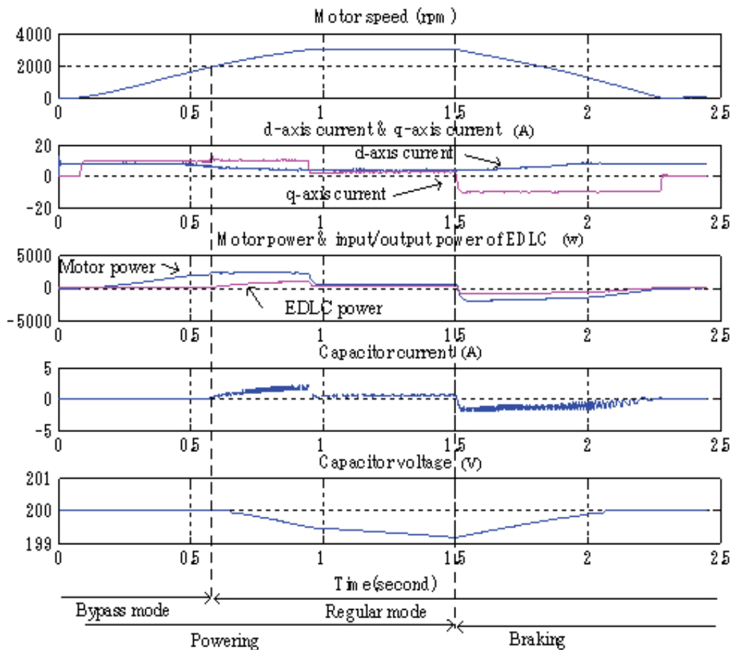
Fig. 8. Simulation wave forms at conventional operating pattern
