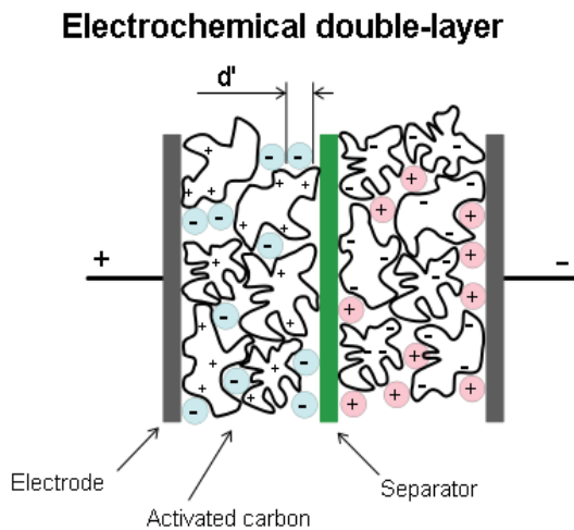
Fig. 17. Principle of supercapacitor (EPCOS AG, 2011)
