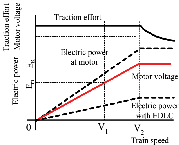
Fig. 4. Traction effort, power and voltage vs. speed characteristics in the system of increased current method
