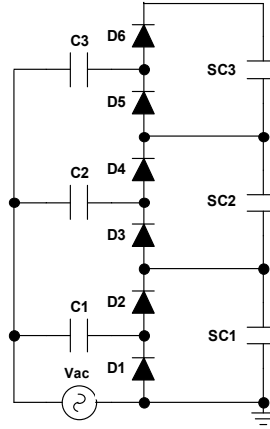
Fig. 6. Switchless cell/module voltage equalizer.
