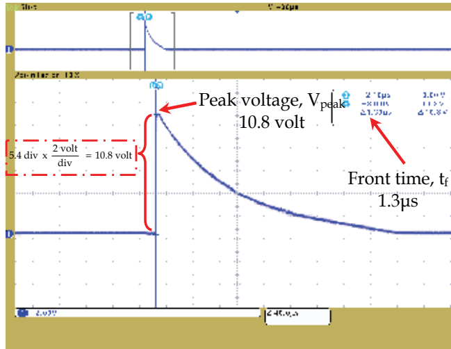
Fig. 15. Front time t_f of the experimental impulse voltage wave shape
