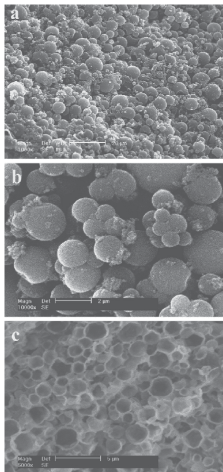
Fig. 18. SEM morphologies of treated and dried microcapsules: (a) piled microPCMs, (b) smooth and the regular global shape with a diameter of about 5–10 \mu\text{m} and (c) a typical cross-sectional morphology of shells.
