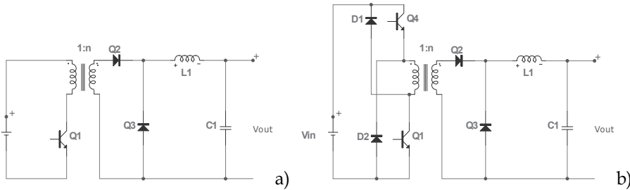
Fig. 14. Buck-derived dc-to-dc converters with transformer isolation (Forward)
