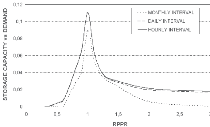
Fig. 9. Critical Storage Curve for different sampling times
