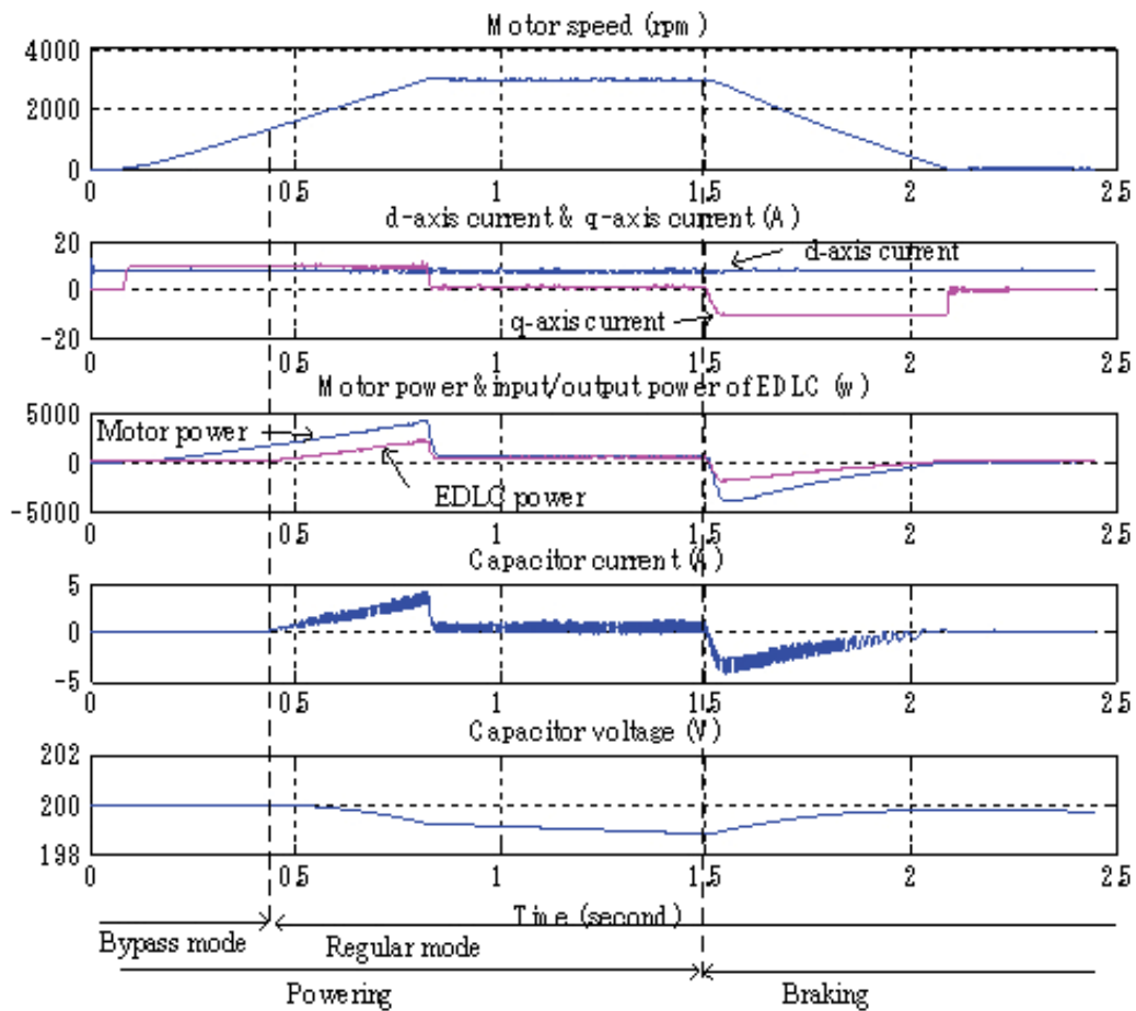
Fig. 10. Simulation wave forms in the new system of increased power with energy storage device
