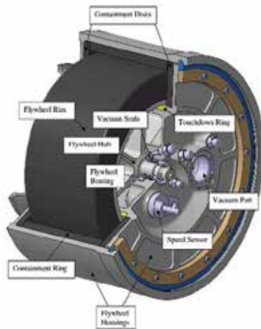
Fig. 30. Flywheel construction (Flybrid Systems, 2010)
