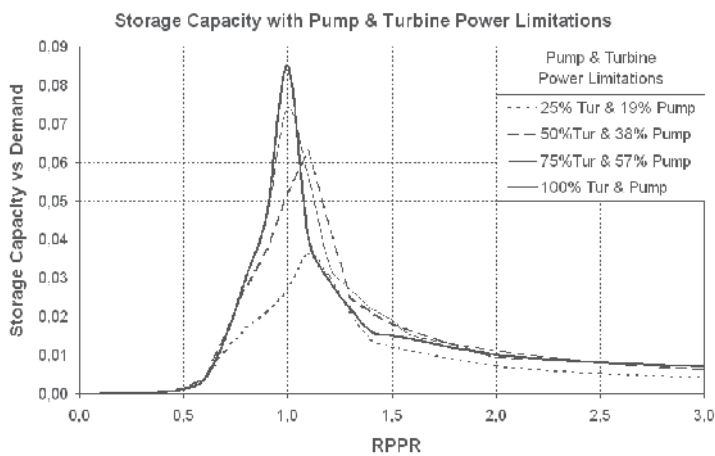
Fig. 11. Influence of storage drives limit power.
