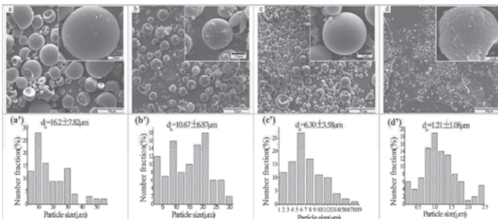
Fig. 14. SEM morphologies (a-d) and diameter number fractions (a'-d') of microPCMs fabricated with different stirring rates ( 1000, 2000, 3000 and 4000 \text{ r min}^{-1} ; C_t=50\% ).
