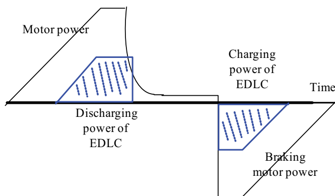
Fig. 18. Total motor power & charging/discharging power of EDLC
