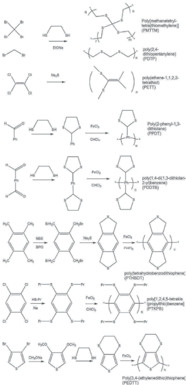
Scheme 2. Structure and Synthesis Routes of thioether polymers
