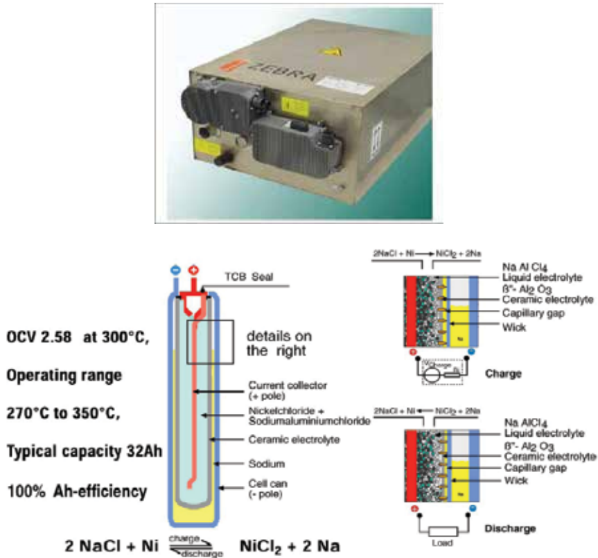
Fig. 5. Zebra battery
