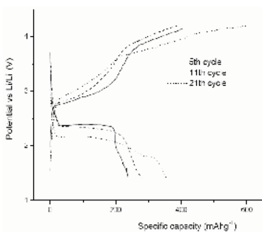
Fig. 9. Charge-discharge curves of poly(1,4-di(1,3-dithiolan-2-yl)benzene) PDDTB
