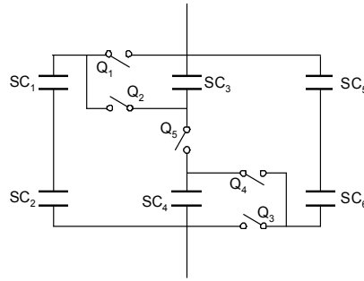
Fig. 14. Reconfigurable series-parallel SC energy storage unit.
