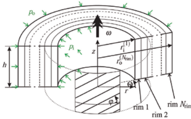
Fig. 5. Multi-rim setup of the flywheel rotor
