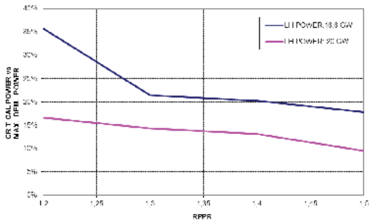
Fig. 17. Critical Power for baseline case depending on large hydro power.
