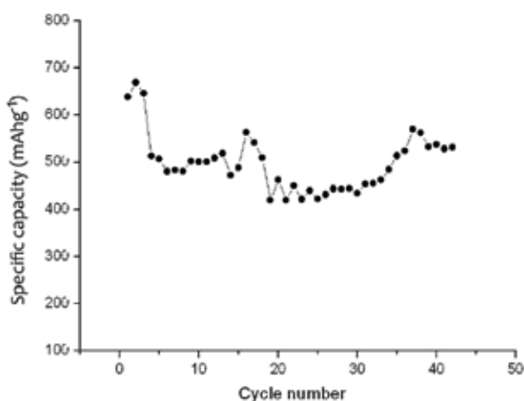
Fig. 6. Specific capacity of poly[3,4-(ethylenedithio)thiophene]
