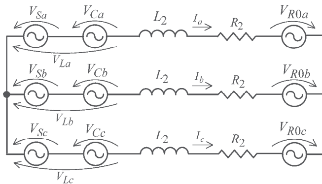
Fig. 3. Three phase equivalent circuit of matrix UPFC and transmission line.
