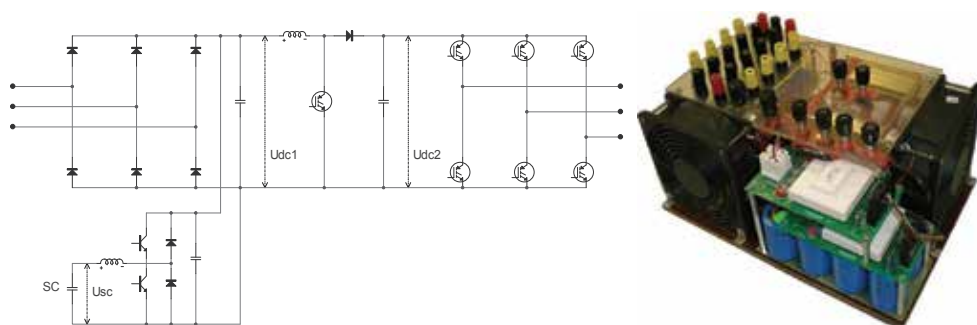
Fig. 27. Concepts of bi-directional converters with supercapacitors
