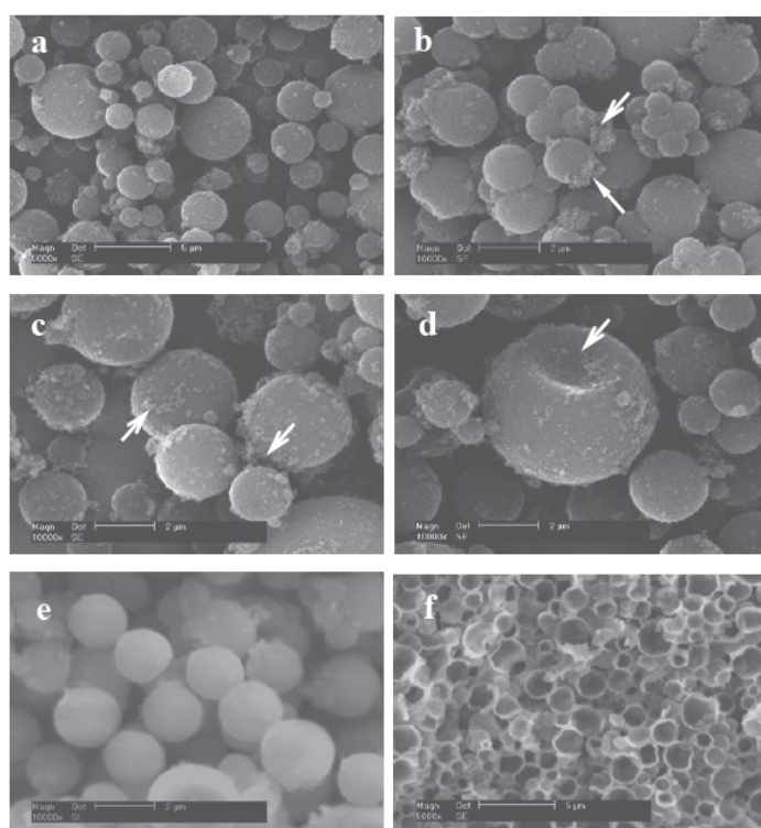
Fig. 3. SEM photographs of microcapsules dried in a vacuum oven at 40\ ^\circ\text{C} for 24 h, (a) (b) surface morphology of piled OSC microcapsules, (c) (d) the rough surface morphology of OSC microcapsules, (e) surface morphology of piled TSC microcapsules, (f) cross section of TSC microcapsules.
