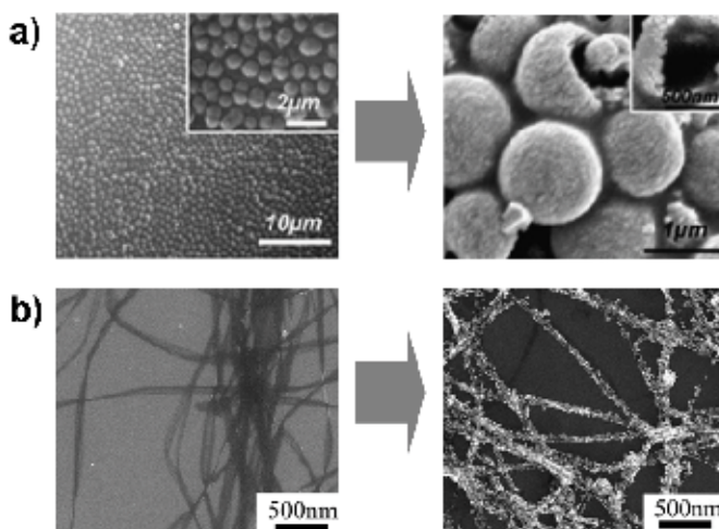
Fig. 3. Nanomaterials fabricated using biomaterials as structural templates: (a) Str. thermophilus (left) and ZnO hollow nanospheres fabricated using Str. thermophilus as the structural template (right) (Zhou et al., 2007) and (b) bacteria-cellulose nanofibers (left) and Au-bacterial-cellulose nanocomposite (right) (Zhang et al., 2010).
