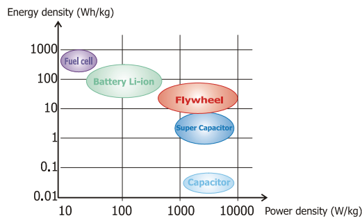
Fig. 3. Comparison of several ESS due to energy and power density
