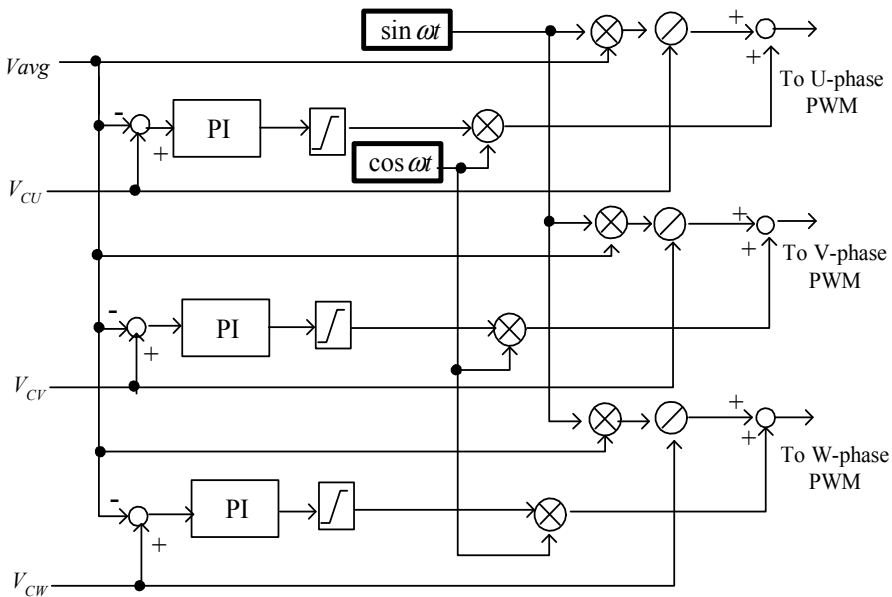
Fig. 16. Block diagram of balancing control
