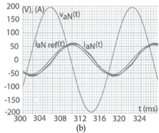
Figs. 13a,b. Inverter phase reference current, inverter phase output current, and power system phase voltage (about the same as inverter output voltage), see Fig.12a and Table 5; (a) \Phi = 30^\circ (generator notation: leading power factor, underexcited, absorbing reactive power from grid); (b) \Phi = -90^\circ (generator notation: lagging power factor, overexcited, delivering reactive power to grid)
