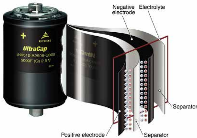
Fig. 18. Typical structure (layers) of supercapacitor (EPCOS AG, 2011)
