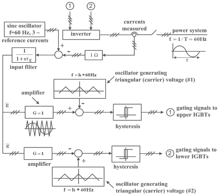
Fig. 12b. Block diagram of control circuit for current-controlled, PWM voltage-source inverter based on P-control
