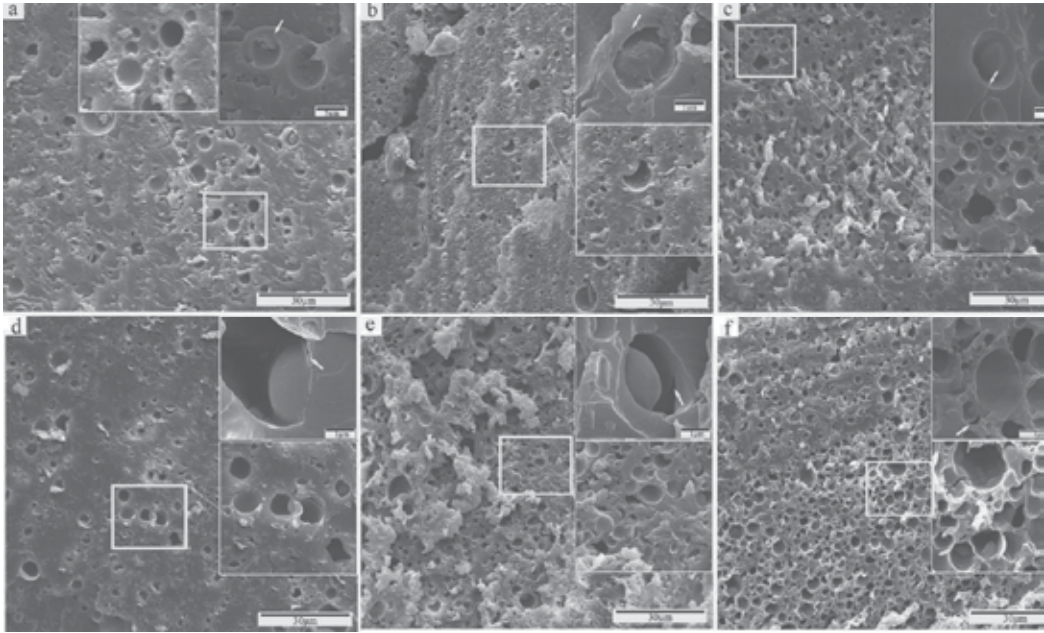
Fig. 16. SEM morphologies of microPCMs/epoxy composites (microPCMs/E-51, wt/wt)=1/1) before (a, b, c) and after (d, e, f) a thermal treatment process with different C_t (%) values: (a) 40%, (b) 50%, (c) 60%.
