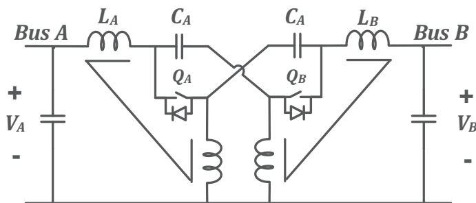
Fig. 4. A different structure for NBDC
