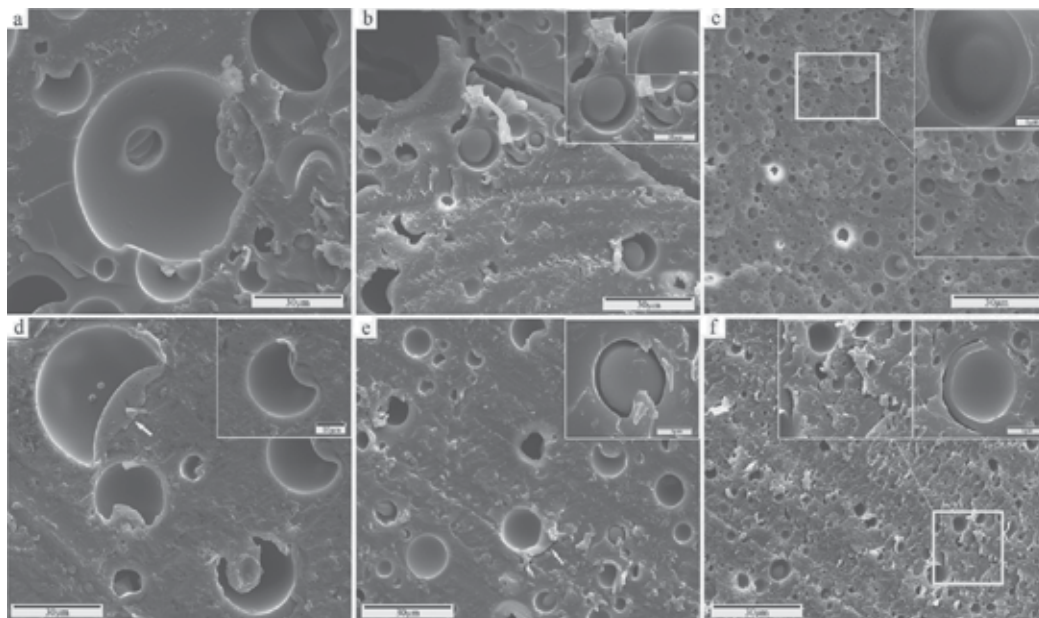
Fig. 17. SEM morphologies of microPCMs/epoxy composites (MicroPCMs/E-51, wt/wt=1/1; C_t=50\% ) before (a, b, c) and after (d, e, f) thermal treatment containing microPCMs prepared by different emulsion rates: (a, d) 1000 \text{ r min}^{-1} , d_n=16 , 20\pm 7.82 \mu\text{m} ; (b, e) 2000 \text{ r min}^{-1} , d_n=10 , 67\pm 6.82 \mu\text{m} ; (c, f) 3000 \text{ r min}^{-1} , d_n=6 , 30\pm 3.58 \mu\text{m} .
