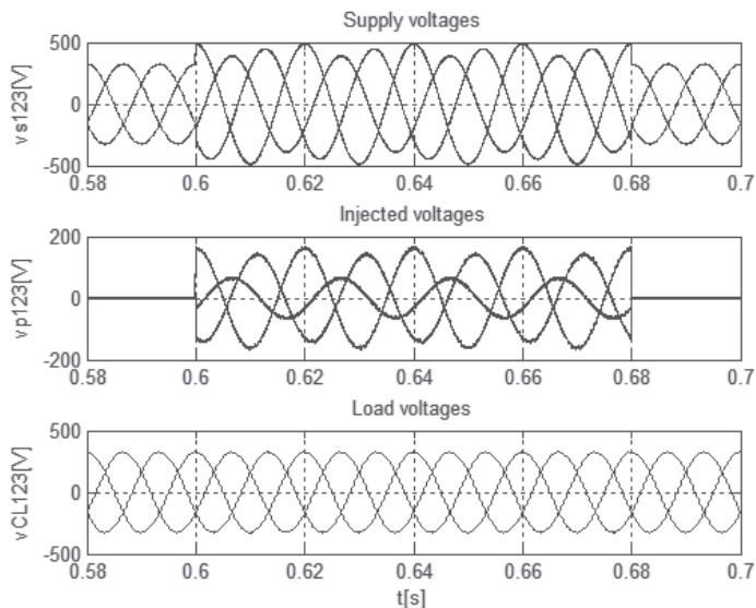
Fig. 17. Simulation result of DVR response to unbalanced voltage swell: Supply voltages ( v_1, v_2, v_3 ), Injected voltage ( v_{p1}, v_{p2}, v_{p3} ) and load voltage ( v_{CL1}, v_{CL2}, v_{CL3} ).
