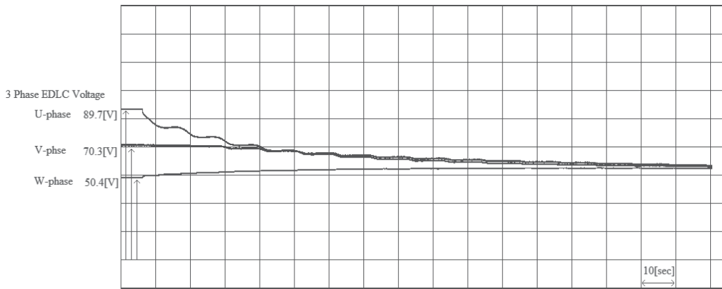
Fig. 17. Experimental results of balancing control
