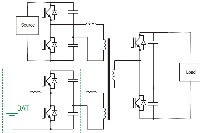
Fig. 13. Traction topology of ESS based on supercapacitors - high voltage version
