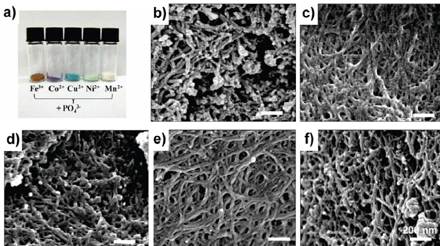
Fig. 23. (a) Photographs and (b-f) SEM images of various peptide-metal phosphate hybrid materials: injected metal ions are (b) \text{Fe}^{3+} , (c) \text{Co}^{2+} , (d) \text{Cu}^{2+} , (e) \text{Ni}^{2+} and (f) \text{Mn}^{2+} ions, respectively. (Ryu et al., 2010a).
