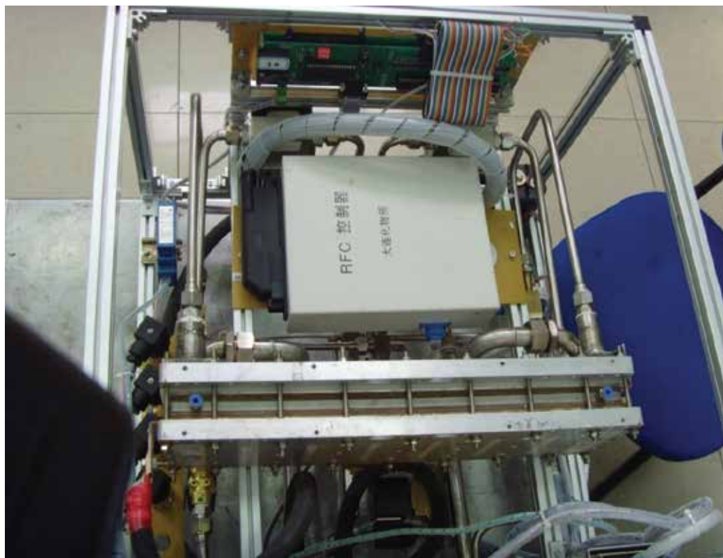
Fig. 11. Assembled high temperature PEMFCs system
