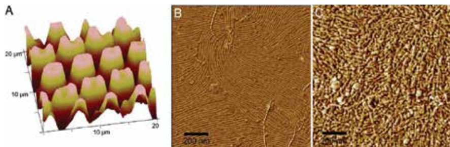
Fig. 12. AFM images of the virus-based microbattery: (a) height image of stacks of the virus- \text{Co}_3\text{O}_4 /(LPEI/PAA) multilayer/PDMS electrode, and phase image of the virus assembly onto the multilayer (b) before and (c) after the nucleation of \text{Co}_3\text{O}_4 (Nam et al., 2008).
