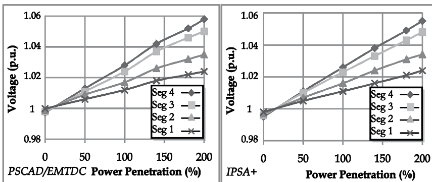
Fig. 2. Steady state voltage measurements at each LV segment during minimum load conditions
