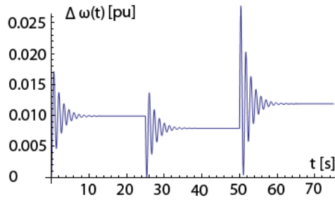
Fig. 3b. Angular frequency change \Delta\omega(t) for a positive load-step at time t=25 s and a negative load step at time t=50 s
