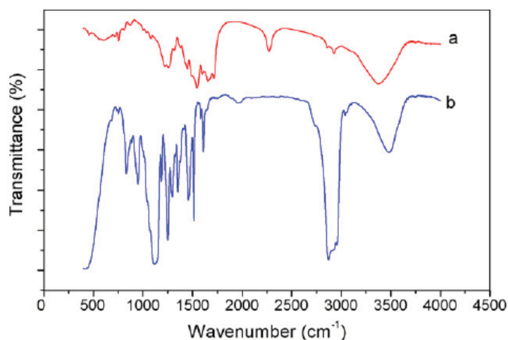
Fig. 19. FTIR curves of (a) liquid core material in shells and (b) shell material.
