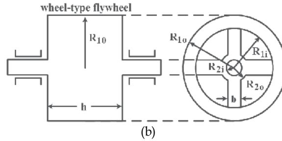
Fig. 15b. Flywheel power plant.
