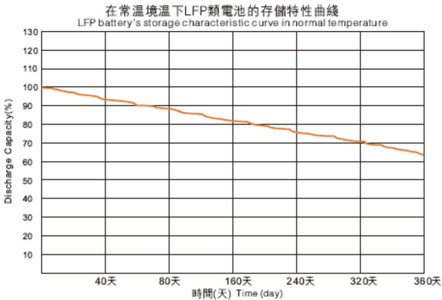
Fig. 10. Battery self discharge behaviour ( \text{LiFeYPO}_4 ) (Winston Battery Limited, n.d.)
