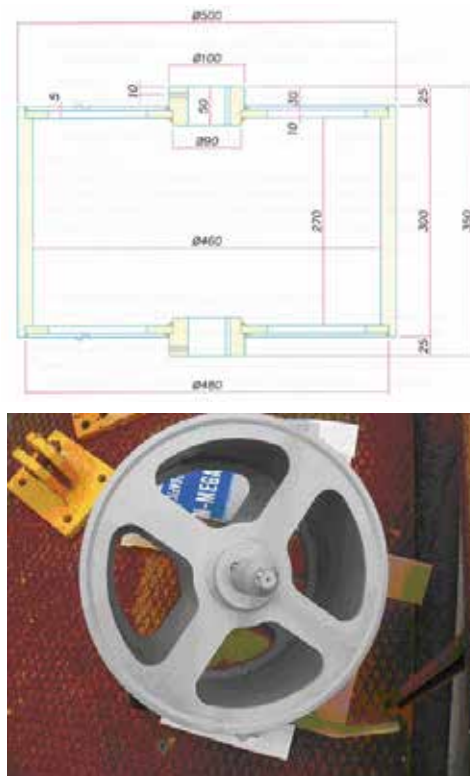
Fig. 8. Dimension and view of the steel barrel.
