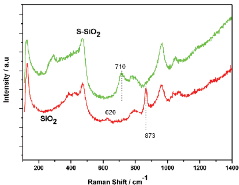
Fig. 2. UV Raman spectra of sol-gel derived SiO 2 and the sulfonated S- SiO 2 . (Ke, Li, et al., 2011)
