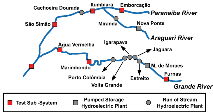
Fig. 1. Hydroelectric System Used.
