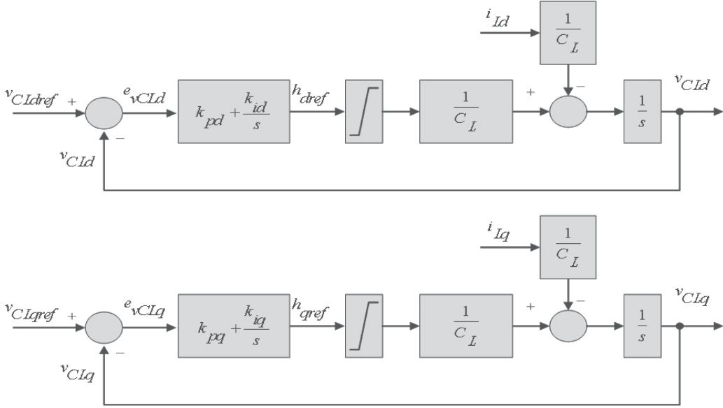
Fig. 3. Block diagram of the voltage components v_{CLd} and v_{CLq} .
