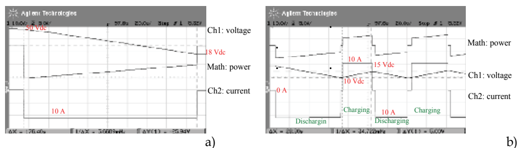
Fig. 28. Charging and discharging of supercapacitor (BMOD0083E48)
