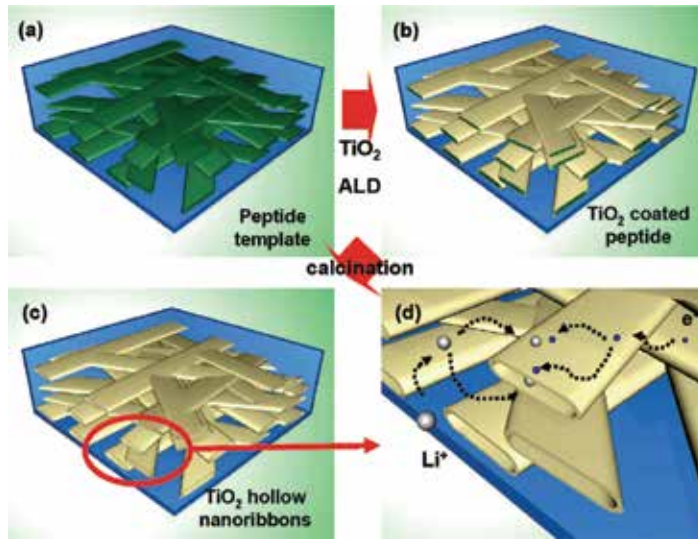
Fig. 19. Schematic illustration of the synthesis process for a network structure of \text{TiO}_2 nanotubes based on peptide assembly and ALD: (a) peptide network template, (b) \text{TiO}_2 coated peptide network by ALD, (c) \text{TiO}_2 nanotube network after removing the peptide template, and (d) \text{Li} -ion and electron transports expected in \text{TiO}_2 nanotube network structure (Kim et al., 2009).
