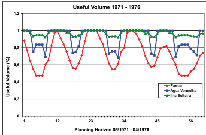
Fig. 10. Trajectories of Volume of some Reservoirs (1971 - 1976).
