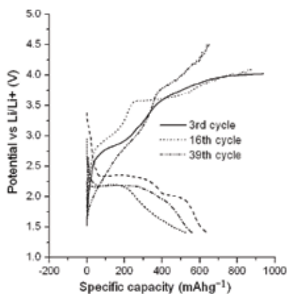
Fig. 12. Charge-discharge curves of Poly[3,4-(ethylenedithio)thiophene] PEDTT
