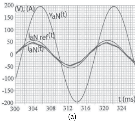
Figs. 13a,b. Inverter phase reference current, inverter phase output current, and power system phase voltage (about the same as inverter output voltage), see Fig.12a and Table 5; (a) \Phi = 30^\circ (generator notation: leading power factor, underexcited, absorbing reactive power from grid); (b) \Phi = -90^\circ (generator notation: lagging power factor, overexcited, delivering reactive power to grid)
