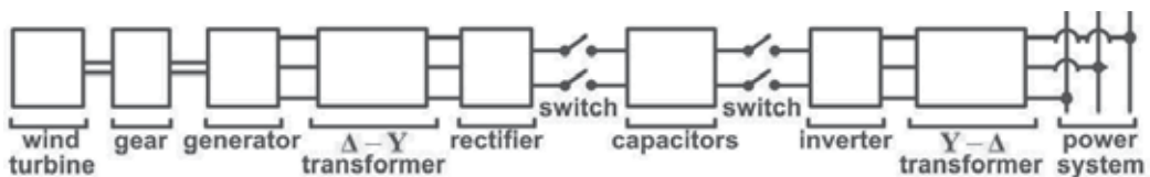
Fig. 14. Block diagram for charging and discharging supercapacitor bank
