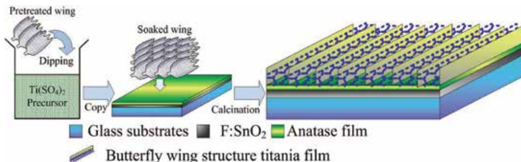
Fig. 27. Schematic diagram of the fabrication of a TiO 2 photo-anode based on butterfly-wing assembly (Zhang et al., 2009).
