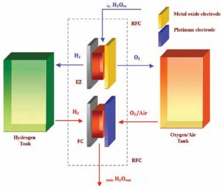
Fig. 6. Regenerative fuel cell (RFC) outline
