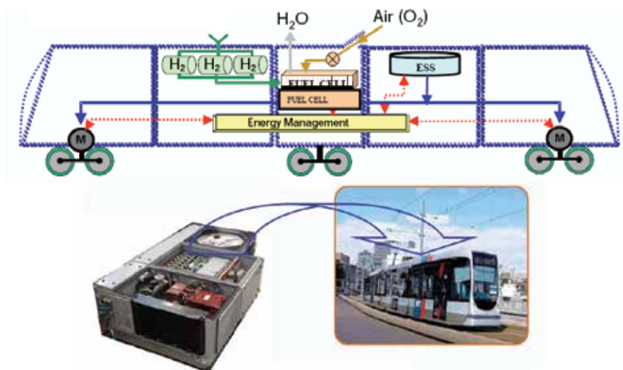
Fig. 34. Hydrogen train (ALSTOM, 2011)
