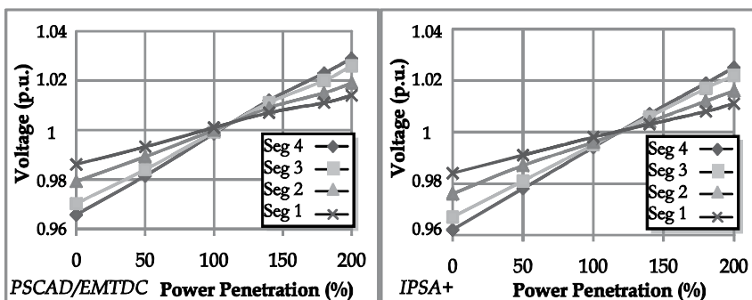
Fig. 3. Steady state voltage measurements at each LV segment during maximum load conditions
