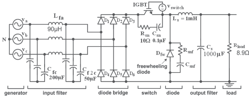
Fig. 10. Controlled three-phase rectifier with self-commutated switch
