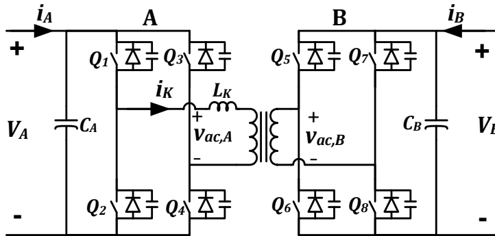
Fig. 6. Circuit diagram of Configuration 1.
