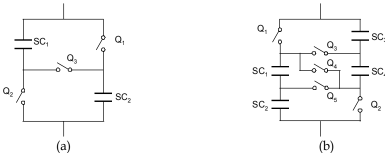
Fig. 13. Conventional reconfiguration techniques using (a) series-parallel and (b) shift-type changeover circuits.
