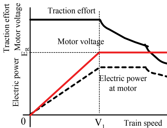
Fig. 3. Traction effort, power and voltage vs. speed characteristics in conventional systems
