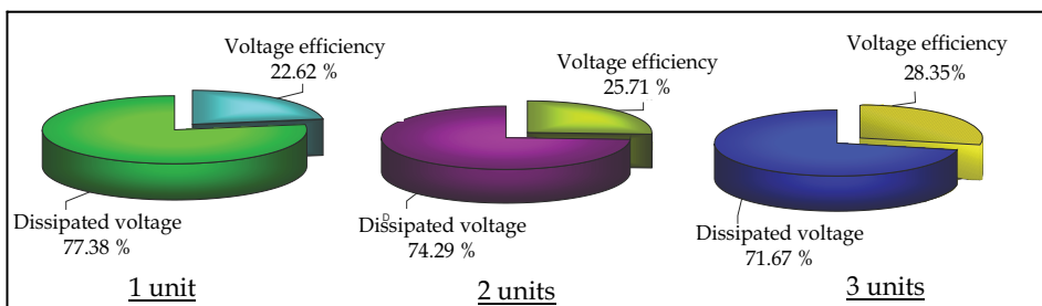
Fig. 20. Pie chart for sample capacitor 0.22 \mu F (KNU 1910)
