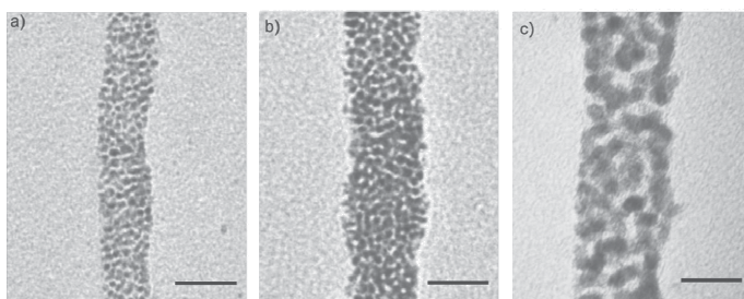
Fig. 30. TEM images of Pt-TMV hybrid nanowires prepared at various Pt precursor concentration. The concentrations increases from (a) through (c). (Scale bar: 20 nm) (Górzny et al., 2010).
