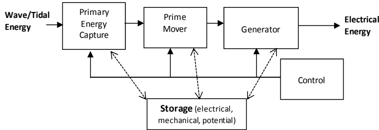
Fig. 4. Typical Ocean Energy Conversion Process
