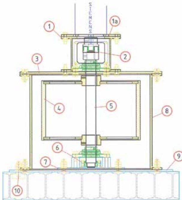
Fig. 9. Flywheel energy storage prototype.
