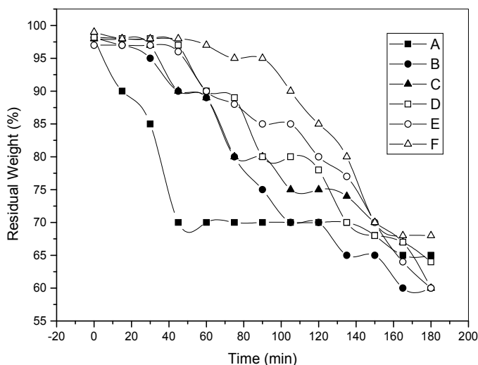
Fig. 8. Curves of the percentage residual weight (%) of core material in microcapsules in extraction solvent. The systems correspond to the conditions of coacervation methods and prepolymer dropping speed: A (■) OSC, 2.0 ml·min -1 ; B (●) OSC, 1.0 ml·min -1 ; C (▲) OSC, 0.5 ml·min -1 ; D (□) TSC, 2.0 ml·min -1 ; E (○) TSC, 1.0 ml·min -1 and F (△) TSC, 0.5 ml·min -1 .
