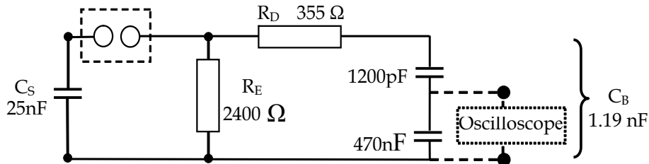
Fig. 14. Circuit diagram for stage 1 testing
