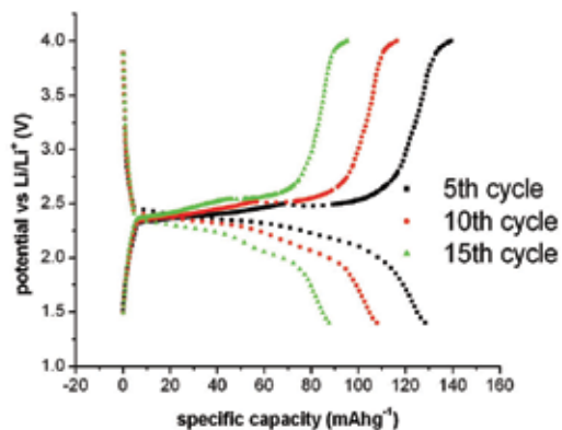
Fig. 10. Charge-discharge curves of poly[1,2,4,5-tetrakis(propylthio)benzene] PTKPB
