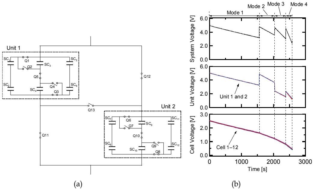
Fig. 16. (a) Reconfigurable series-parallel SC energy storage system and (b) resultant discharging curves of system, unit and cell voltages.
