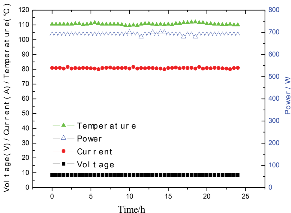
Fig. 12. Stabilization testing of the high temperature PEMFCs (H 2 /O 2 )
