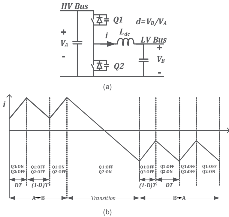
Fig. 2. (a) Basic NBDC and (b) operating waveforms.
