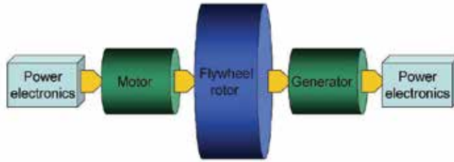
Fig. 4. Schematic showing power flow in FES system
