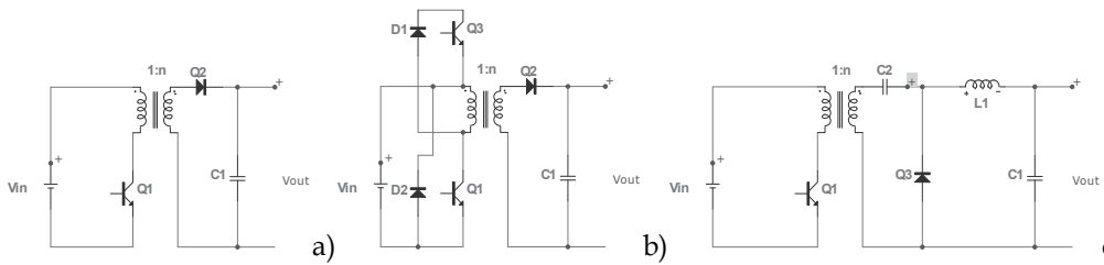
Fig. 17. Buck-Boost derived dc-to-dc converters with transformer isolation (Flyback) a) basic; b) two transistor Flyback; c) ZETA converter
