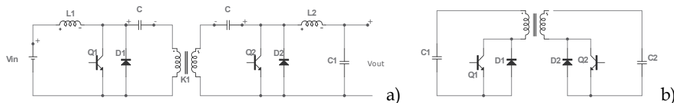
Fig. 22. Bi-directional form of a) Cúk dc-to-dc converter with transformer (Aboulnaga & Emadi, 2004); b) Bi-directional form of Flyback
