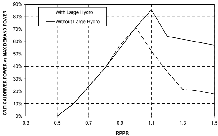
Fig. 15. Critical Power Drives for baseline case.
