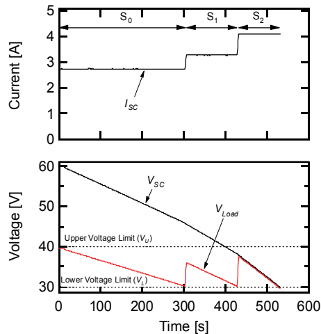
Fig. 12. Experimental discharge curves of the SC module with the prototype discharger using cascaded switched capacitor converters with selectable intermediate taps.
