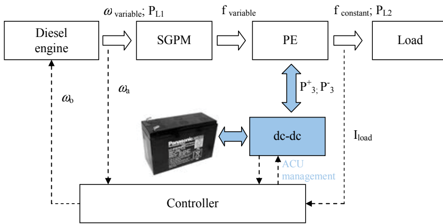
Fig. 3. The bi-directional dc-dc converters
