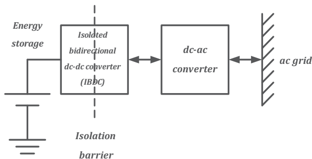
Fig. 13. Basic structure of an energy storage device connected to an ac grid with high frequency isolation barrier inside IBDC.
