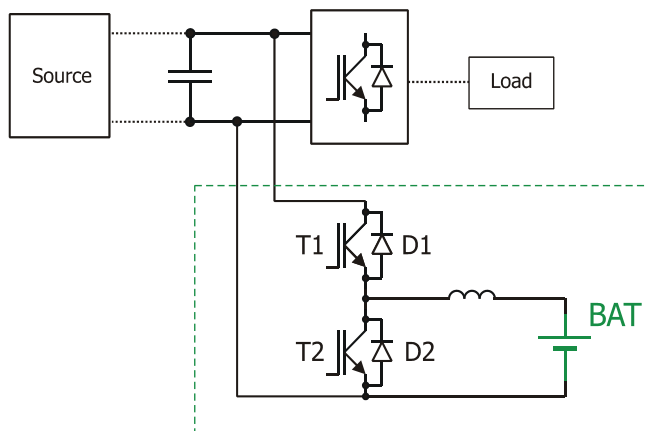
Fig. 11. The basic power circuit for ESS based on battery (standard buck/boost converter)
