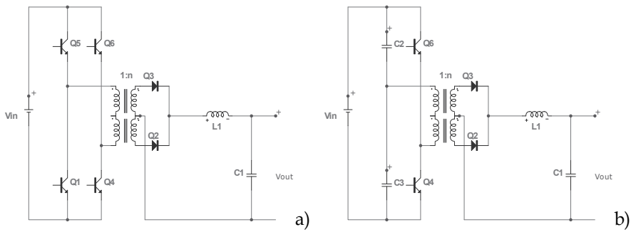
Fig. 16. Dc-to-dc converters with transformer isolation a) Full-bridge; b) Half-bridge
