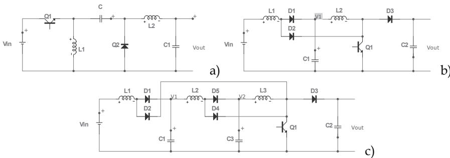
Fig. 13. Developed dc-to-dc converter a) positive Luo-converter; b) Two-stage Boost; c) Three-stage Boost (Luo & Ye, 2000).
