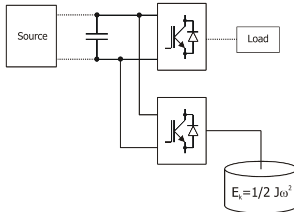
Fig. 27. Flywheel energy storage done electrically
