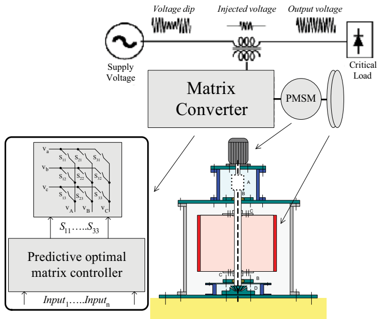
Fig. 1. Schematic diagram of a typical DVR.
