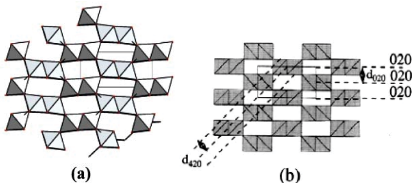
Fig. 3. a. The structure of \gamma - MnO_2 with irregular intergrowth of ( 1 \times 1 ) tunnels (pyrolusite) and ( 1 \times 2 ) tunnels (ramsdellite), b, ramsdellite- MnO_2 (Johnson et al., 1997; Devaraj & Munichandraiah, 2008).
