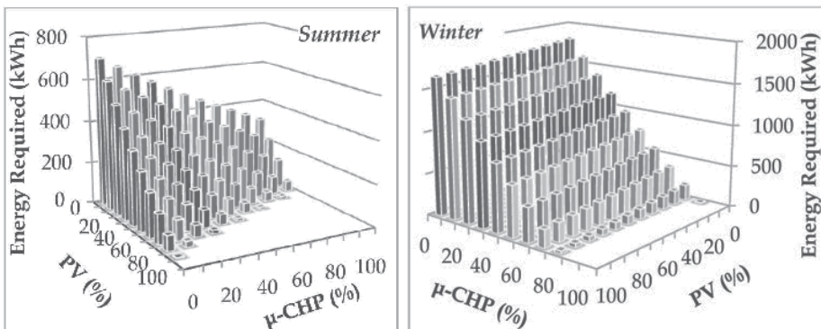
Fig. 13. Backup generator energy requirements for different penetration levels of micro-generation
