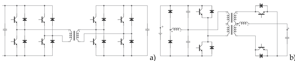
Fig. 21. a) Dual Full-bridge topology; b) Bi-directional dc-to-dc converter of half-bridge + current fed push-pull (Jain et al., 2000)
