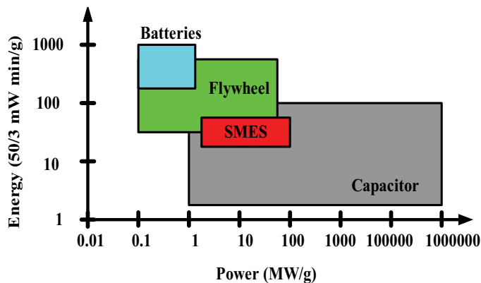
Fig. 3. Specific power versus specific energy ranges
