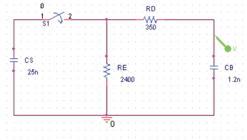
Fig. 9. Single stage impulse voltage generator simulation circuit
