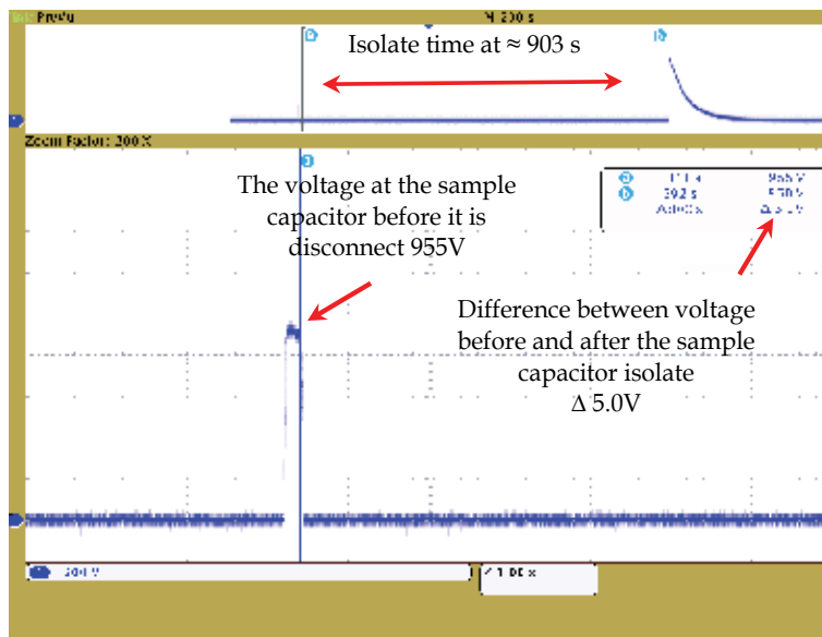
Fig. 24. The capacitor 0.22\mu\text{F} is isolated for 903 second after the switch opens
