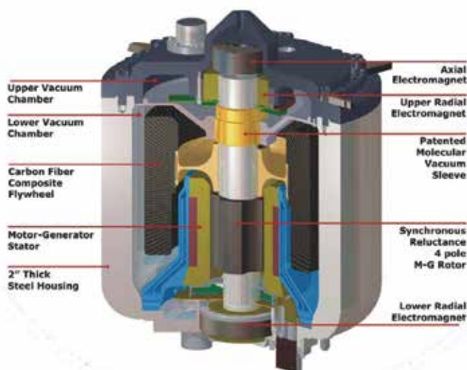
Fig. 1. Example of a commercial flywheel energy storage system (courtesy of POWERTHRU, Livonia, MI, USA - www.power-thru.com )
