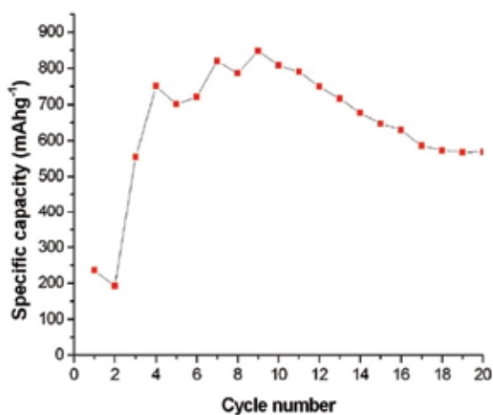
Fig. 5. Specific capacity ( \text{mAhg}^{-1} ) of poly(tetrahydrobenzodithiophene) vs. cycle numbers.
