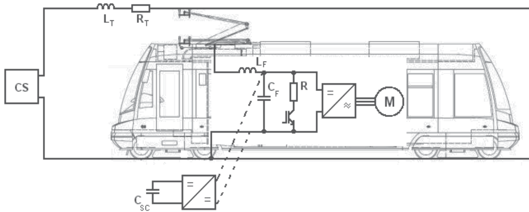
Fig. 24. Topology of energy storage system in light rail vehicle
