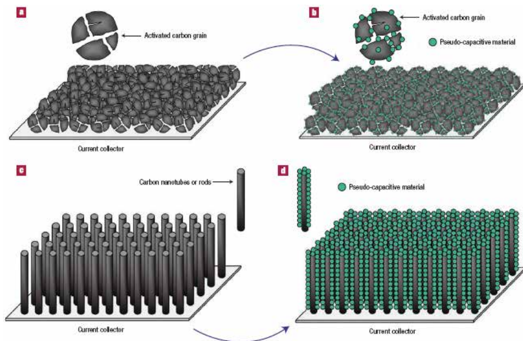
Fig. 11. Possible strategies to enhance energy and specific power of electrochemical capacitors: a, b) decoration of active carbon grains (a) with pseudo capacitive materials (b). c, d) attainment of a uniform deposit of pseudo-capacitive material (d) on high ordered, high SSA CNT layer (c).
