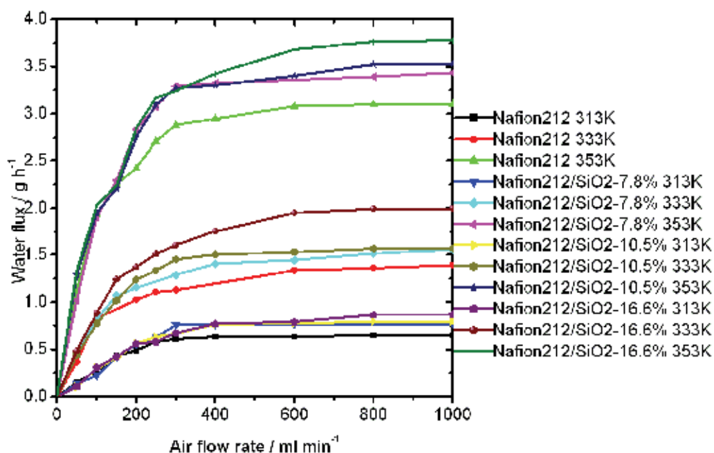
Fig. 6. Water flux of Nafion212/SiO 2 composite membrane with different content of SiO 2 as a function of the inlet gas flow rate of air at different operating temperatures. (Qu, Li, et al. , 2011)
