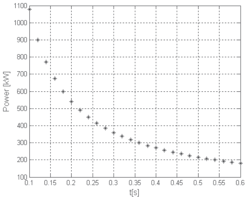
Fig. 10. Output power of the flywheel energy storage.
