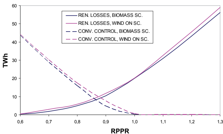
Fig. 25. Renewable energy losses and controllable conventional generation. Transition process.
