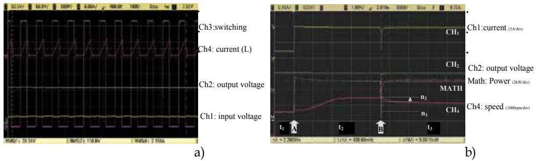
Fig. 29. a) The characteristic of Bi-directional converter with supercapacitor b) The verification of the EGS concept with supercapacitor and bi-directional converter
