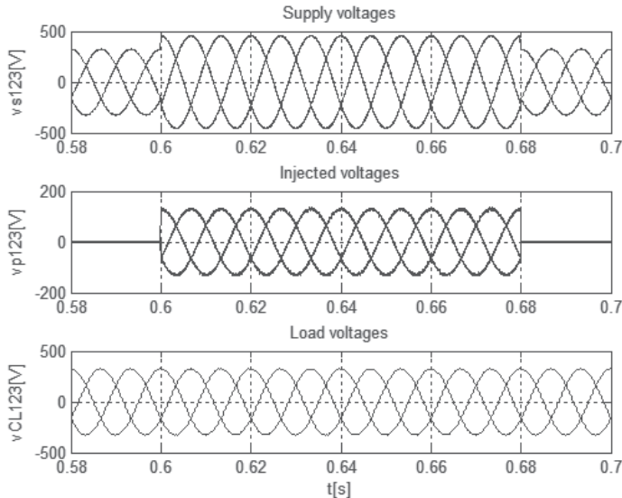
Fig. 16. Simulation result of DVR response to balanced voltage swell: Supply voltages ( v_1, v_2, v_3 ), Injected voltage ( v_{p1}, v_{p2}, v_{p3} ) and Load voltage ( v_{CL1}, v_{CL2}, v_{CL3} ).
