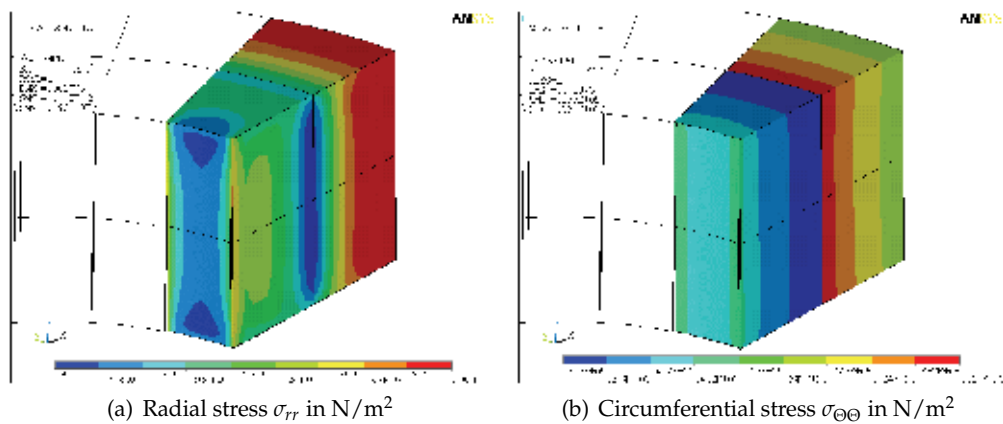
Fig. 6. Stress distributions in the finite element sector model for a rotational speed of n = 30000 \text{ min}^{-1}
