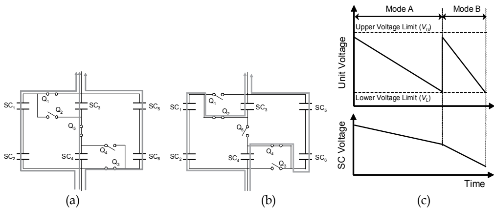
Fig. 15. Current flow directions in (a) mode A and (b) mode B, and (c) cell and unit voltage curves during discharging.
