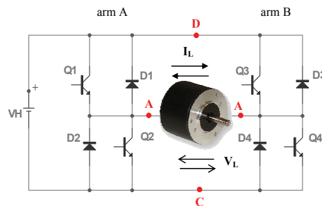
Fig. 9c. Four-quadrant dc-to-dc converter (I-Q, II-Q, III-Q, IV-Q).
