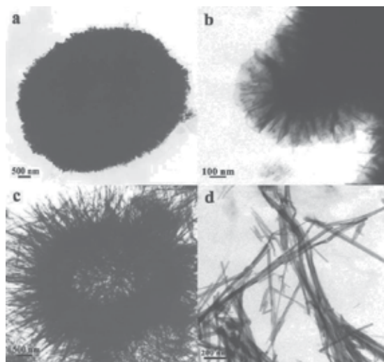
Fig. 8. TEM of \alpha -MnO 2 obtained at 110 °C for different reaction time (a, 3 h; b, 6 h; c, 12 h; d, 24 h).
