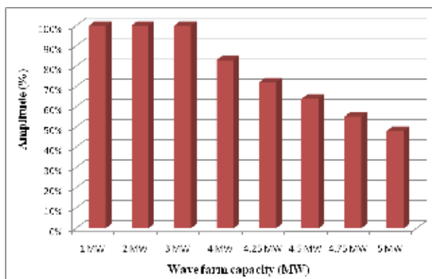
Fig. 14. Maximum allowed power fluctuation amplitude
