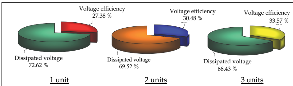
Fig. 22. Pie chart for sample capacitor 0.68µF (CBB20)
