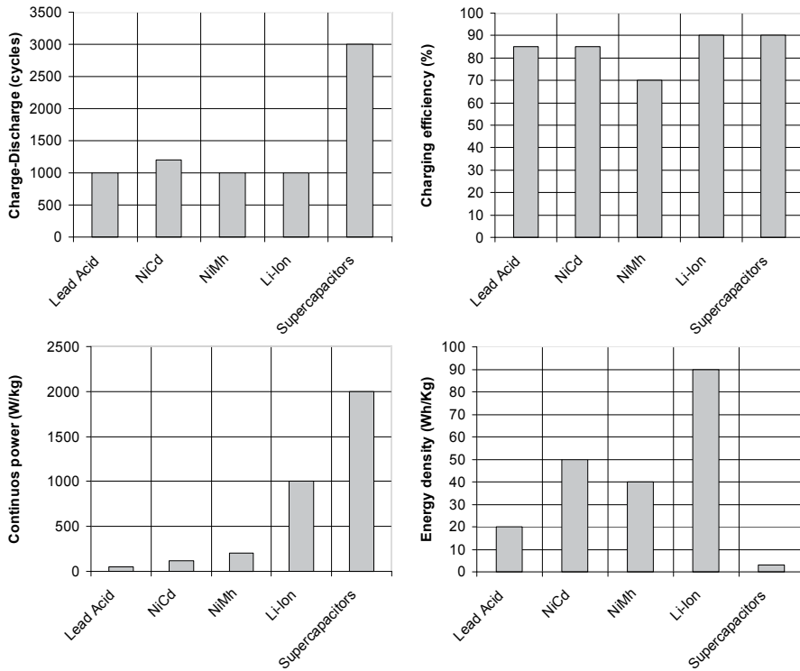
Fig. 25. Battery comparing (Leuchter et al., 2010)
