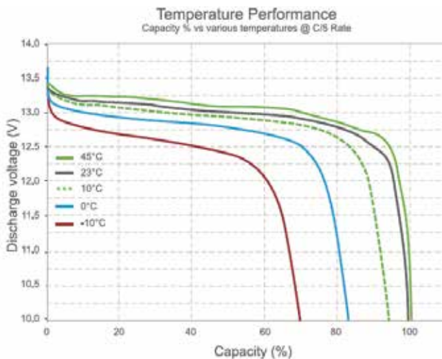
Fig. 7. Discharge Voltage depends on operating temperature ( \text{LiFeMgPO}_4 ) (Valence Technology, 2010)
