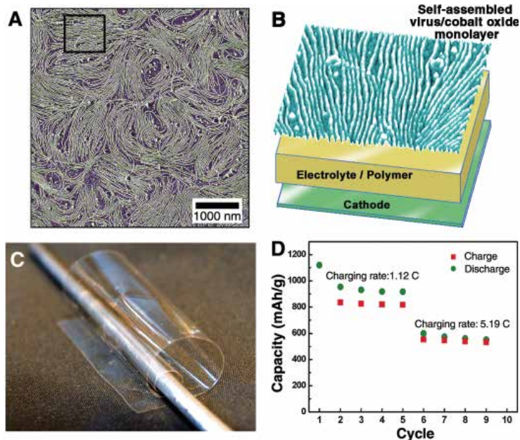
Fig. 14. Self-standing and flexible electrode film based on the virus- \text{Co}_3\text{O}_4 nanowires: (a-b) phase-mode AFM image of the virus- \text{Co}_3\text{O}_4 nanowires, (c) photograph of the electrode film composed of virus- \text{Co}_3\text{O}_4 on a LPEI/PAA multilayer with excellent flexibility, and (d) electrochemical property of the virus- \text{Co}_3\text{O}_4 anode at current rates of 1.12C and 5.19C. (Nam et al., 2006).
