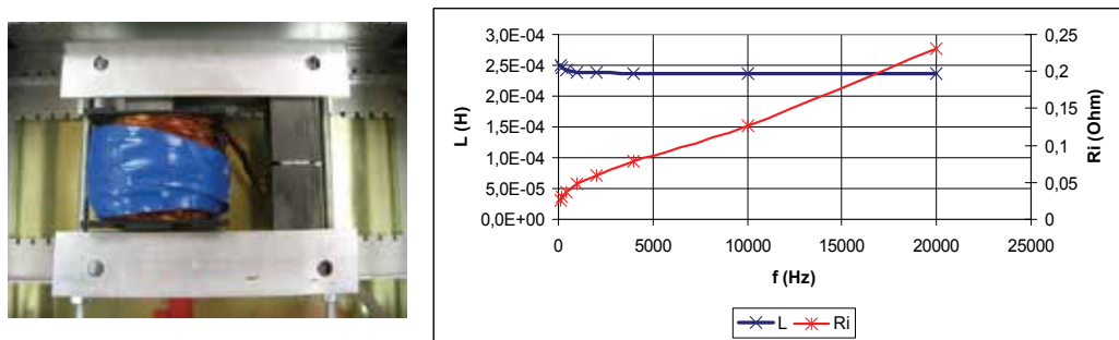
Fig. 30. Inductance versus frequency
