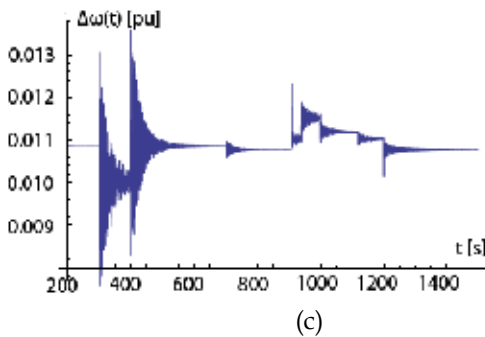
Figs. 18c,d. (c) Transient response \Delta\omega(t) if storage plants 4 and 6 absorb the additional energy generated by WP plant with 0.2 s delay; (d) Transient response \Delta\omega(t) if only storage plant 6 absorbs the additional energy generated by WP plant with 0.2 s delay.
