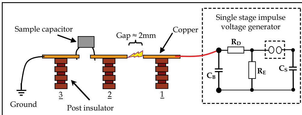
Fig. 17. Connection of sample capacitor with the impulse voltage generator.
