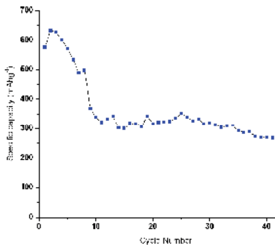
Fig. 2. Cycling capacity of Poly(ethene-1,1,2,2-tetrathiol) (PETT). Poly(ethene-1,1,2,2-tetrathiol) (PETT) displays a stable discharge specific capacity value of ca. 300 mAhg -1 from the 10th cycle to the 40th cycle and shows maximal specific capacity of 632 mAhg -1 at the second cycle. The coulomb efficiency is at high level of 90% from the 10th cycle to the 40th cycle. It shows more stable discharge specific capacity compare to saturate aliphatic thioether polymers; indicating vinyl structure benefits the electrode reaction.
