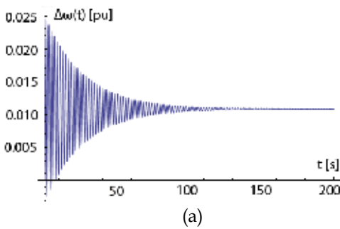
Figs. 18a,b. (a) Establishment of steady-state conditions for \Delta\omega(t) ; (b) Plot of given WP plant load reference Lr5[t]
