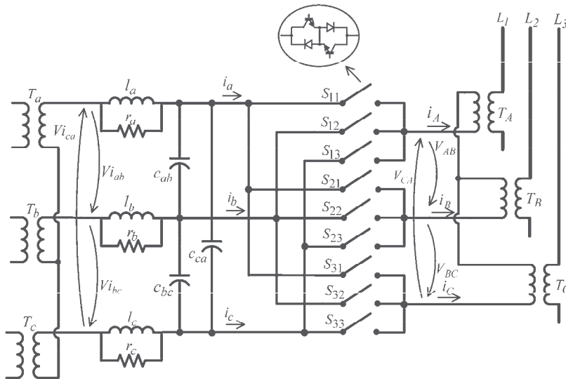
Fig. 2. Detailed matrix converter based UPFC.
