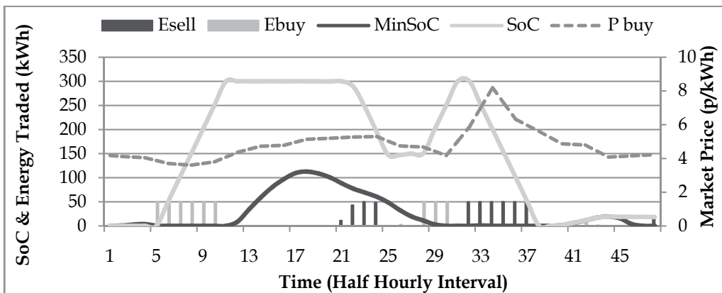
Fig. 15. Optimisation results for winter scenario
