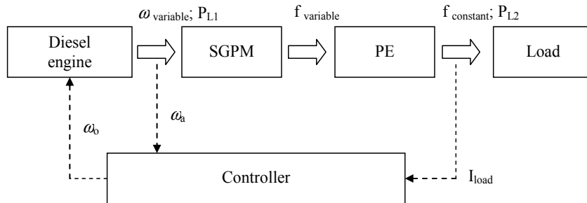
Fig. 1. Block diagram of EGS system with VSCF technology (SGPM-synchronous generator with PM; PE-power electronics)
