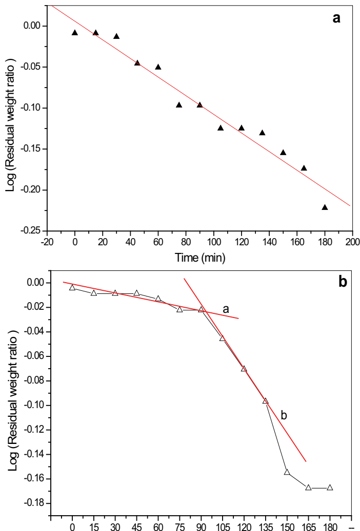
Fig. 9. The release curves of the OSC (a) and TSC (b) shells prepared by pre-polymer material dropping rates of 0.5 \text{ ml}\cdot\text{min}^{-1} .
