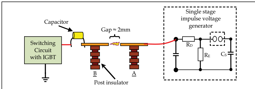
Fig. 23. IGBT switch is placed in series with the sample capacitors
