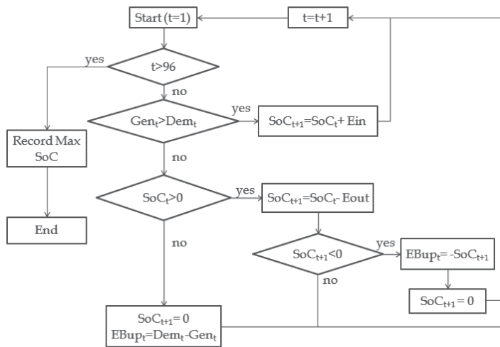
Fig. 10. Algorithm flow chart
