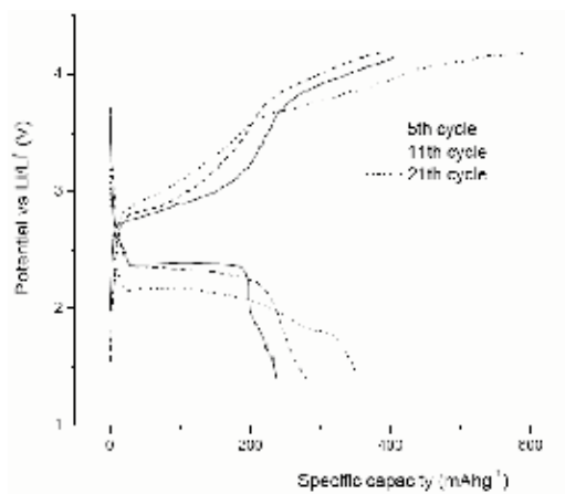
Fig. 8. The charge-discharge of poly(ethene-1,1,2,2-tetrathiol) PETT
