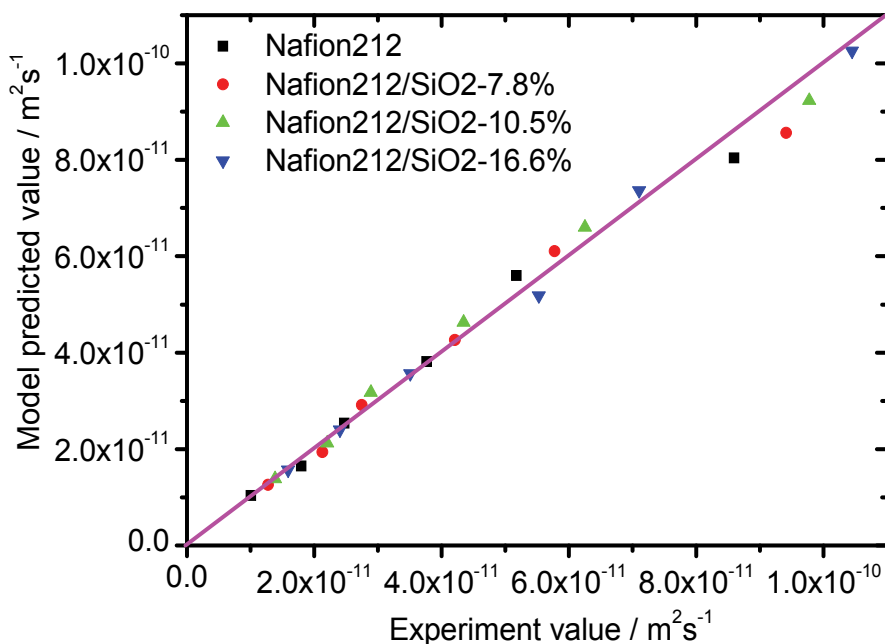
Fig. 9. Comparison of the empirical correlation predicted and experimental water apparent diffusion coefficient of composite membrane. (Qu, Li, et al. , 2011)
