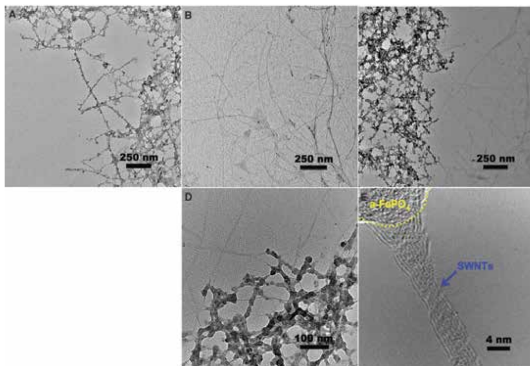
Fig. 8. Nanostructure of synthesized hybrid nanowires: (a) virus-amorphous \text{FePO}_4 hybrid nanowires without CNTs, (b) bare CNTs, and (c-e) virus-amorphous \text{FePO}_4 -CNT hybrid nanowires at different resolutions (Lee et al., 2009).
