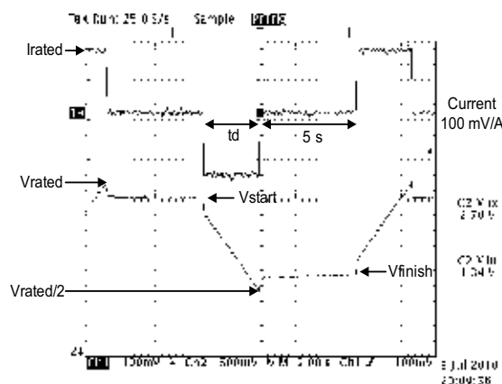
Fig. 18. SC current and voltage during characterisation
