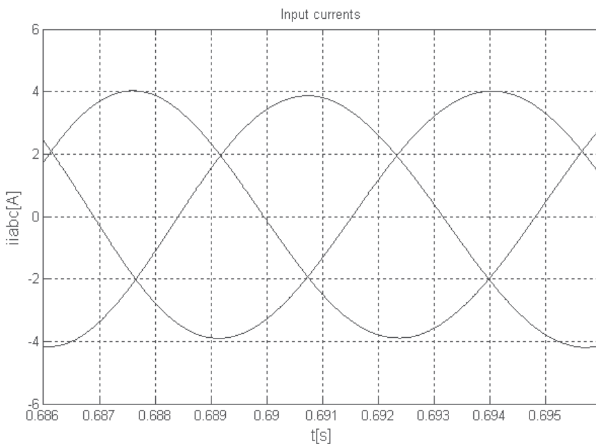
Fig. 18. Matrix input currents ( i_{ia}, i_{ib}, i_{ic} ).
