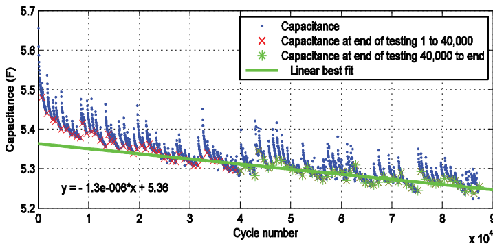
Fig. 22. Capacitance versus cycle number during application testing
