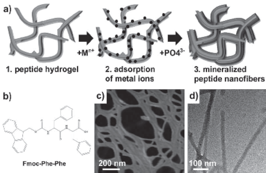
Fig. 22. Fabrication of peptide-amorphous \text{FePO}_4 hybrid material using the sequential injection method: (a) schematic diagram describing the fabrication process, (b) molecular structure of Fmoc-diphenylalanine, (c) SEM image and (d) TEM image of the peptide network (Ryu et al., 2010a).
