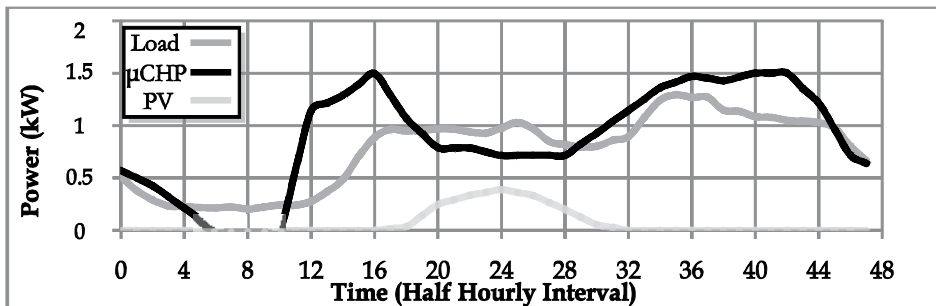
Fig. 5. Winter generation and demand profiles
