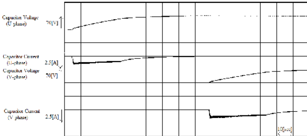
Fig. 15. Experimental results of initial charge operation
