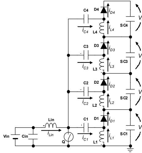
Fig. 3. Single-switch cell/module voltage equalizer using multi-stacked SEPICs.
