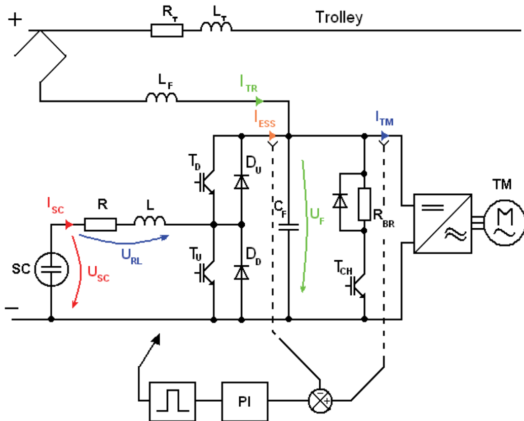
Fig. 25. Light rail topology - Buck (TD)/Boost (TU) convertor for SC
