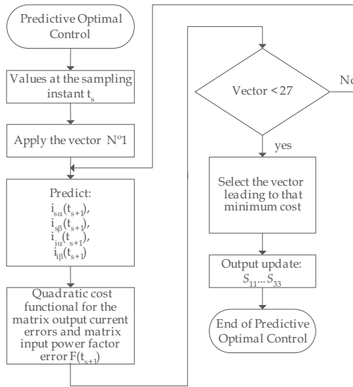
Fig. 6. Predictive Optimal Matrix Converter Control Algorithm.
