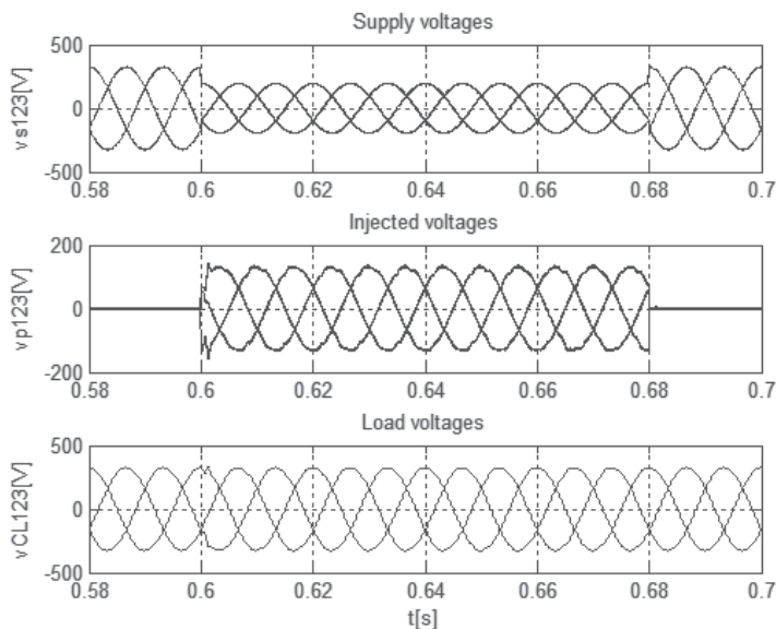
Fig. 14. Simulation result of DVR response to balanced voltage sag: Supply voltages ( v_1, v_2, v_3 ), Injected voltage ( v_{p1}, v_{p2}, v_{p3} ) and Load voltage ( v_{CL1}, v_{CL2}, v_{CL3} ).
