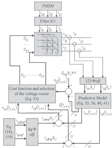
Fig. 7. Block diagram of the predictive optimal matrix converter control.
