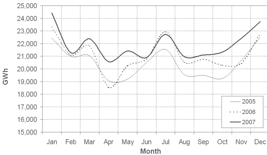
Fig. 2. Monthly demand in Spain (2005 – 2007)
