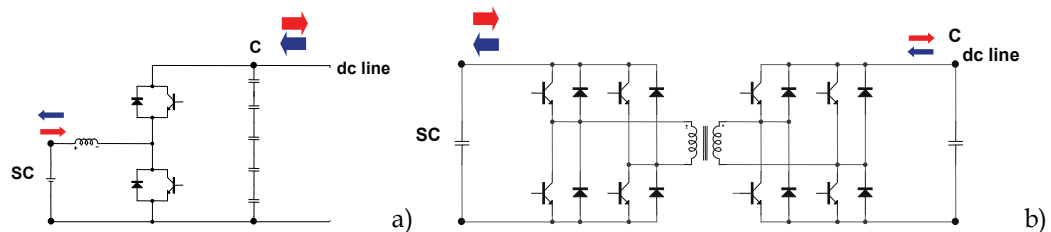
Fig. 26. Concepts of bi-directional converters with supercapacitors
