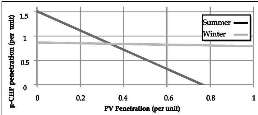
Fig. 7. Micro-generation penetration required to achieve the balance in the micro-grid
