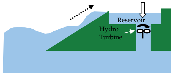
Fig. 10. Overtopping Device Illustration
