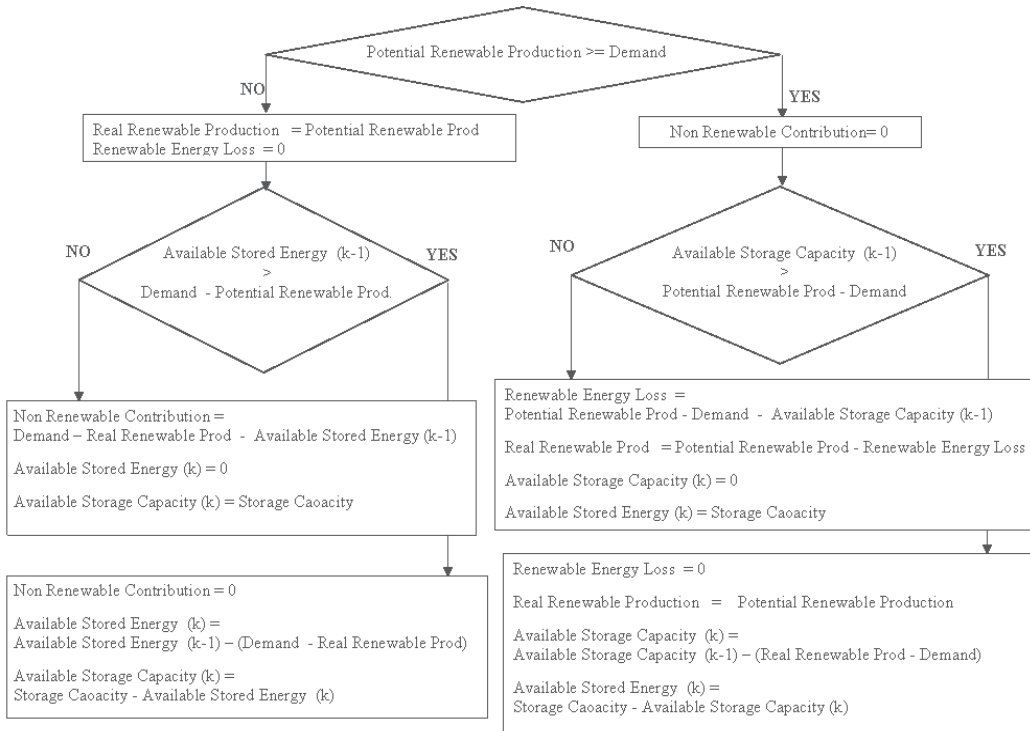
Fig. 6. Hour-by-hour energy balance algorithm.
