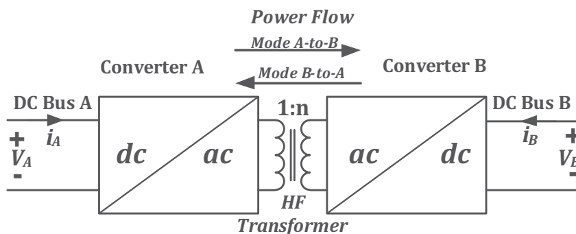
Fig. 5. Basic structure of an IBDC
