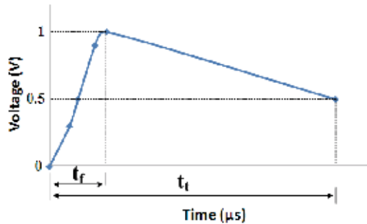
Fig. 2. Standardized impulse voltage wave shape
