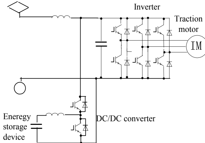
Fig. 2. Shunt connected energy storage device for DC electric rolling stock
