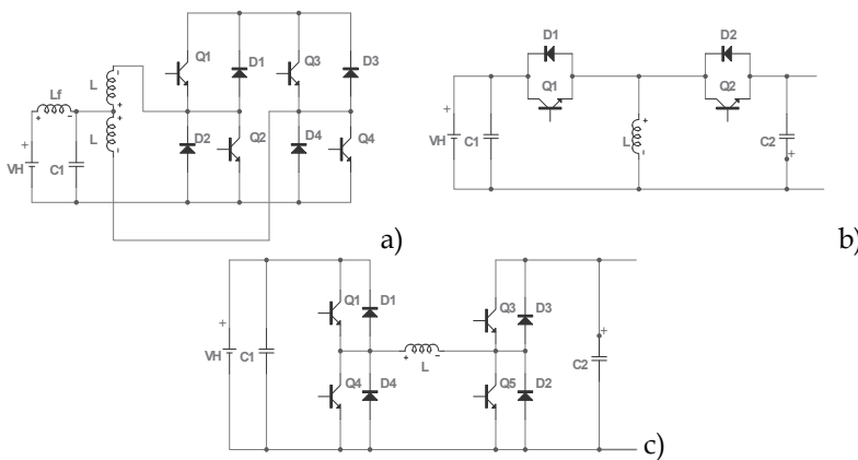
Fig. 19. Bi-directional dc-to-dc converter a) multiple legs Buck and Boost converter); b) Conventional bi-directional Buck-Boost dc-to-dc converter (delivered from Fig. 20); c) Cascade Buck-Boost converter)
