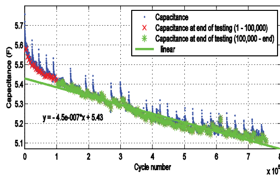
Fig. 20. Capacitance versus cycle number during cycle lifetime testing
