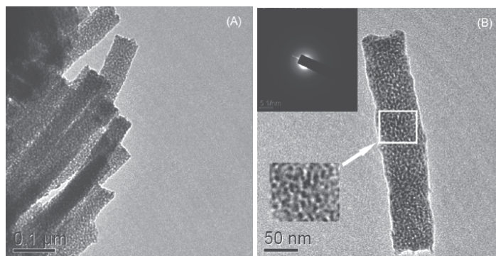
Fig. 15. TEM images of the mesoporous \text{MnO}_2 nanowires: (A) low magnification image, and (B) high magnification image. Inset is the electron diffraction pattern of nanowires in TEM.
