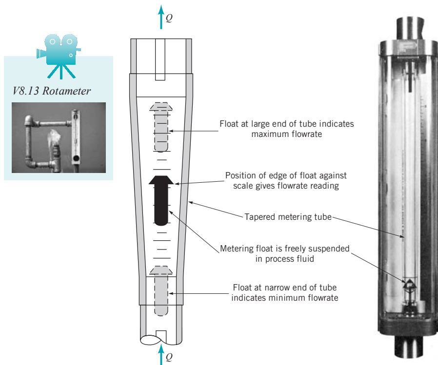
FIGURE 8.46 Rotameter-type flow meter. (Courtesy of Fischer & Porter Co.)
