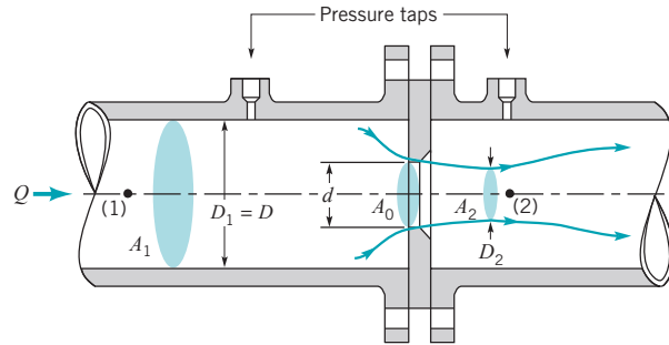
■ FIGURE 8.40 Typical orifice meter construction.
