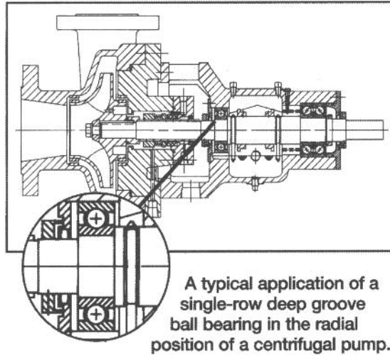
Figure 5.3: API 610 style centrifugal pump cross section with the radial bearing circled.
