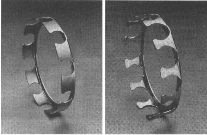
Figure 5.14: Snap-in pressed steel cages for Conrad-type bearings (left) and filling slot bearings (right).
