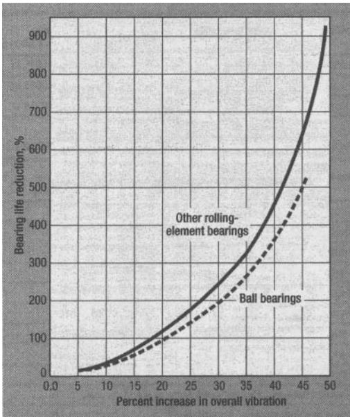
Figure 13.3: Bearing degradation shows up as vibration and can be related to life reduction.
