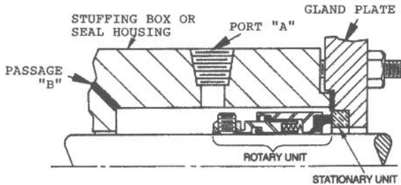
Figure 9.1: Operating principle and essential nomenclature of mechanical seals.
