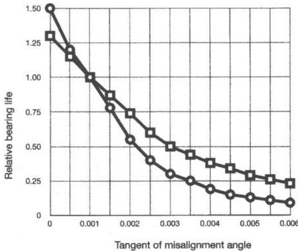
Figure 14.7: How misalignment shortens service life of typical bearings. Most bearings fit somewhere between the two curve boundaries. At tangents below 0.001, bearing life is here assumed to exceed a relative rating of 1 (Ref. 4).
