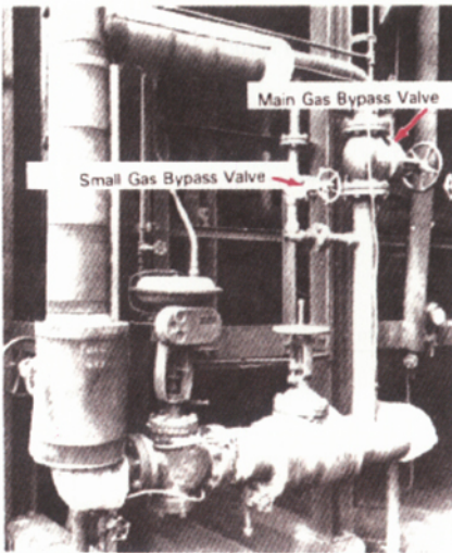
Figure 44b Gas bypass valves. The small gas valve is car-sealed (chain-locked) open during furnace operation to prevent flame-out.
