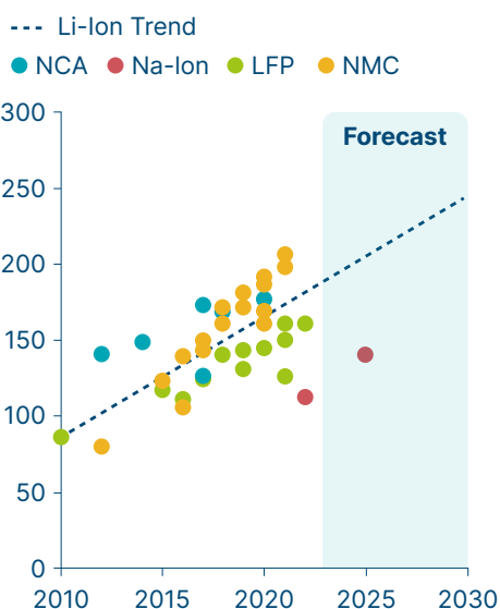
Li-ion battery pack energy density 1 Wh/kg
