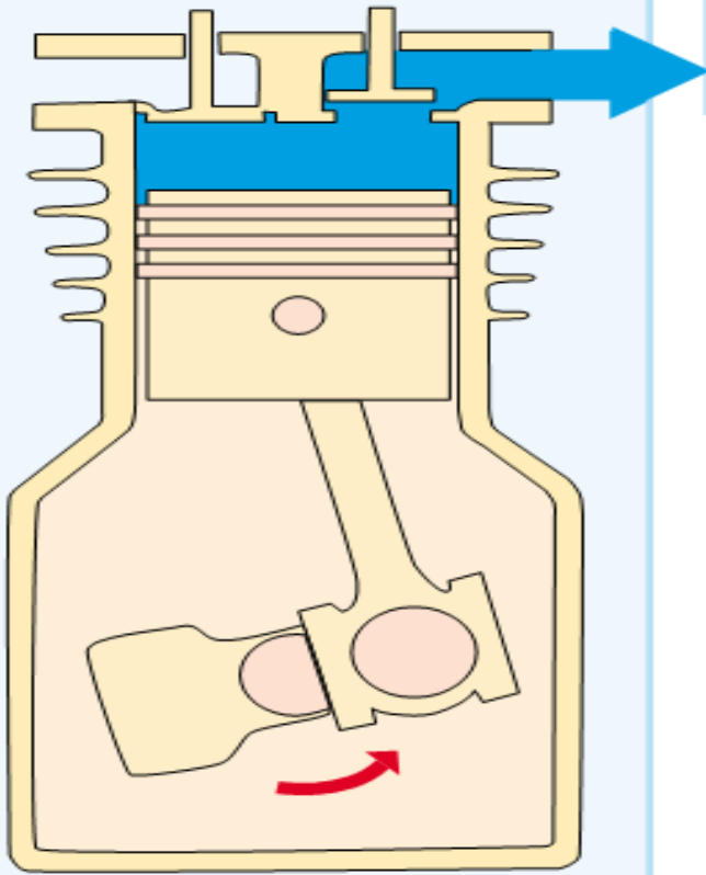
Single stage, single acting piston compressor.
