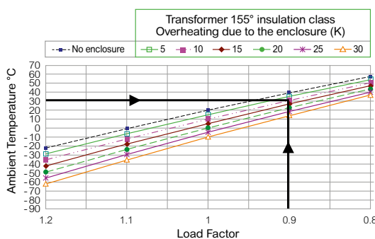
Fig E2 Dry-type transformer load factor (155°C insulation class)
