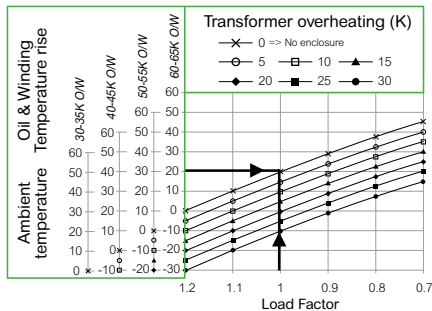
Fig E1 Liquid filled transformer load factor
