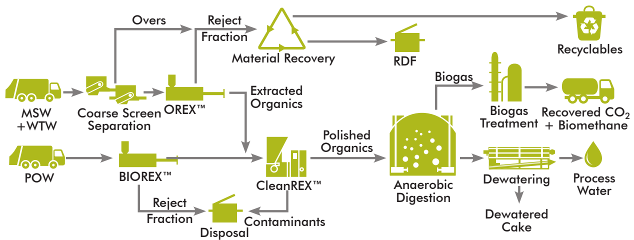
Figure 2.6: Flow diagram showing overall process of New Horizons Waste to Energy (Anaergia)
