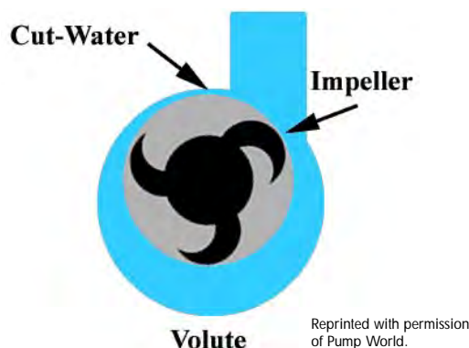
Figure 7.7.4. Centrifugal pump.
