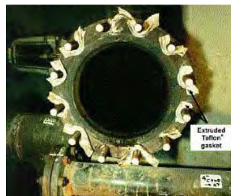
Figure 7.3.7. Failed gasket on blind flange.
