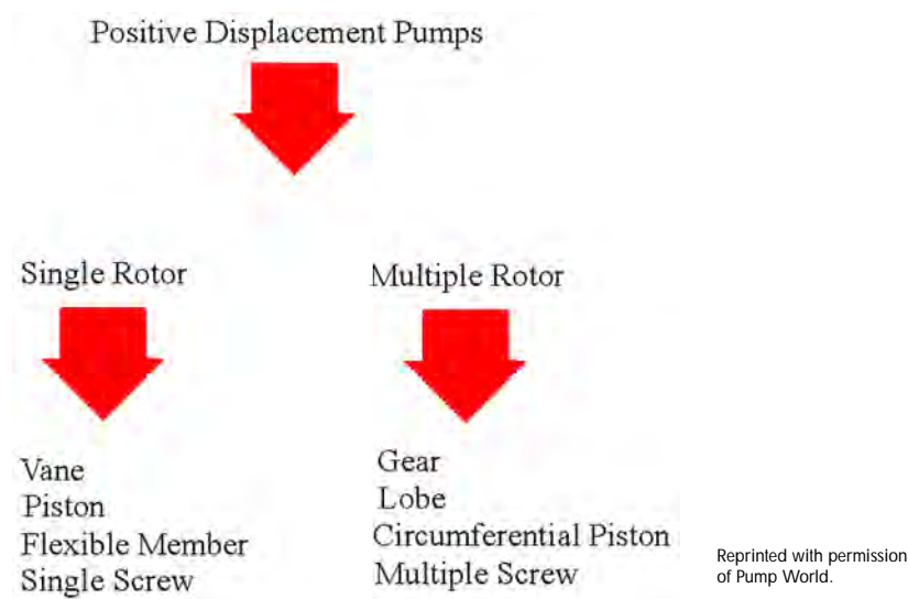
Figure 7.7.3. Positive displacement pumps.
