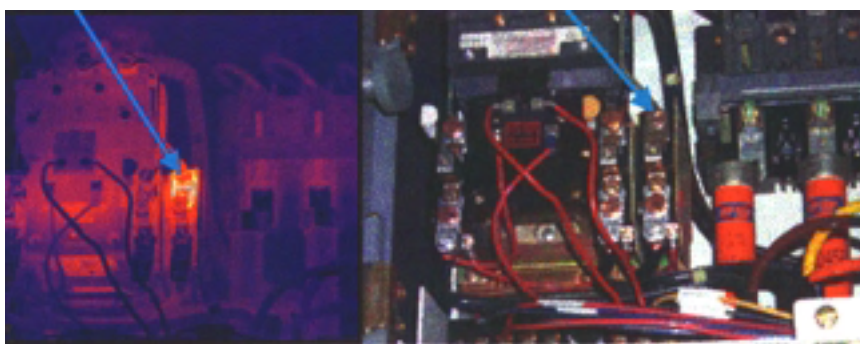
Figure 6.2.5. Overload connection problem. Note difference in IR image coloration between overload contacts.
