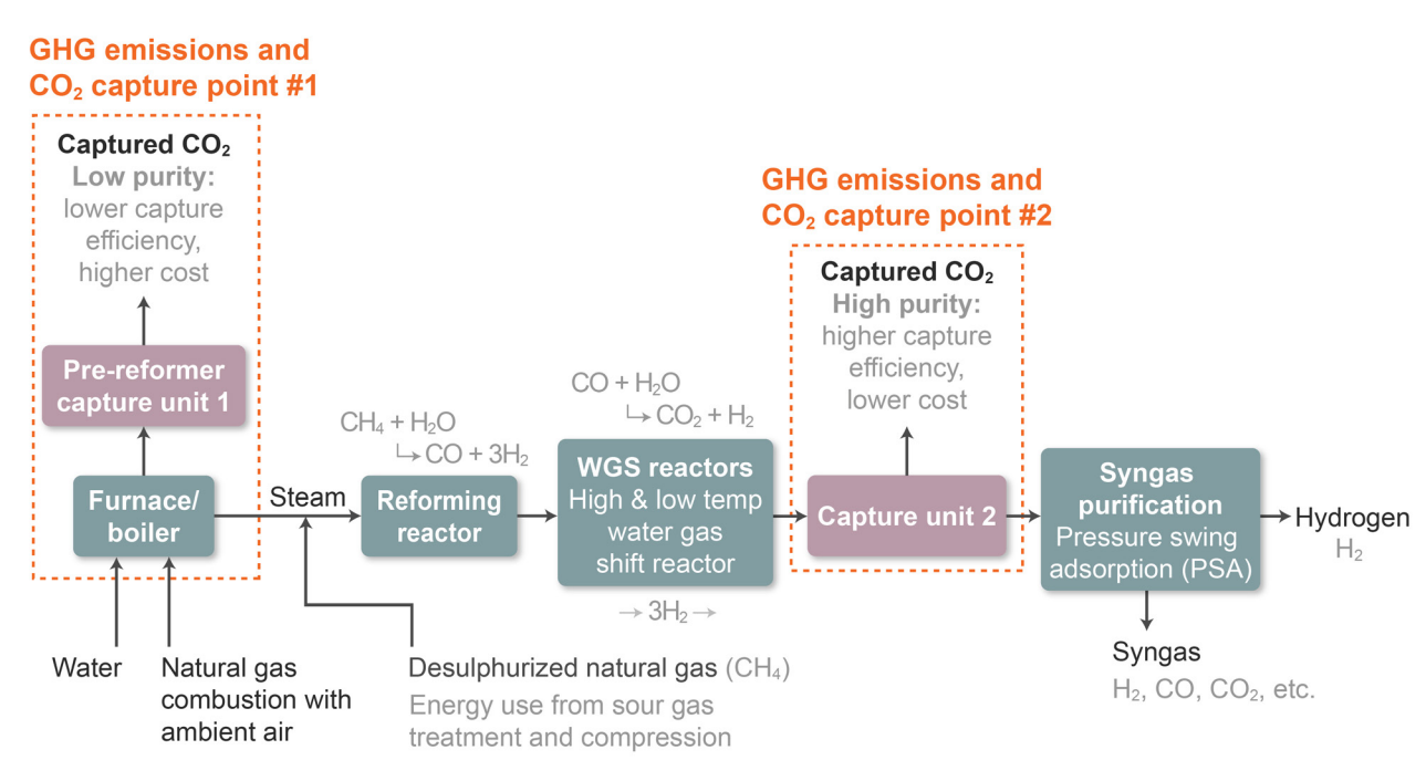
Process diagram: SMR with carbon capture
