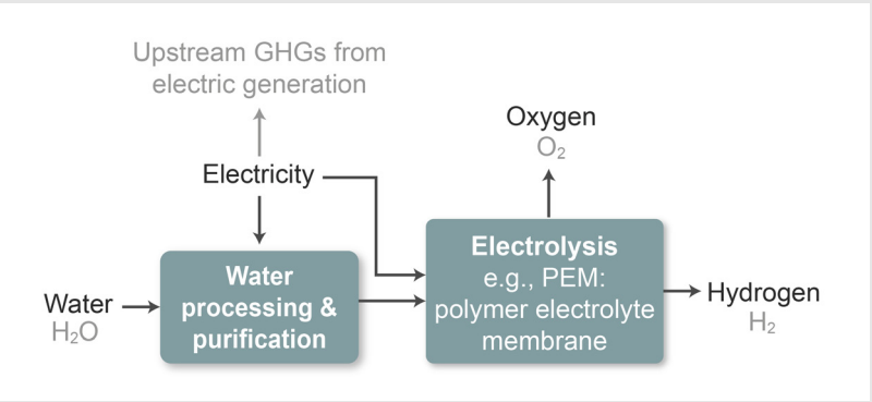
Process diagram: Hydrogen electrolysis
