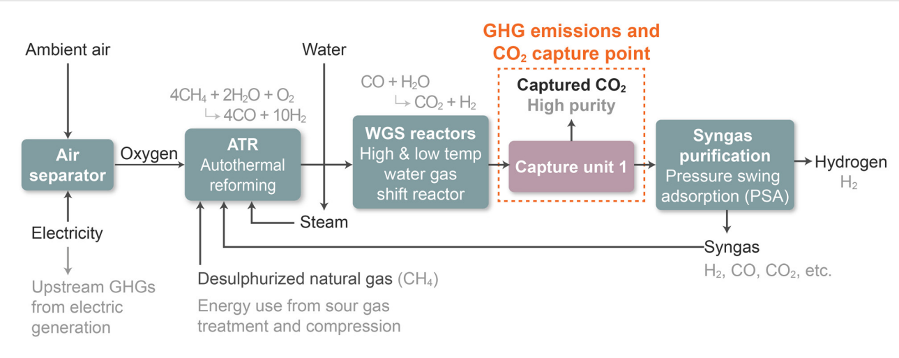
Process diagram: ATR with carbon capture
