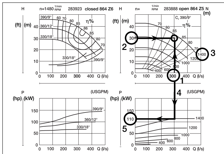
Figure 6. An example of pump curves. Left: Pump with three different impeller diameters. Right: Pump with six different speeds.
