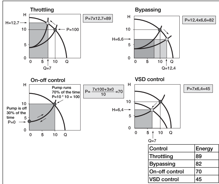
Figure 4. The power consumption of the four most common flow control methods for centrifugal pumps.
