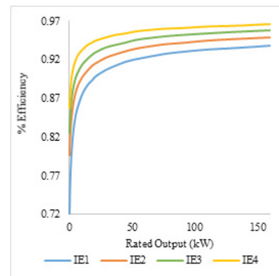
Figure 8 Illustrates the IE3 to IE4 efficiency bands for 4 pole motors, as defined in the IEC standard.
