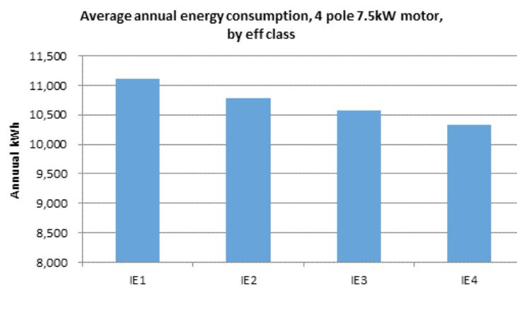
Figure 9 Broad comparison of motor efficiency
