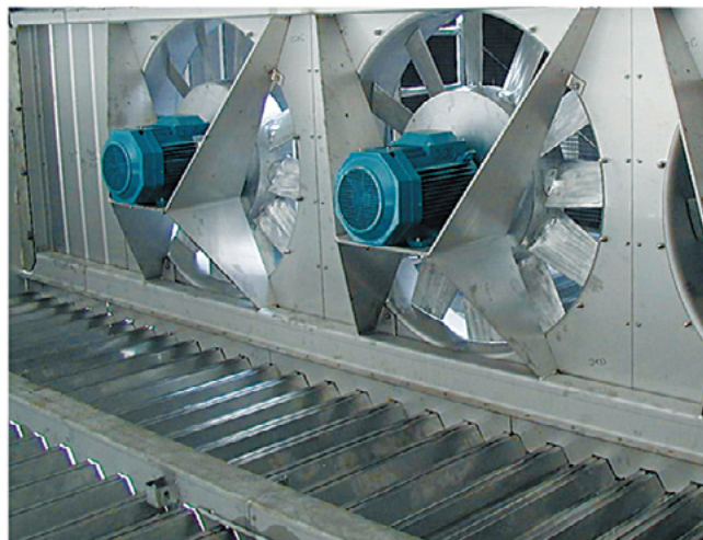
"Motors with axial fans in ventilation system" Supplied courtesy of Siemens
