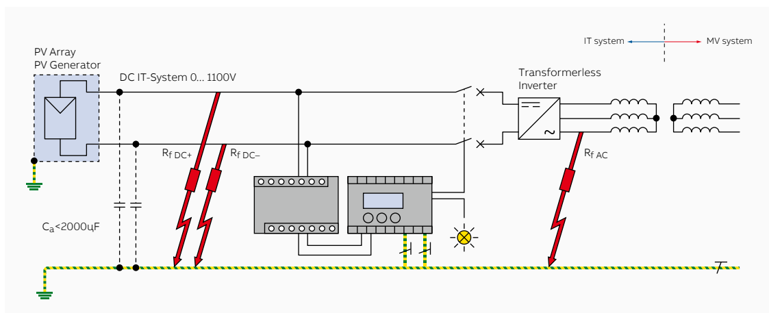
Figure 66 insulation surveillance controller
