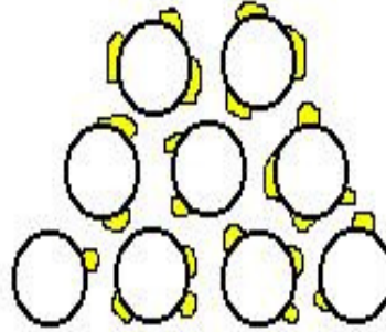
Physical Adsorption
