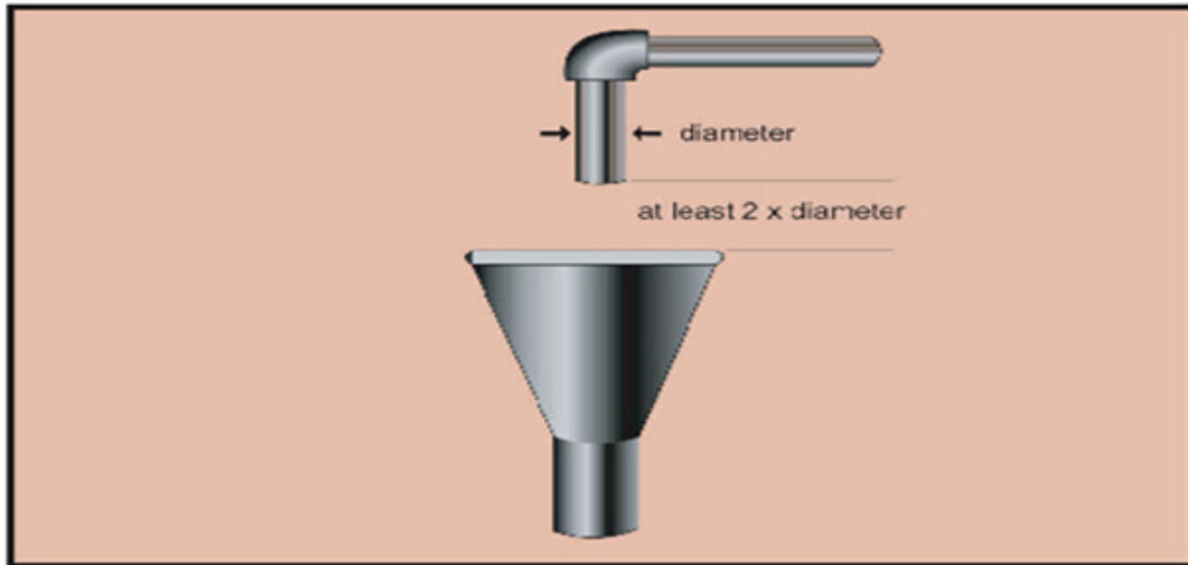
8.4.1 Figure 1: Air gap
