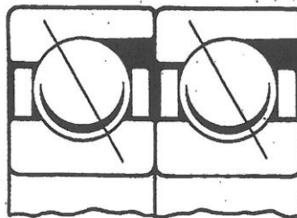
Tandem Mounting
