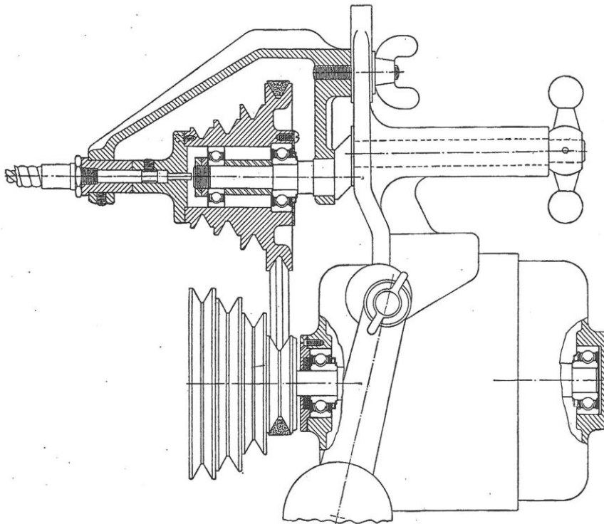
Flexible Shaft Drive Unit
