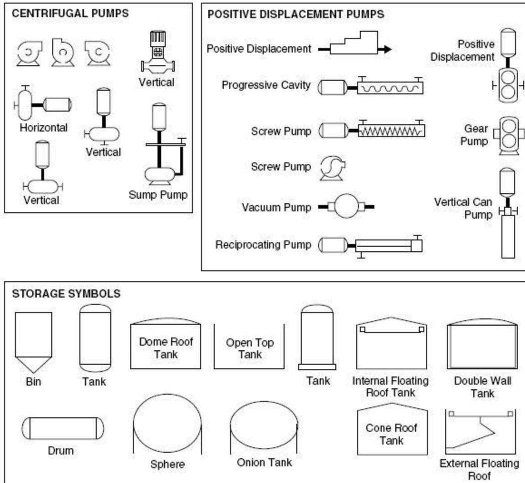
Pumps and Tanks
