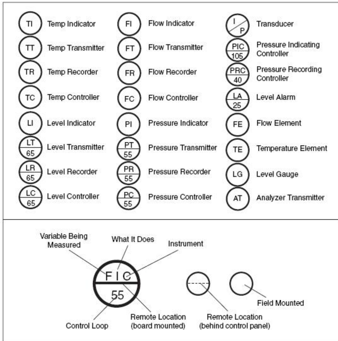
Process and Instrument Symbols
