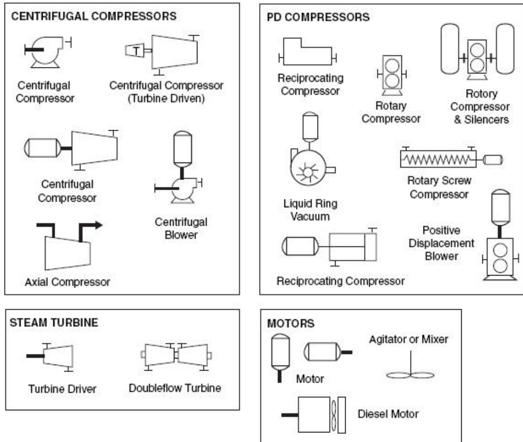
Compressors, Steam Turbines, and Motors
