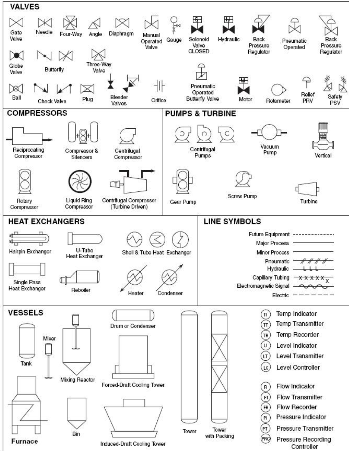
Process and Instrument Symbols
