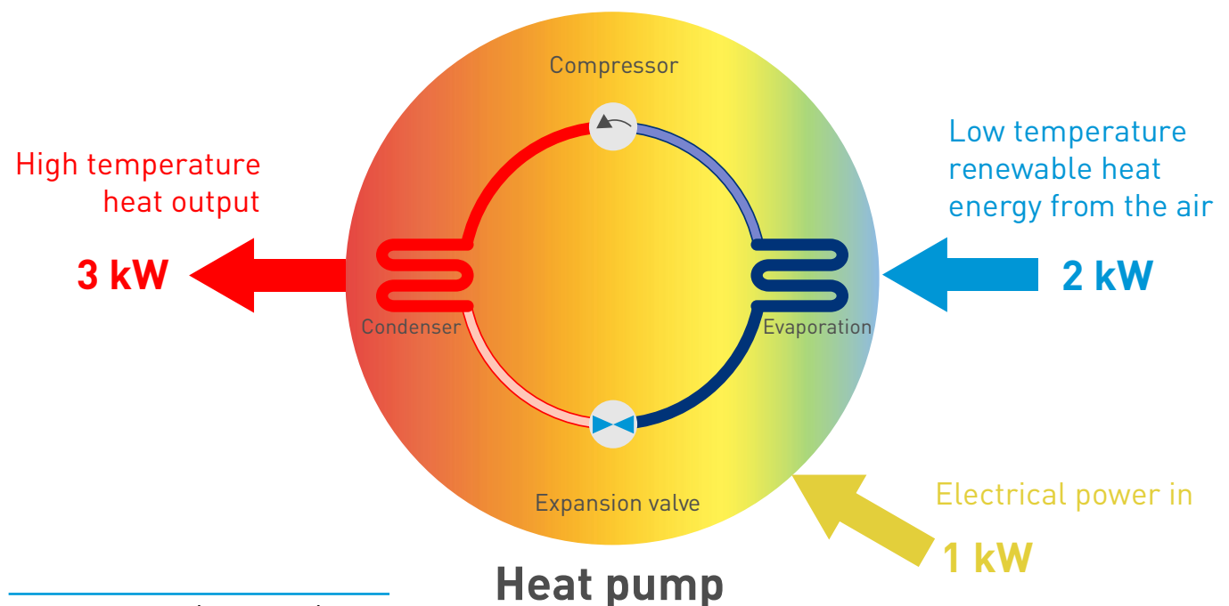
Figure 1: Air-source heat pump diagram
