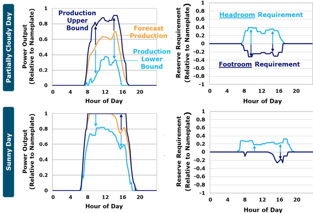
Figure 2: Confidence in solar forecasts hours ahead of real-time (left) and resulting forecast error reserve levels (right) on an example partly cloudy day (top) and sunny day (bottom), normalized to solar power plant capacity. As discussed below, reserve requirements must be met by non-solar resources if solar flexibility is not integrated into system operator dispatch procedures, but can be partially met by solar power plants when solar is represented as more flexible.
