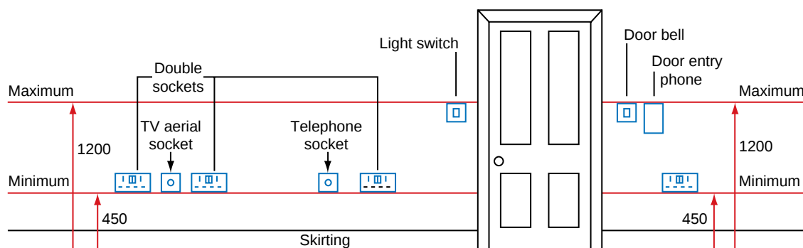
Figure 4.10 Fixing positions of switches and socket outlets.
