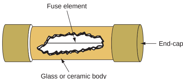
Figure 3.33 Cartridge fuse.
