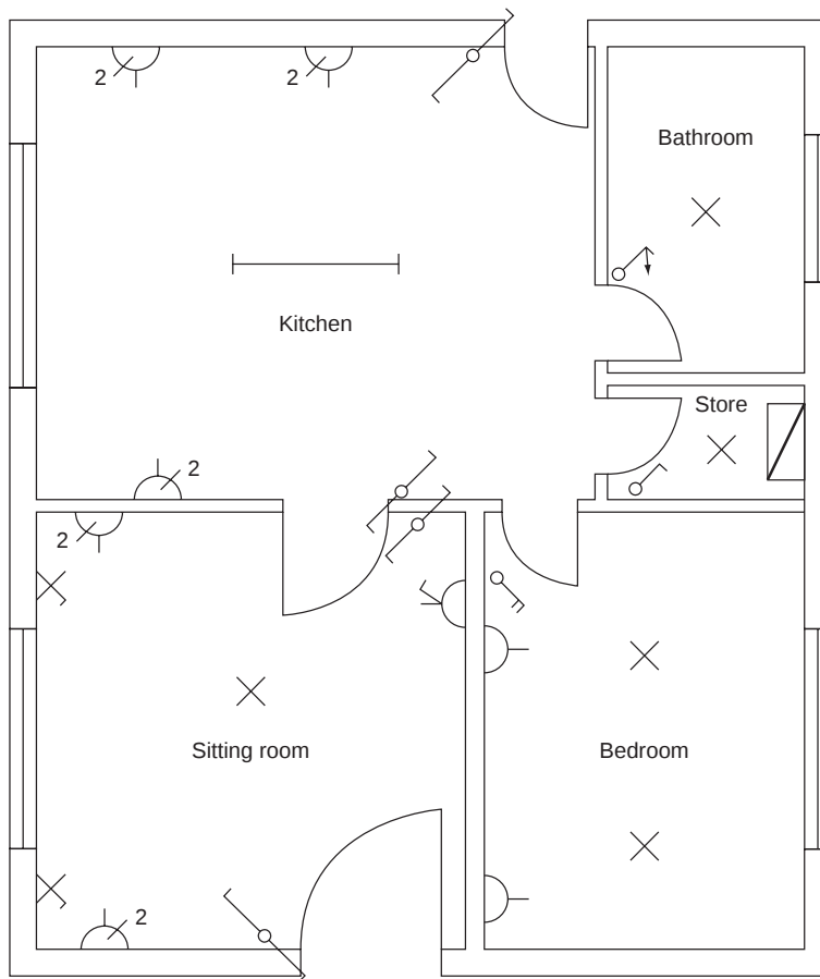
Figure 1.13 Layout drawing or site plan of a small electrical installation.
