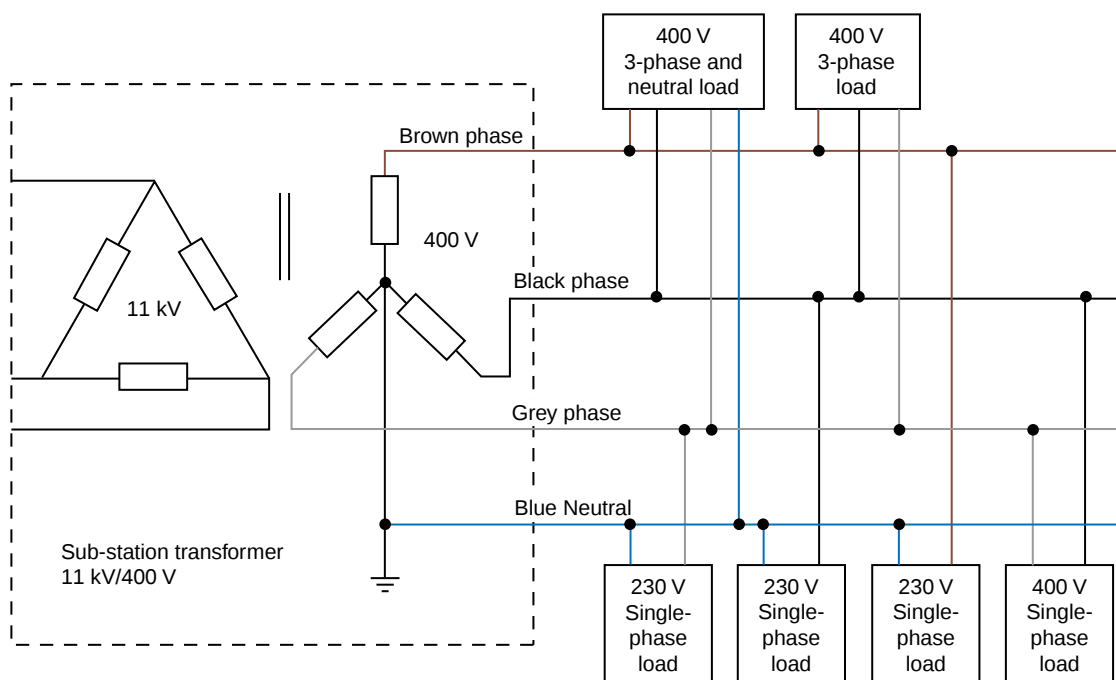
Figure 3.30 Three phase four wire distribution.
