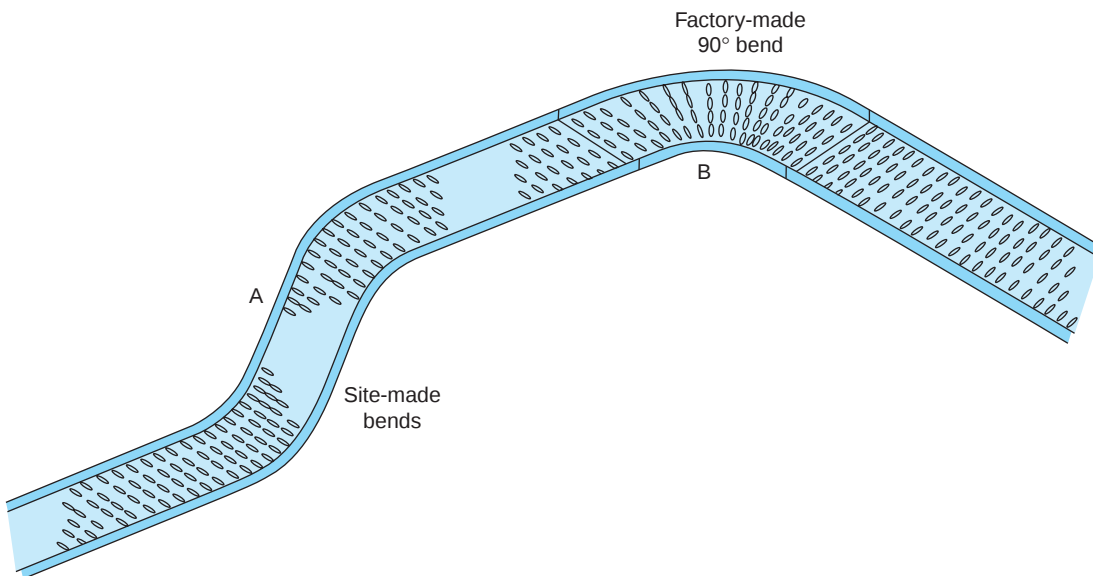
Figure 4.19 Cable tray with bends.
