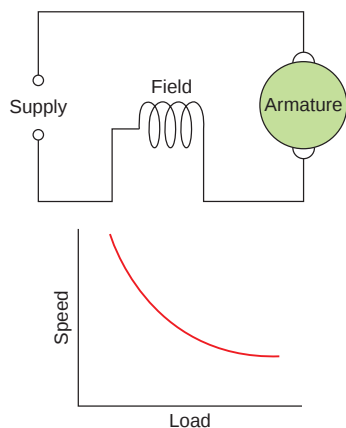
Figure 3.22 Series motor connections and characteristics.
